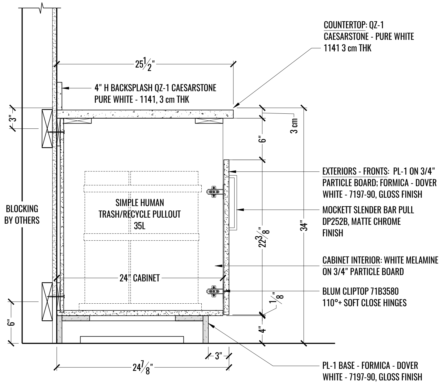
1 SECTION: LOUNGE RM# 1804 - TRASH/RECYCLE PULLOUT A SCALE: 1-1/2" = 1'-0"
