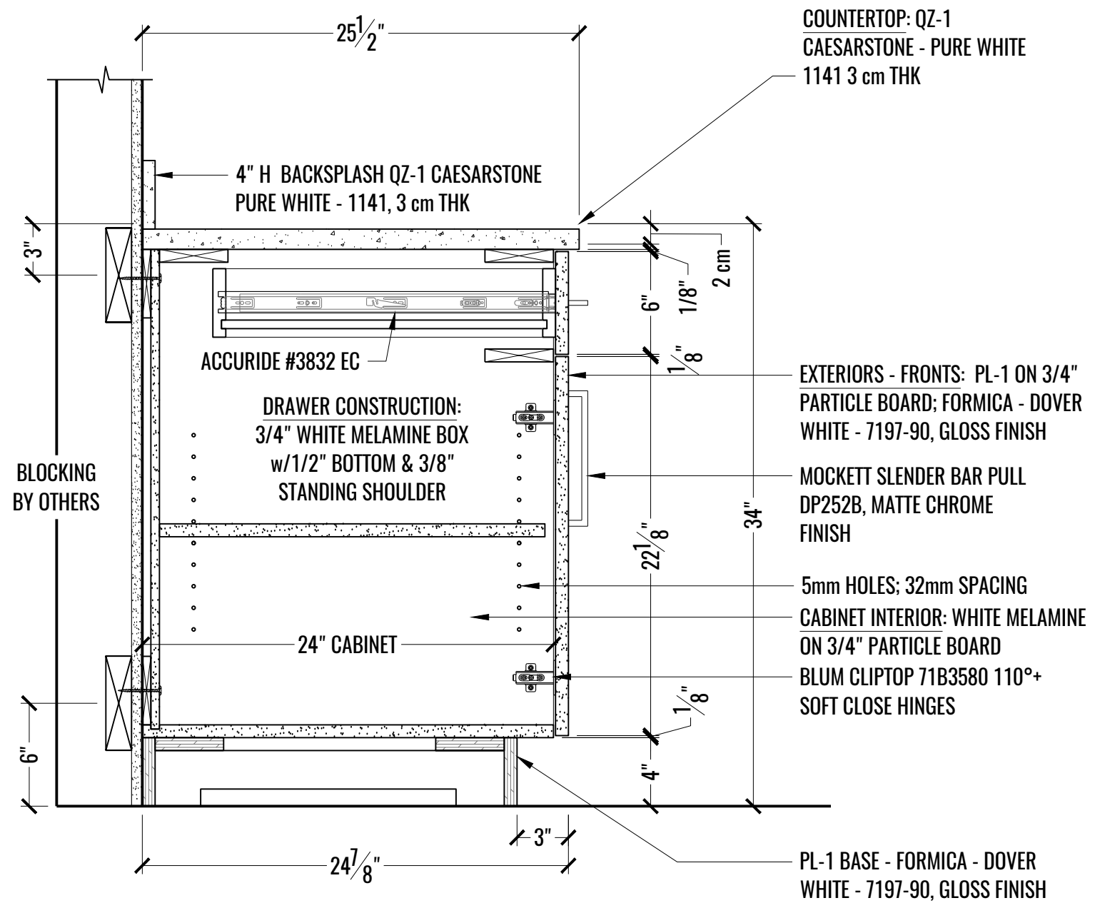
2 SECTION: LOUNGE RM# 1804 - BASE CABINET W/DRAWER A SCALE: 1-1/2" = 1'-0"
