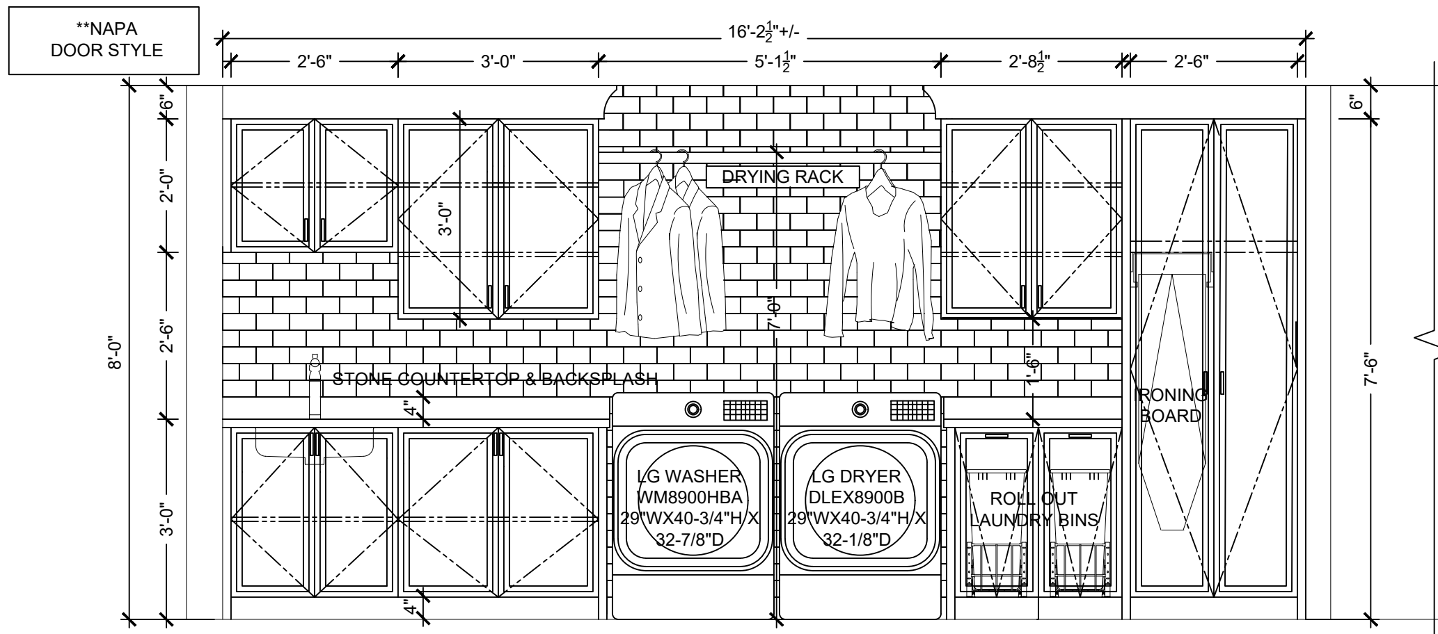
LAUNDRY ROOM ELEVATION - OPTION 2
