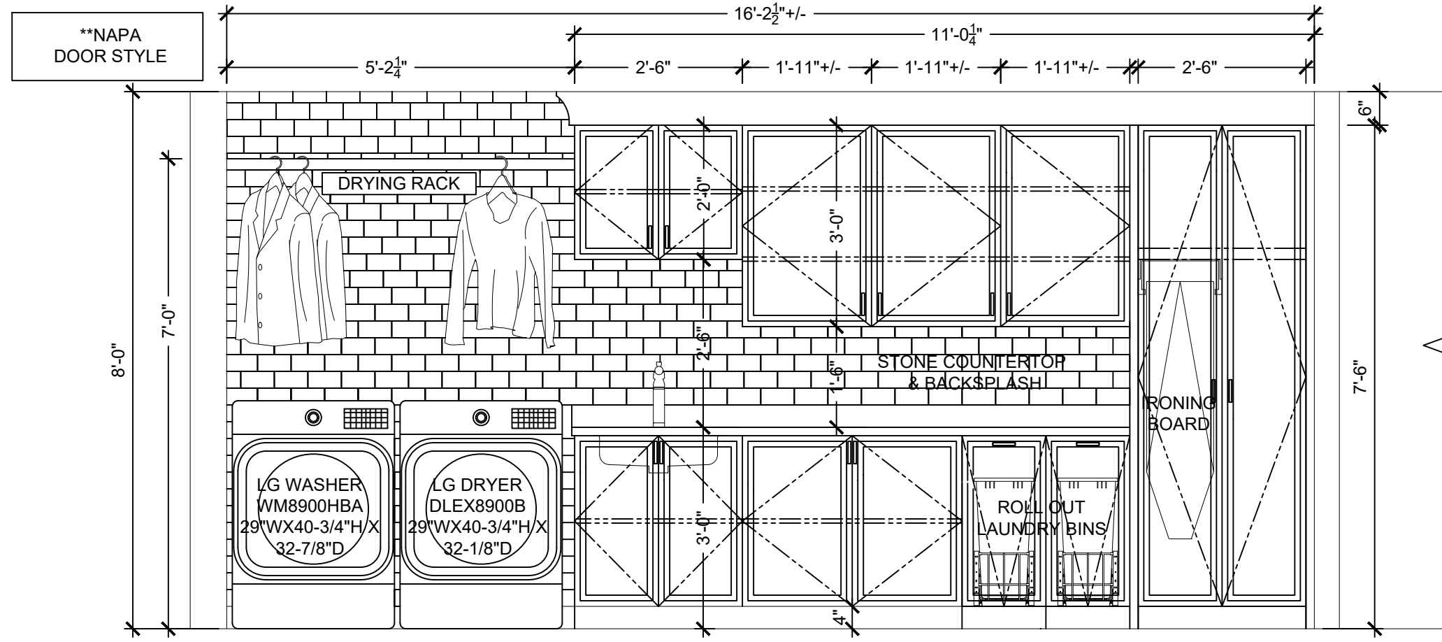
LAUNDRY ROOM ELEVATION - OPTION 4
