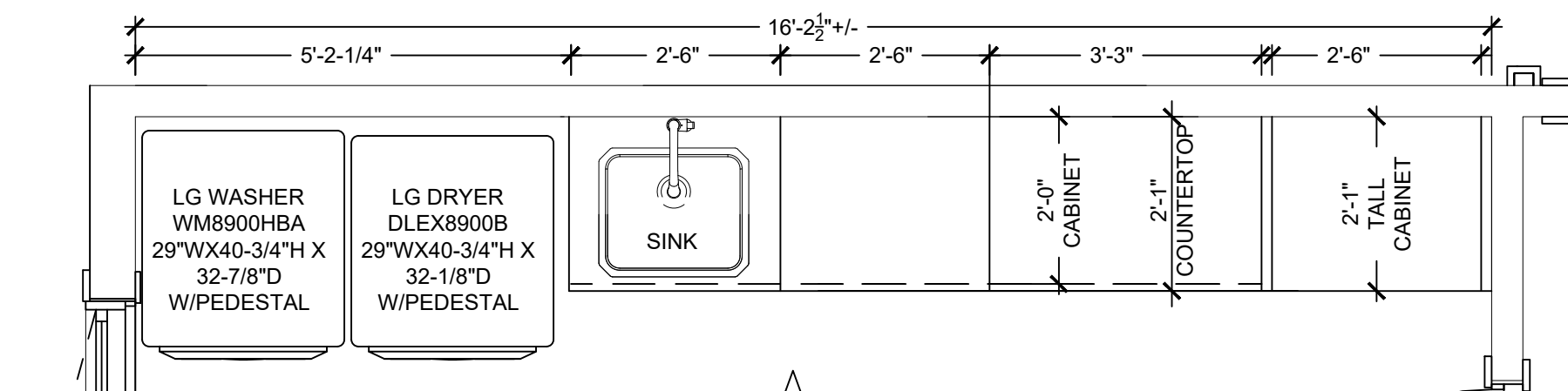
LAUNDRY ROOM PLAN - OPTION 3
