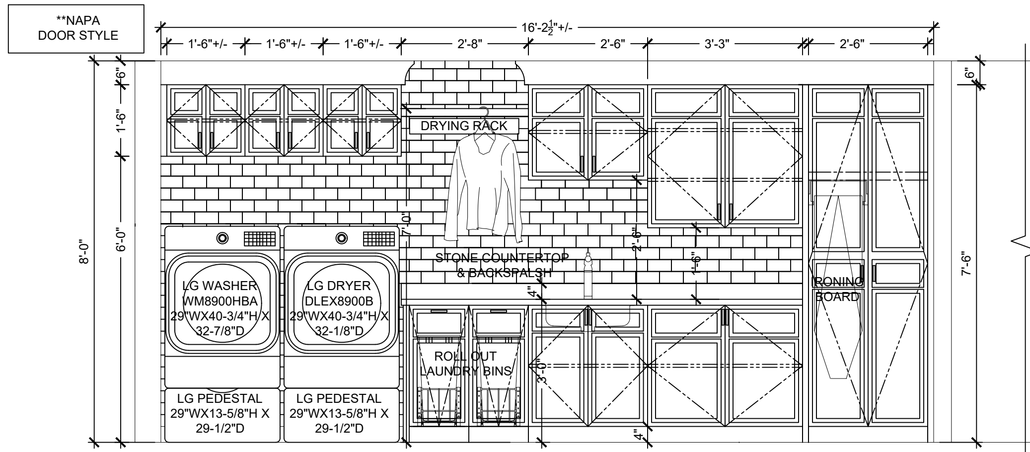
LAUNDRY ROOM ELEVATION - OPTION 4.1
