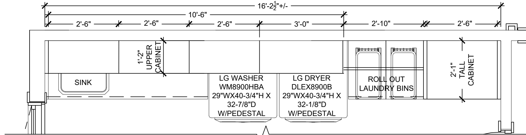
LAUNDRY ROOM PLAN (UPPERS) - OPTION 2.1
