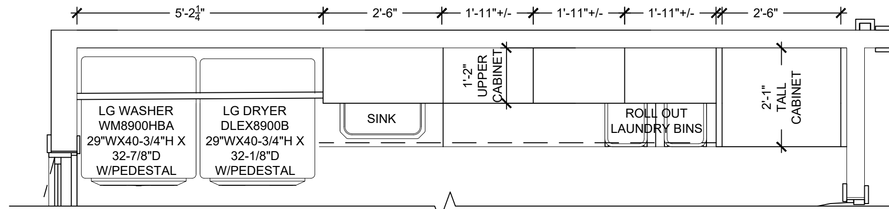
LAUNDRY ROOM PLAN (UPPERS) - OPTION 4
