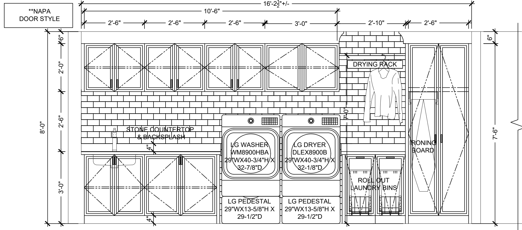
LAUNDRY ROOM ELEVATION - OPTION 2.1
