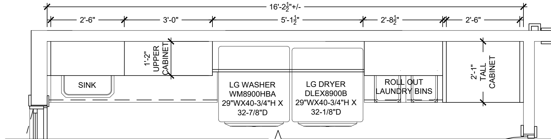
LAUNDRY ROOM PLAN (UPPERS) - OPTION 2
