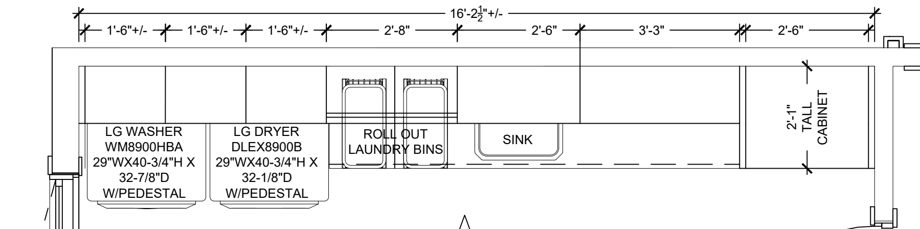
LAUNDRY ROOM PLAN (UPPERS) - OPTION 4.1
