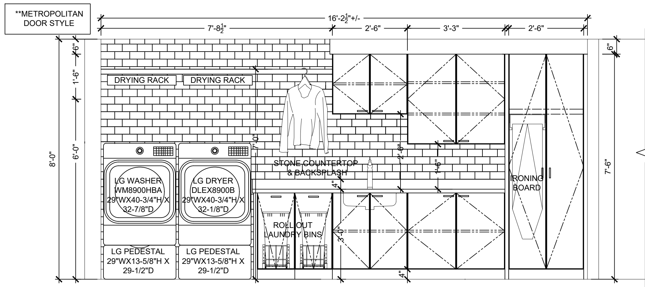
LAUNDRY ROOM ELEVATION - OPTION 3.1
