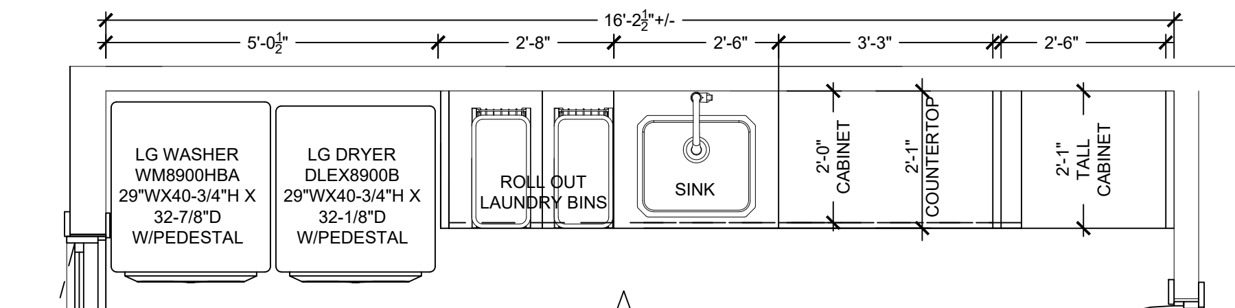
LAUNDRY ROOM PLAN - OPTION 4.1
