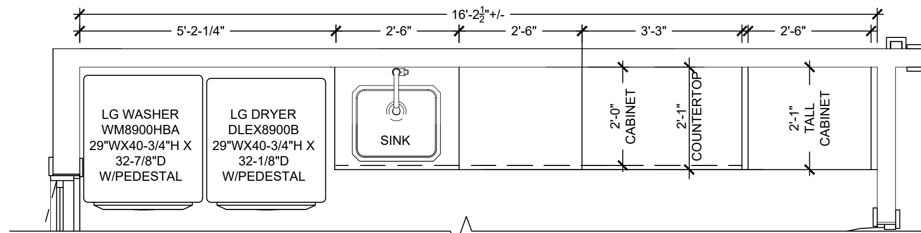
LAUNDRY ROOM PLAN - OPTION 4
