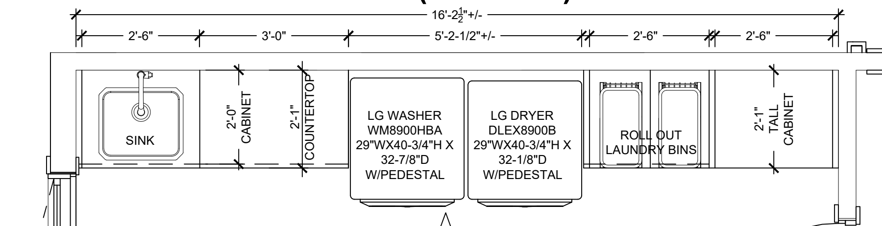
LAUNDRY ROOM PLAN - OPTION 1.1
