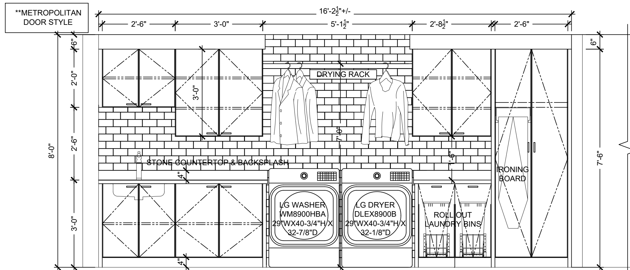
LAUNDRY ROOM ELEVATION - OPTION 1
