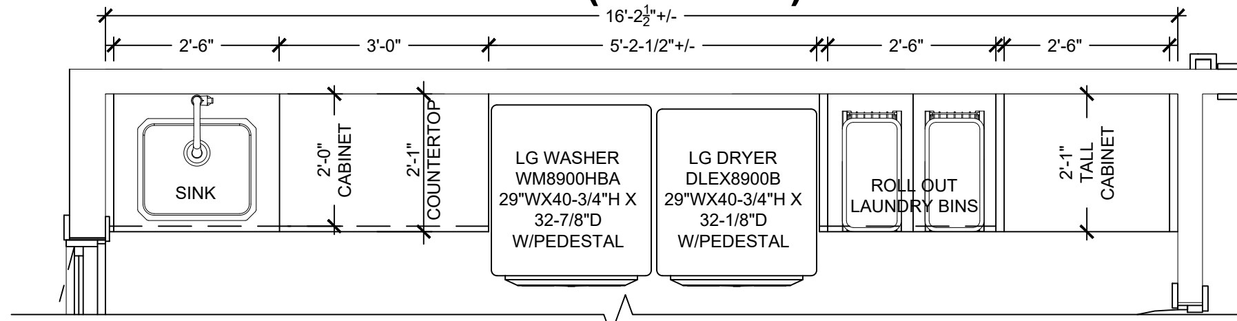
LAUNDRY ROOM PLAN - OPTION 2.1
