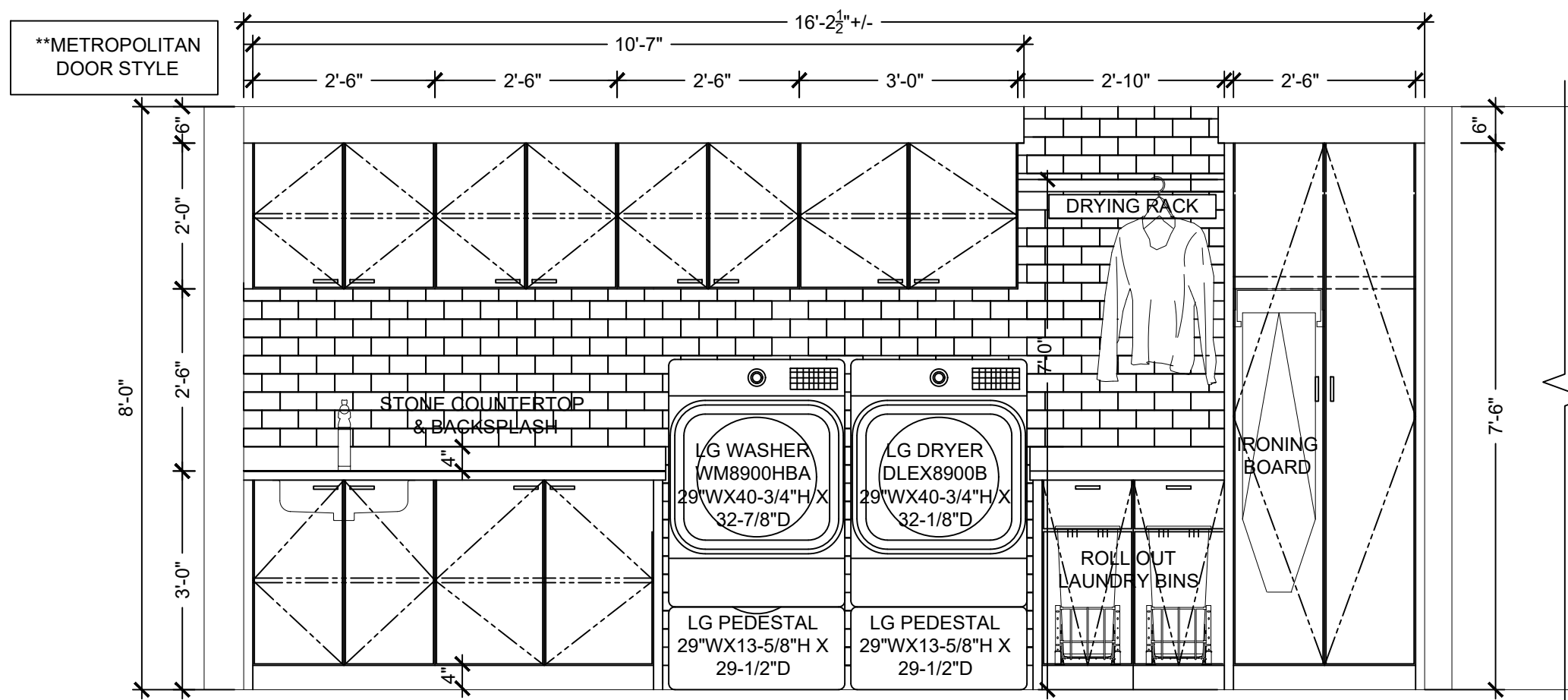
LAUNDRY ROOM ELEVATION - OPTION 1.1
