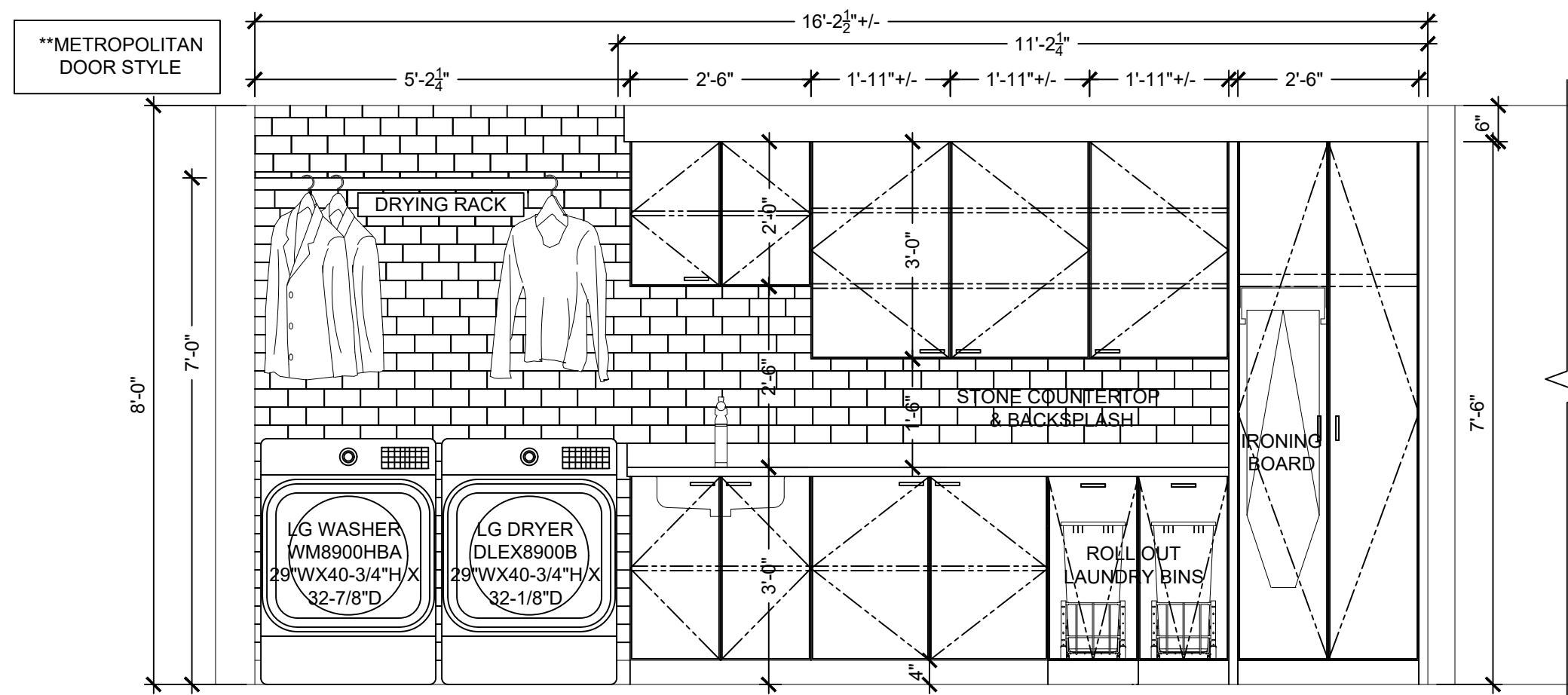
LAUNDRY ROOM ELEVATION - OPTION 3
