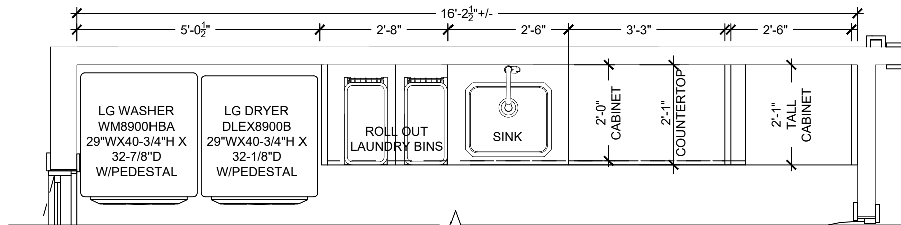
LAUNDRY ROOM PLAN - OPTION 3.1
