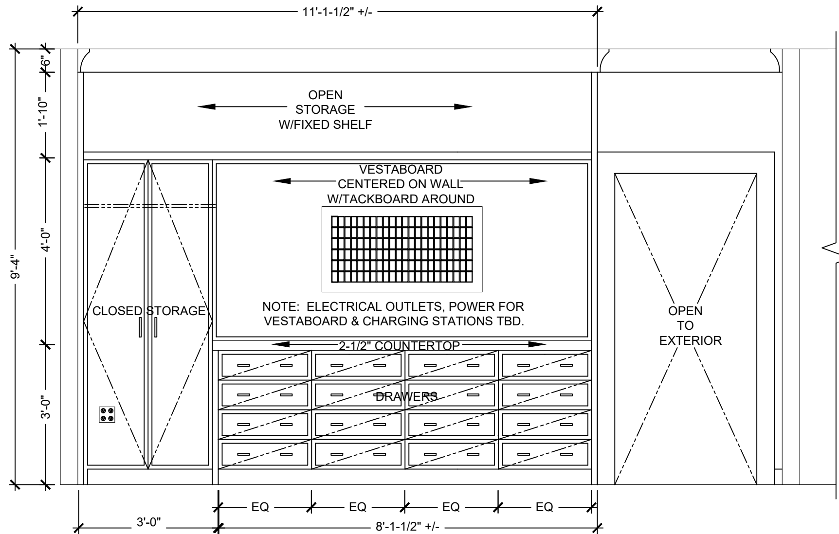
MUD ROOM ELEVATION @ ENTRY - OPTION ONE
