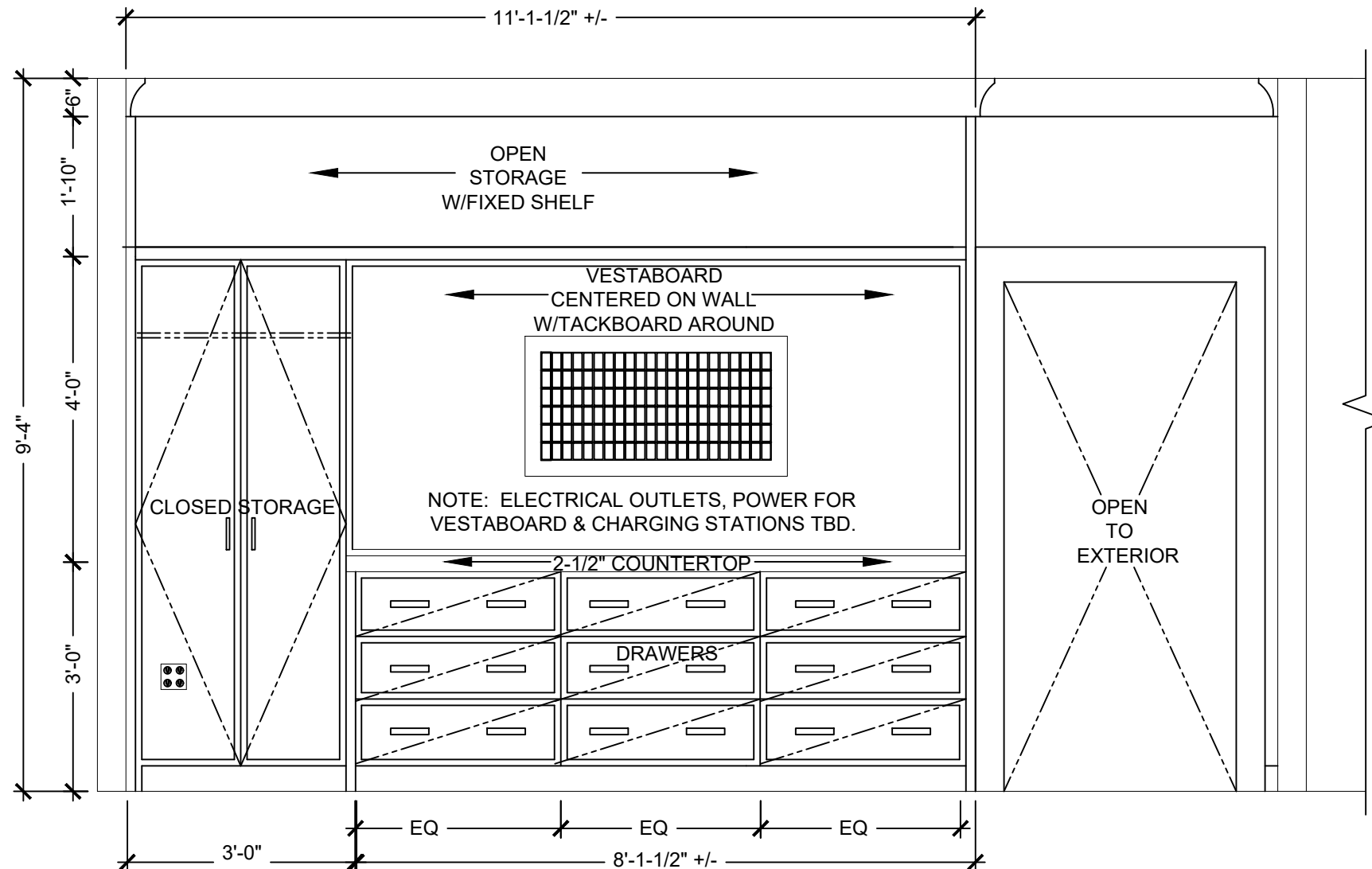
MUD ROOM ELEVATION @ ENTRY - OPTION TWO
