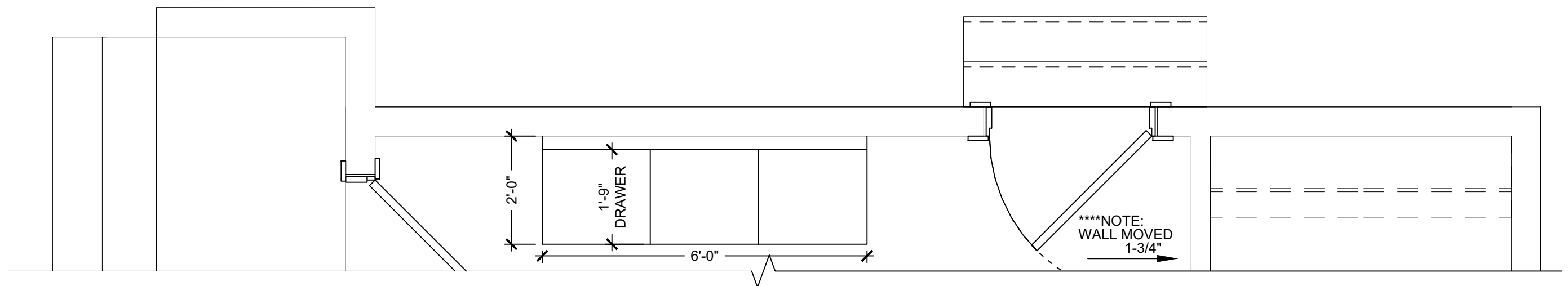
MUD ROOM PLAN @ ENTRY - OPT 2 / REV 3
