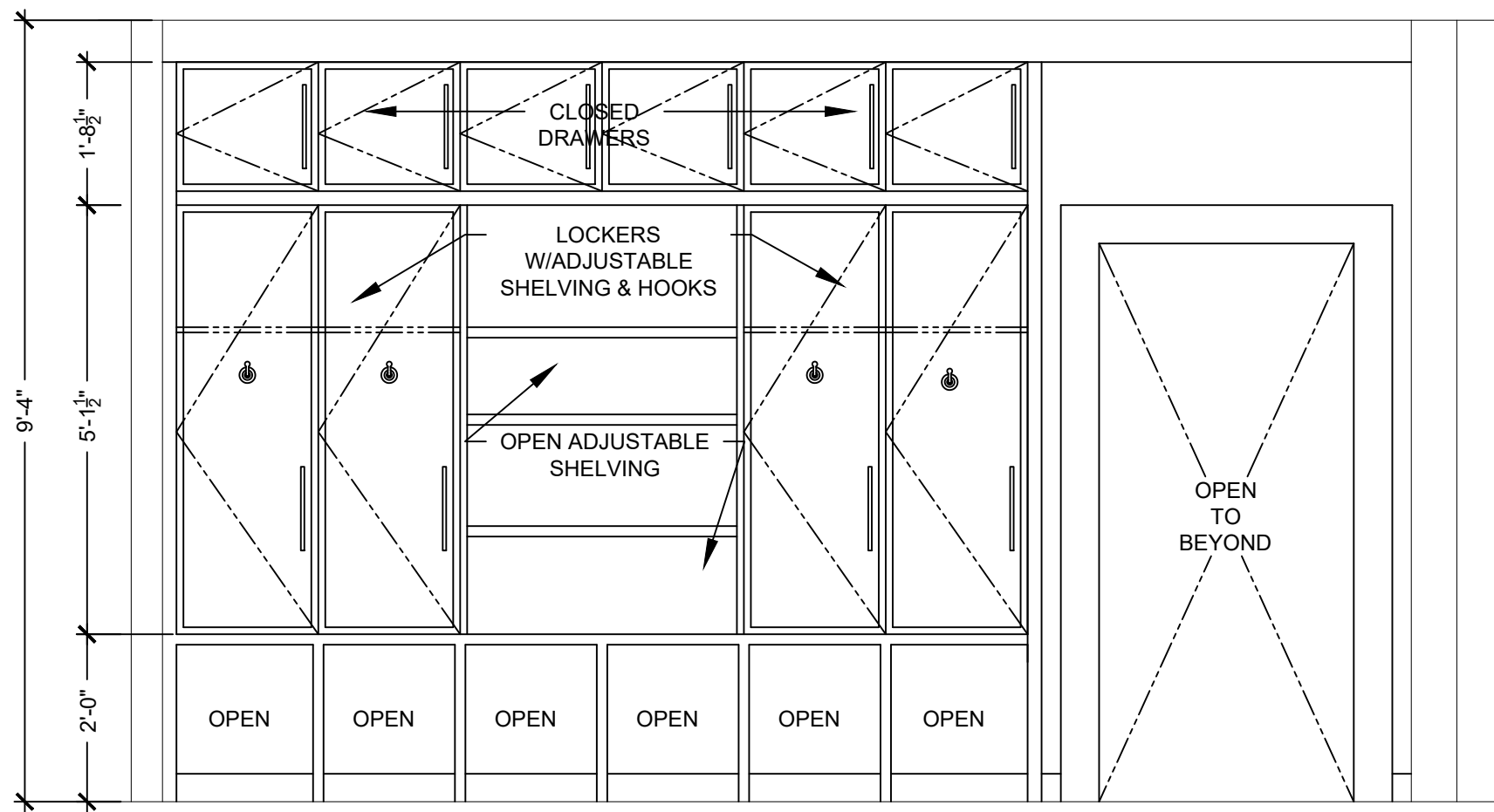
MUD ROOM ELEVATION - OPTION TWO
