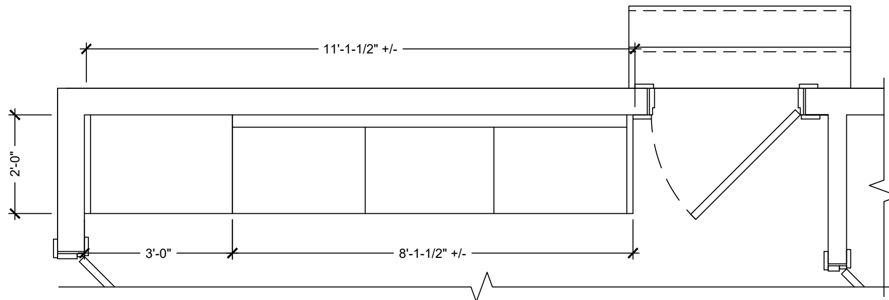
MUD ROOM PLAN @ ENTRY - OPTION TWO
