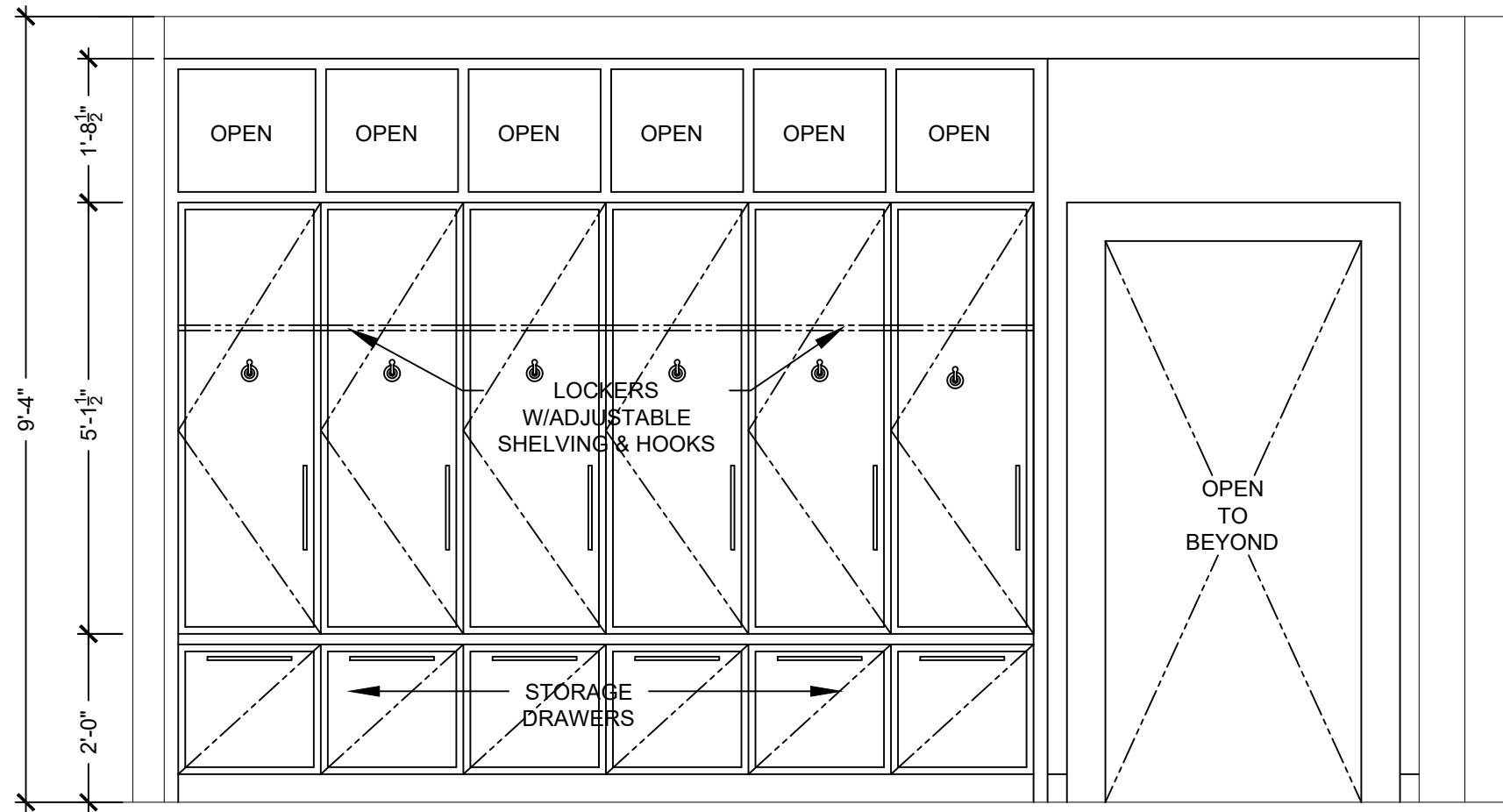
MUD ROOM ELEVATION - OPTION ONE
