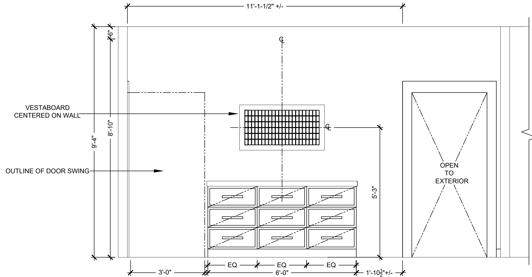
MUD ROOM ELEVATION @ ENTRY - OPT 2 / REV 3
