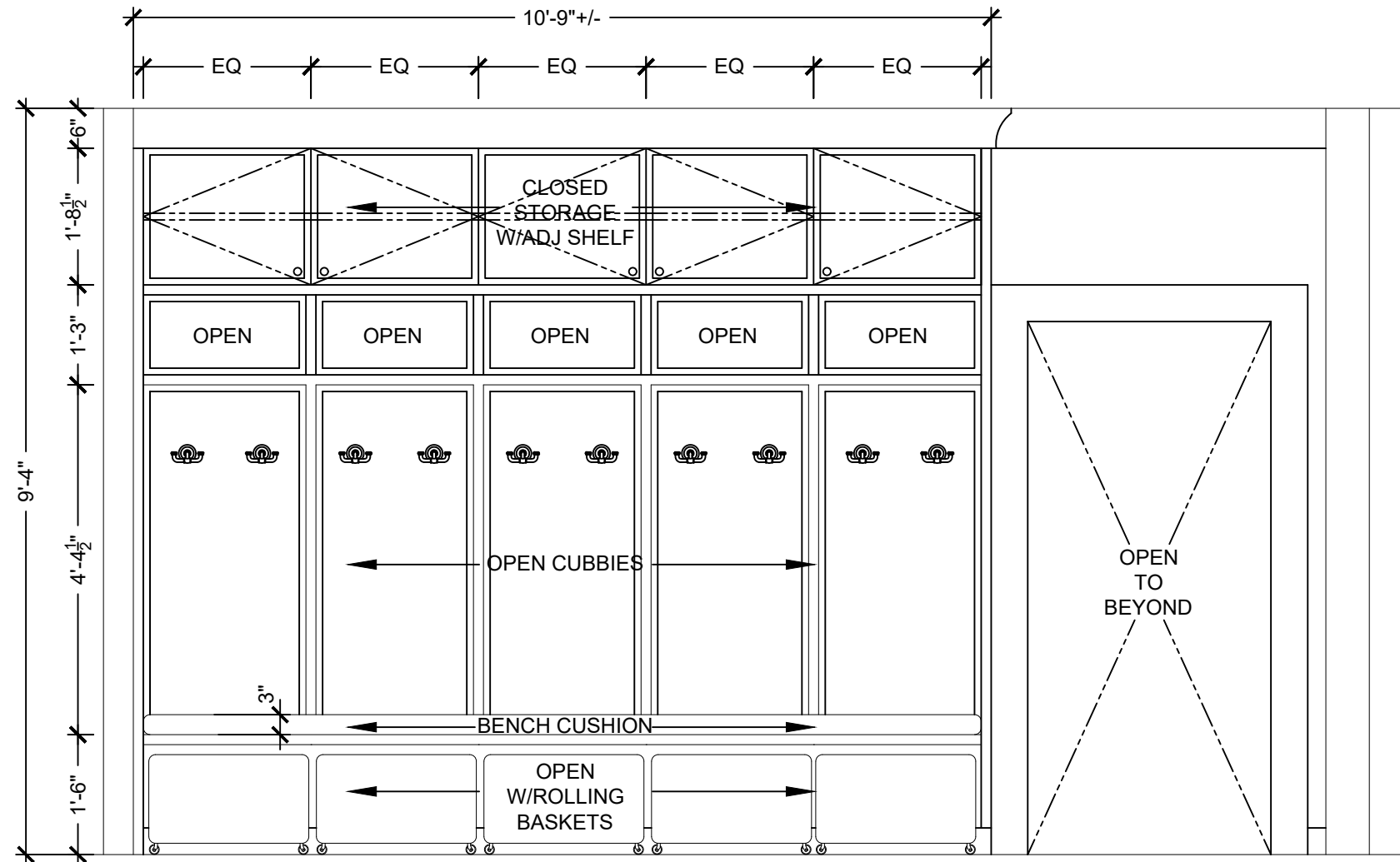
MUD ROOM ELEVATION - OPTION THREE
