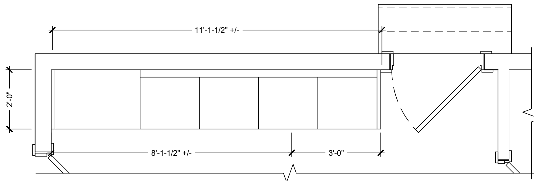
MUD ROOM PLAN @ ENTRY - OPTION ONE
