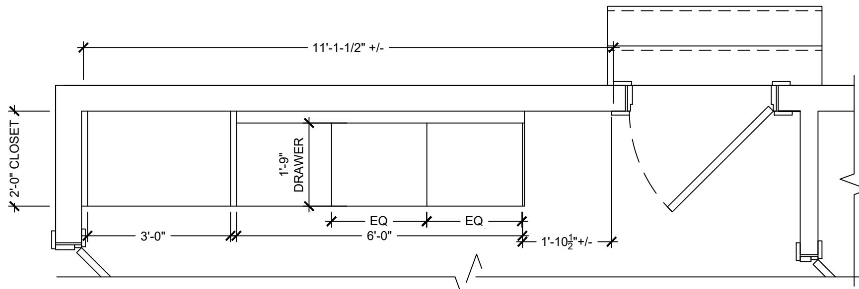
MUD ROOM PLAN @ ENTRY - REV 2 / OPT 2
