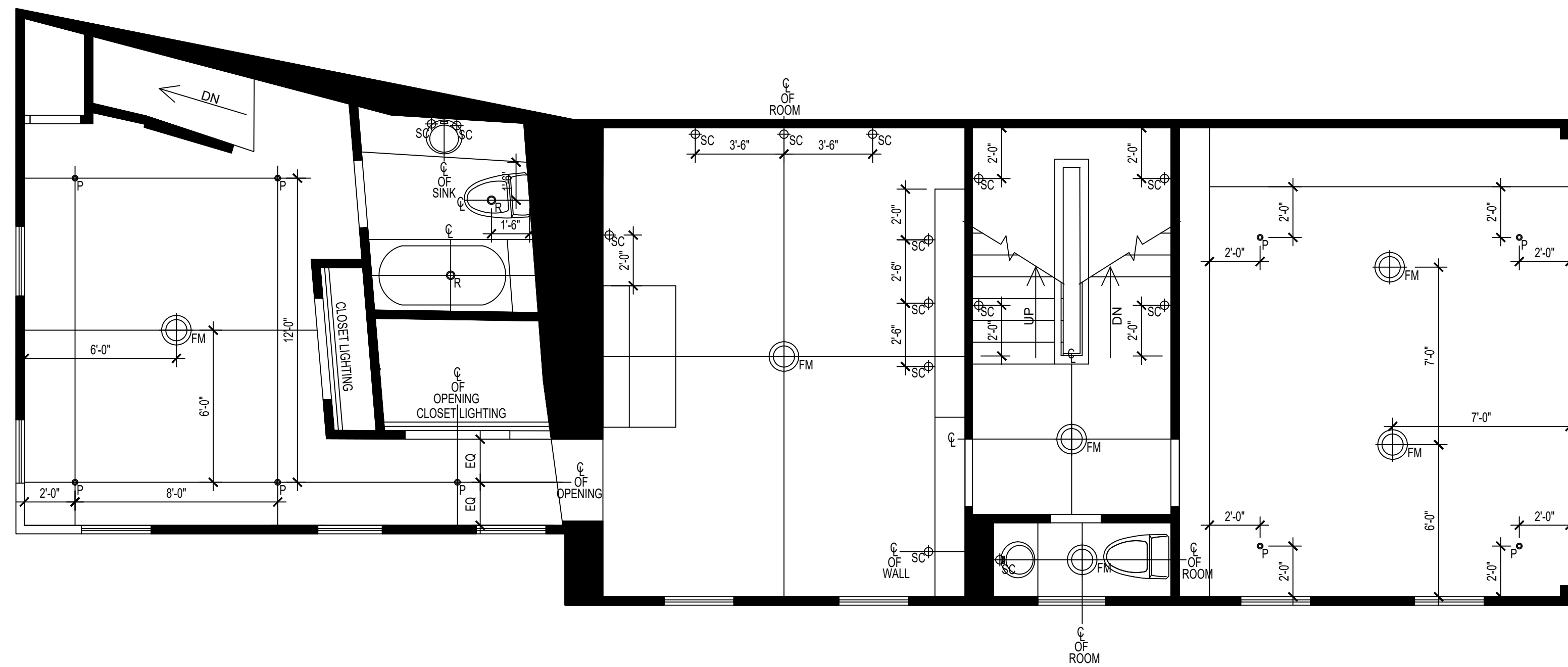
2 SECOND FLOOR REFLECTED CEILING PLAN SCALE = 1/4"=1'-0"
