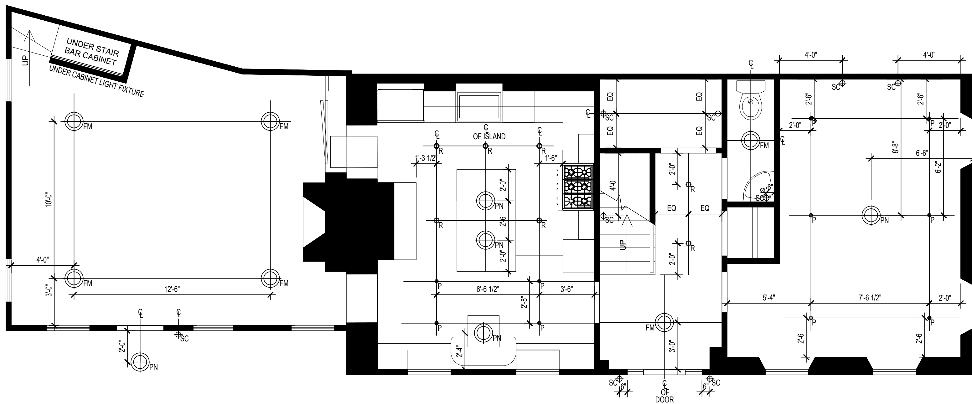
1 FIRST FLOOR REFLECTED CEILING PLAN SCALE = 1/4"=1'-0"
