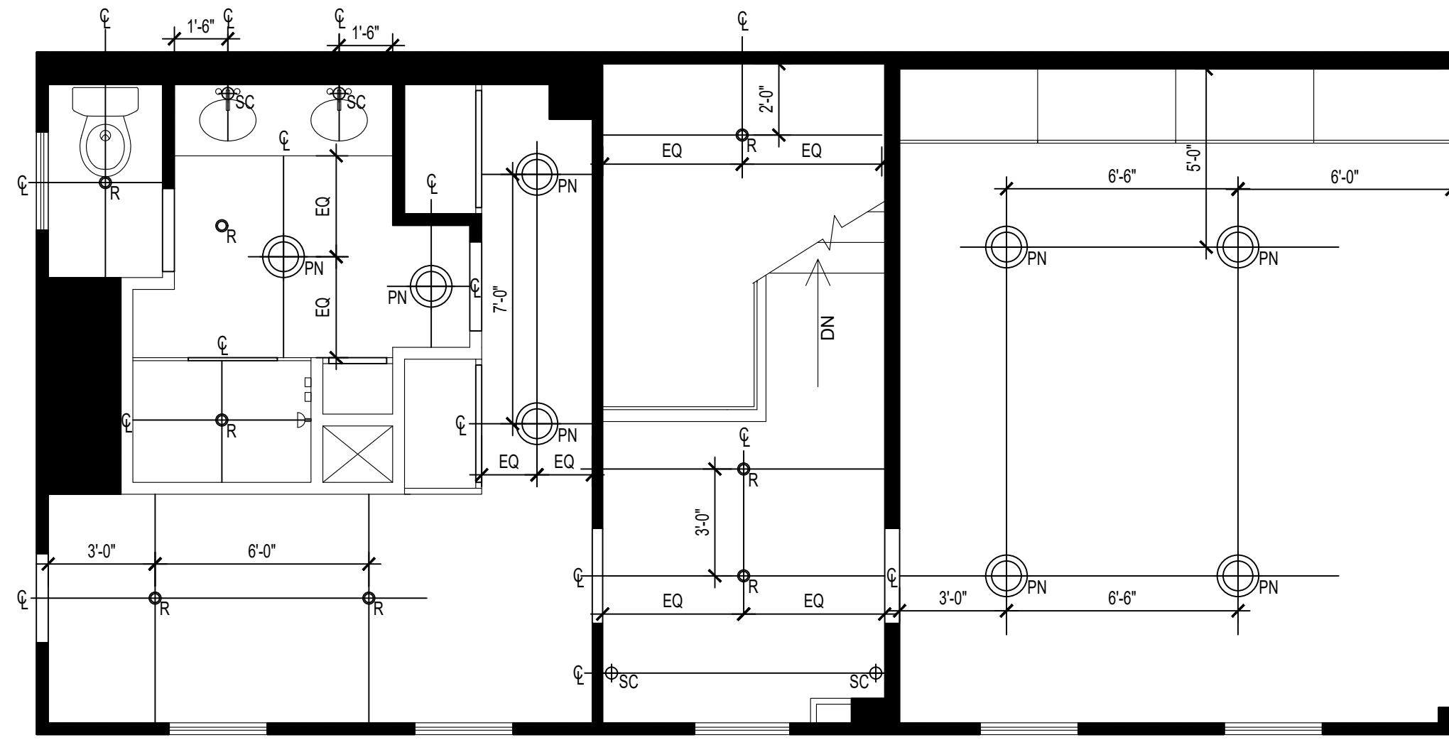
3 UPPER FLOOR REFLECTED CEILING PLAN SCALE = 1/4"=1'-0"
