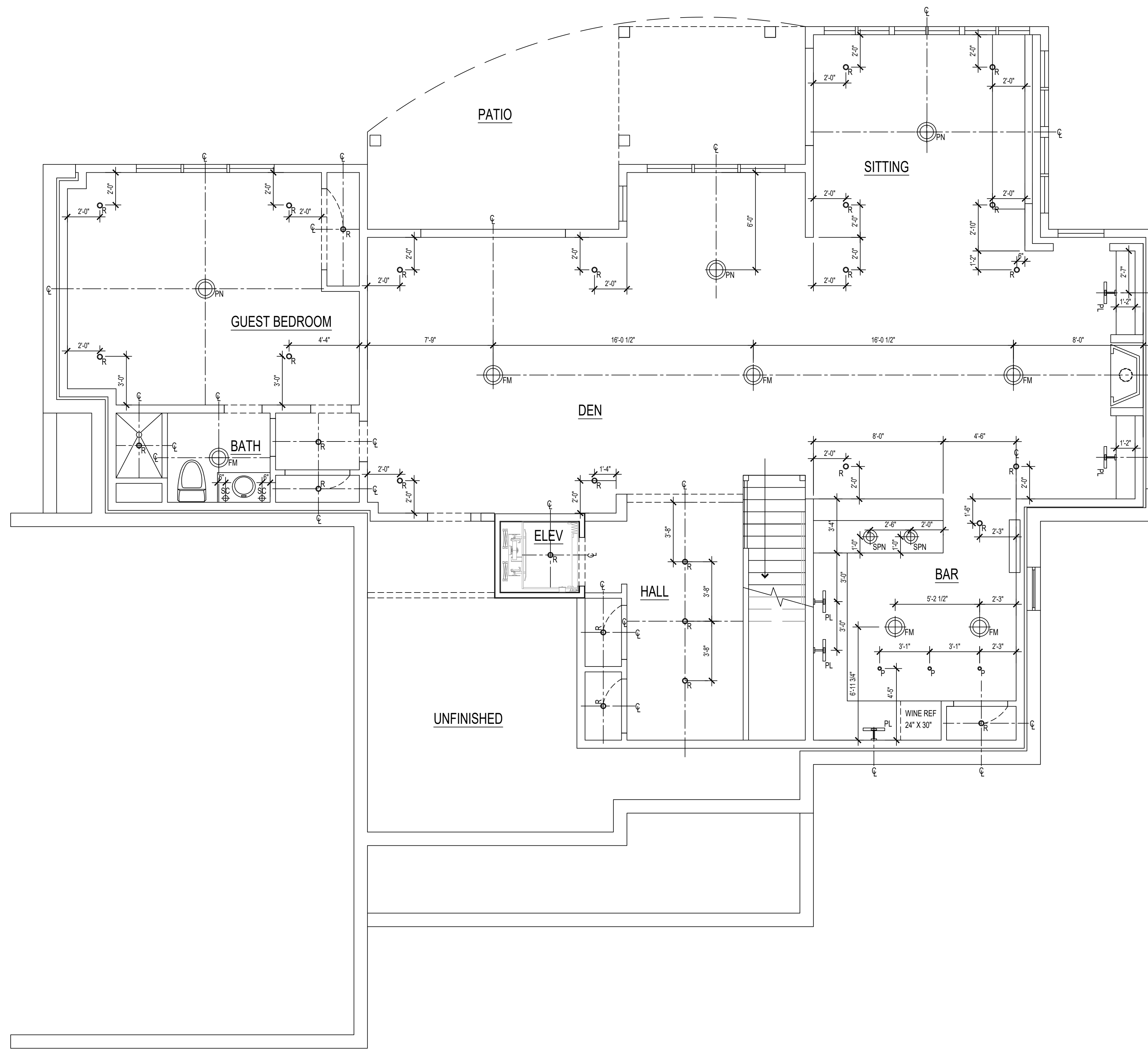
1 LOWER LEVEL REFLECTED CEILING PLAN A2 SCALE = 1/4"=1'-0"
