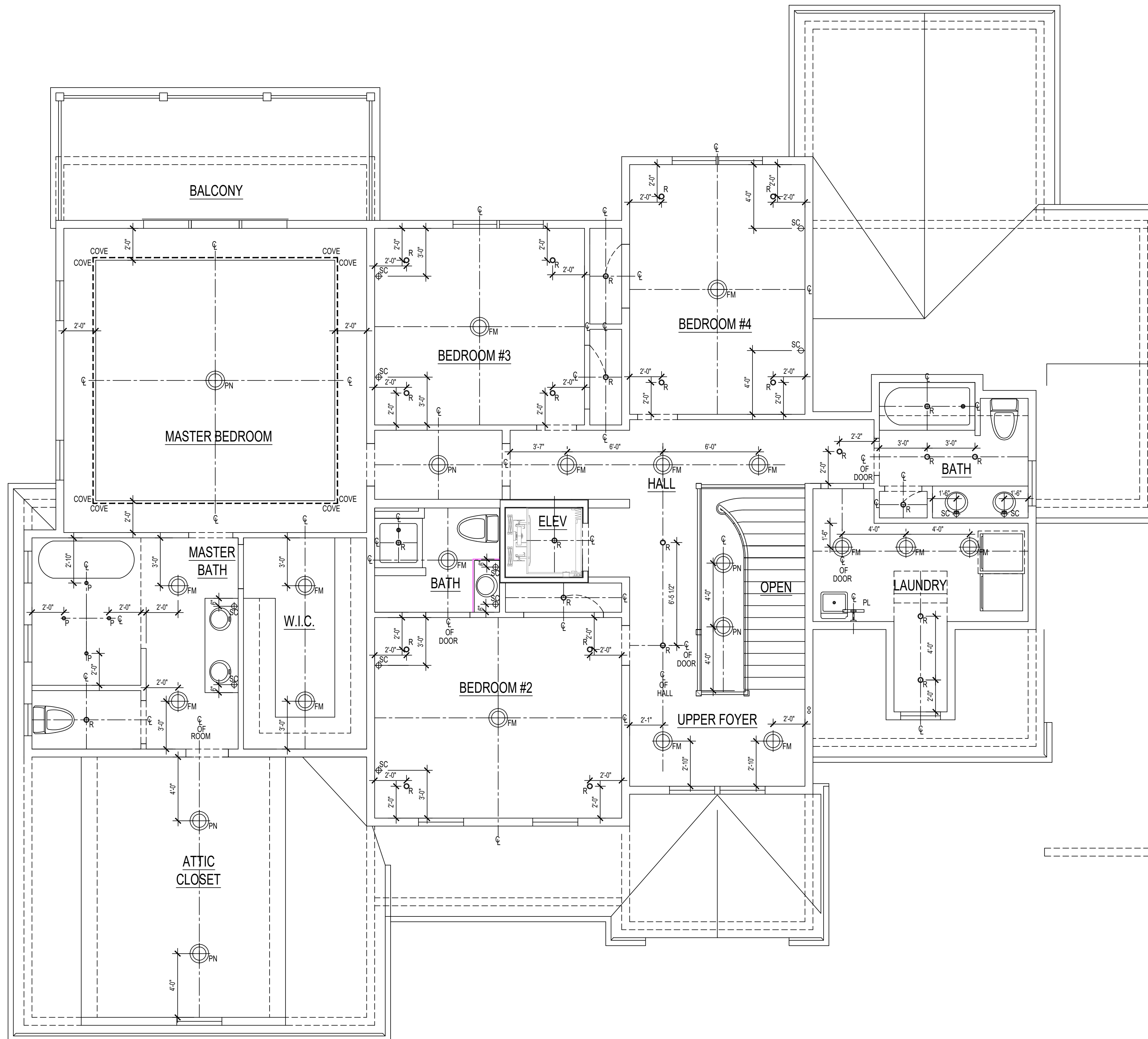
1 SECOND FLOOR REFLECTED CEILING PLAN A2.2 SCALE = 1/4"=1'-0"
