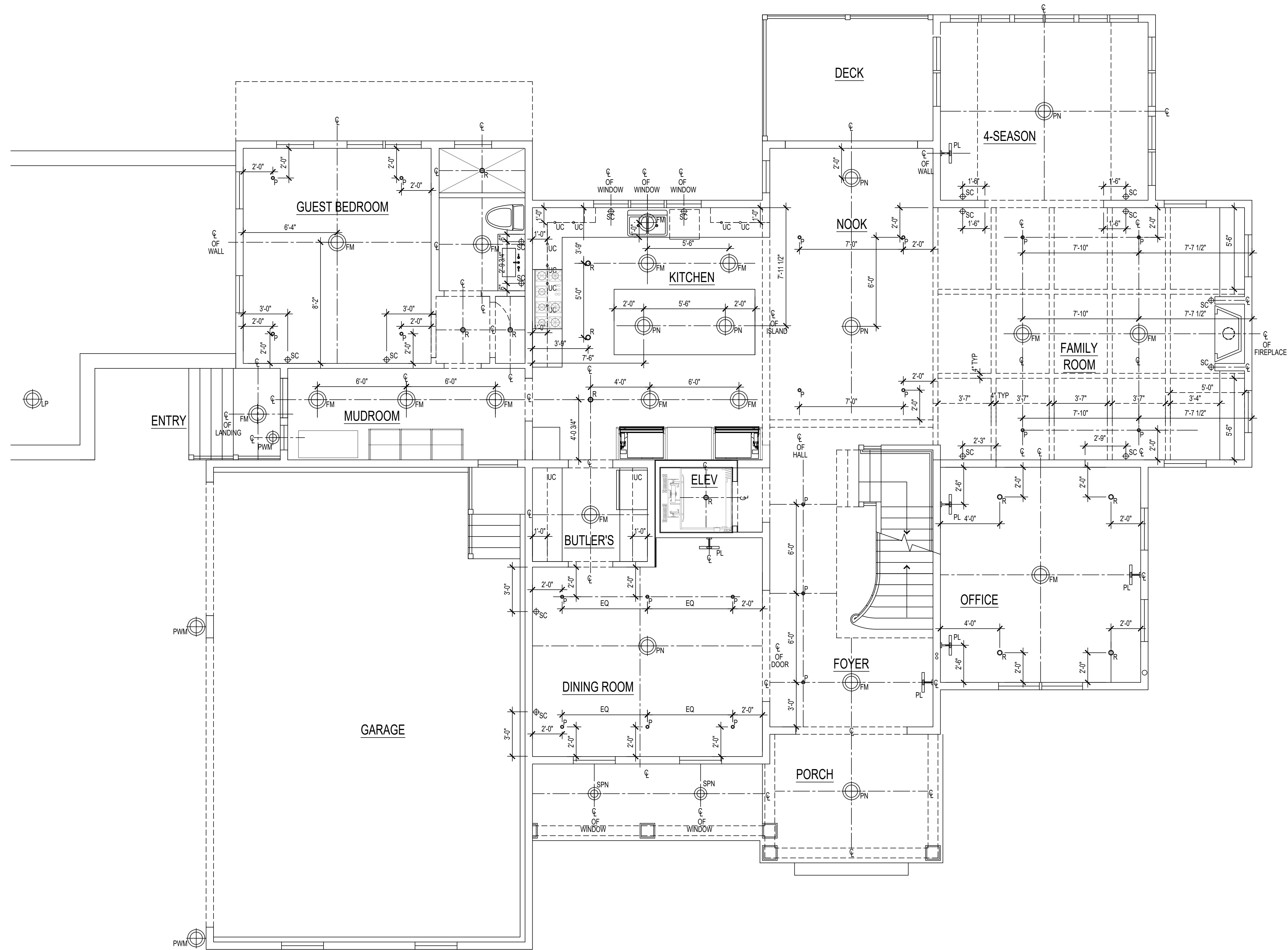
1 FIRST FLOOR REFLECTED CEILING PLAN A2.1 SCALE = 1/4"=1'-0"
