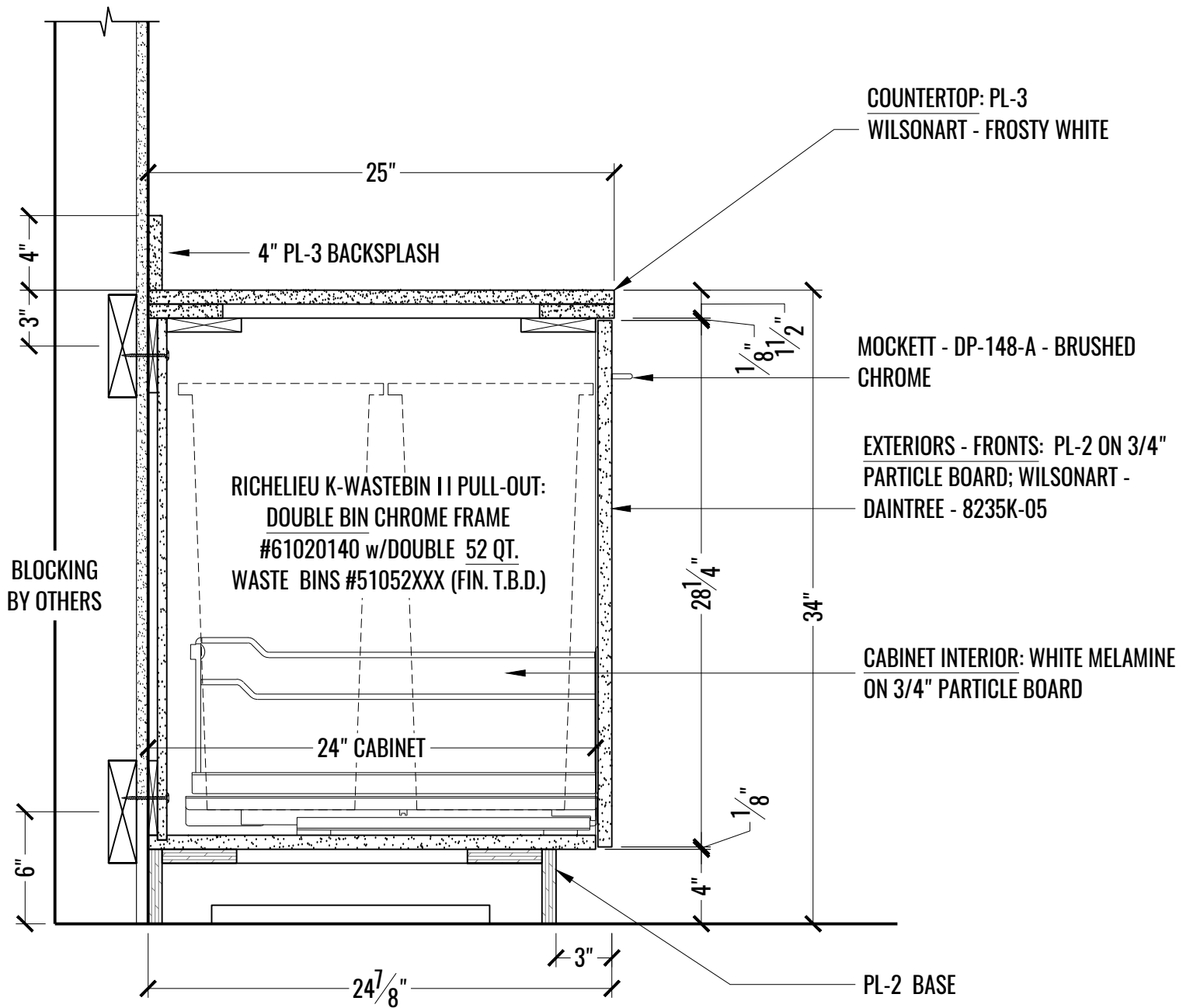
1 SECTION: TRASH/RECYCLE PULLOUT @ EX SEARCH/COPY/PRINT - 1701 A SCALE: 1-1/2" = 1'-0"
