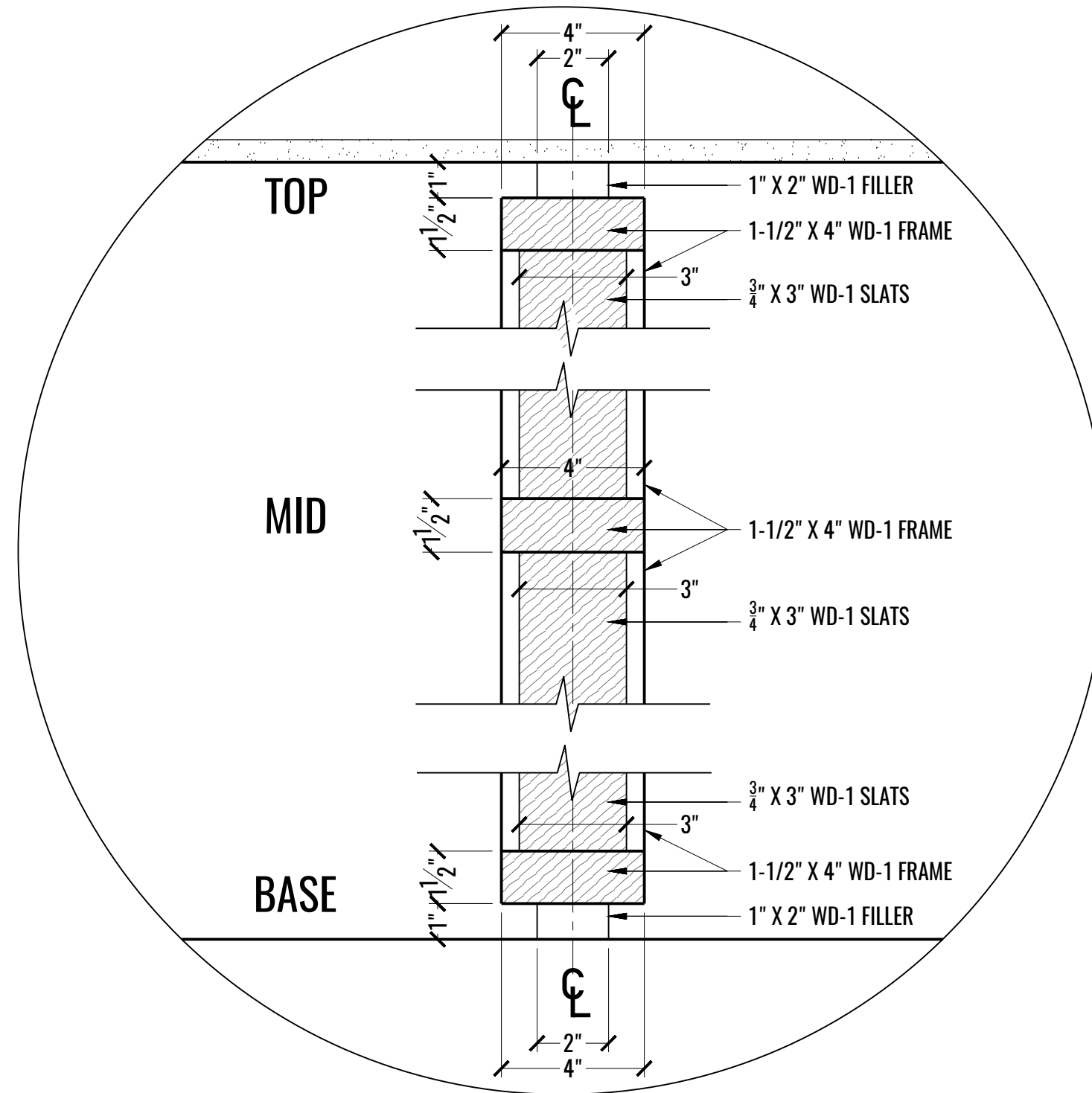
1 SECTION: WOOD SCREEN PANEL A SCALE: 3" = 1'-0"
