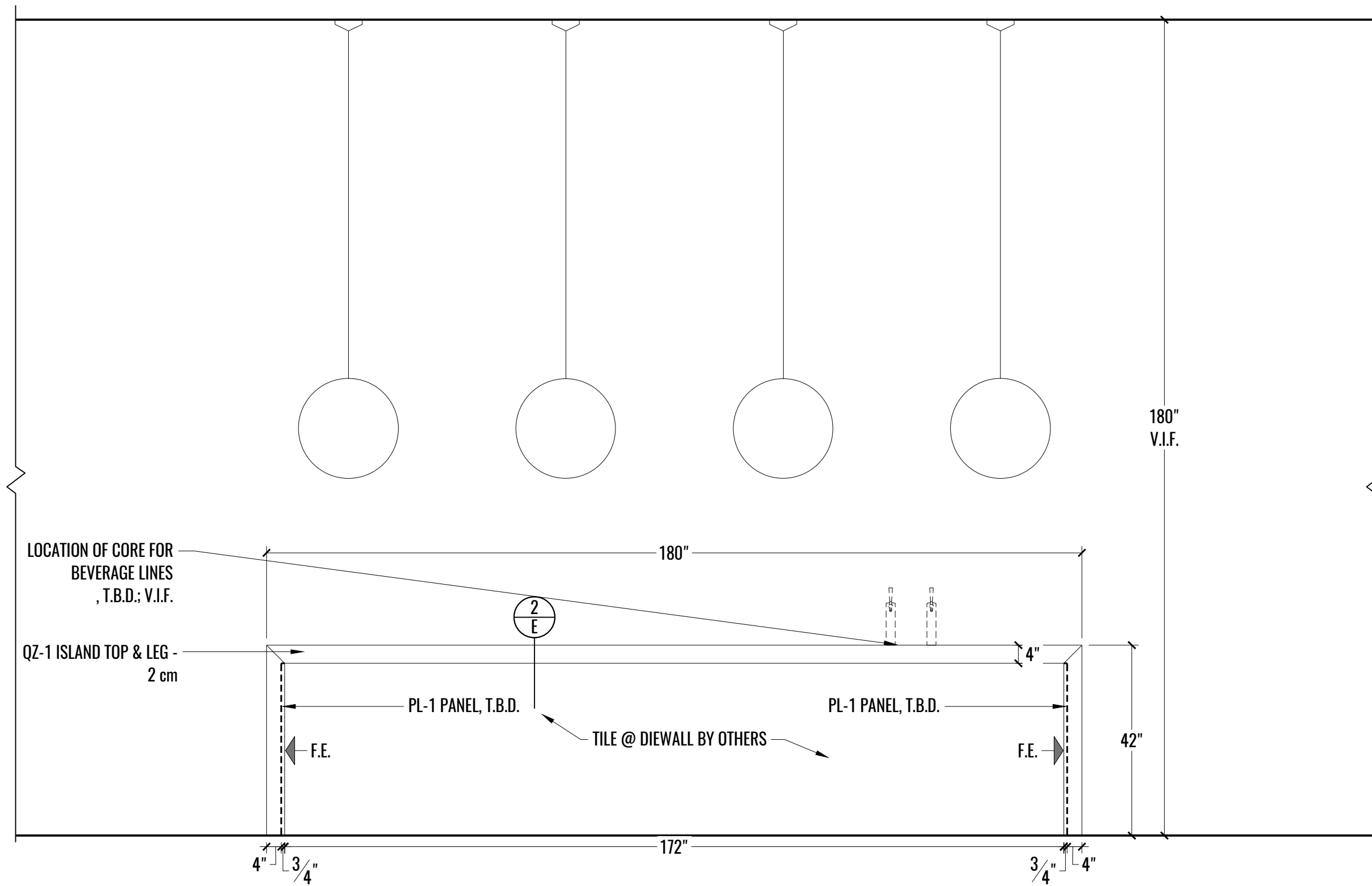
1 ELEVATION: KITCHEN ISLAND RM# 303 @ SEATING SIDE 6 SCALE: 1/2" = 1'-0"
