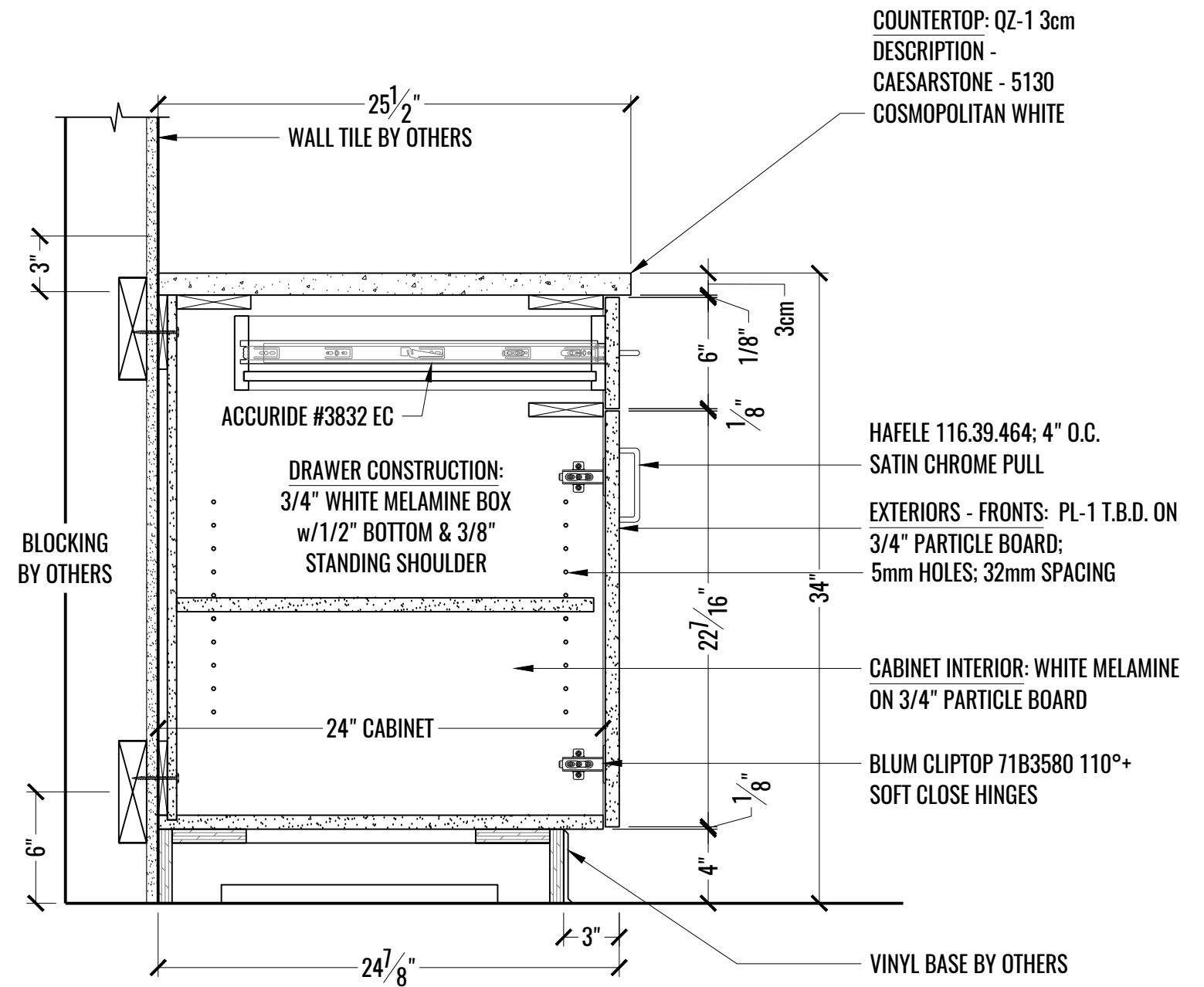
2 SECTION: KITCHEN RM# 303 - BASE CABINETS A SCALE: 1-1/2" = 1'-0"
