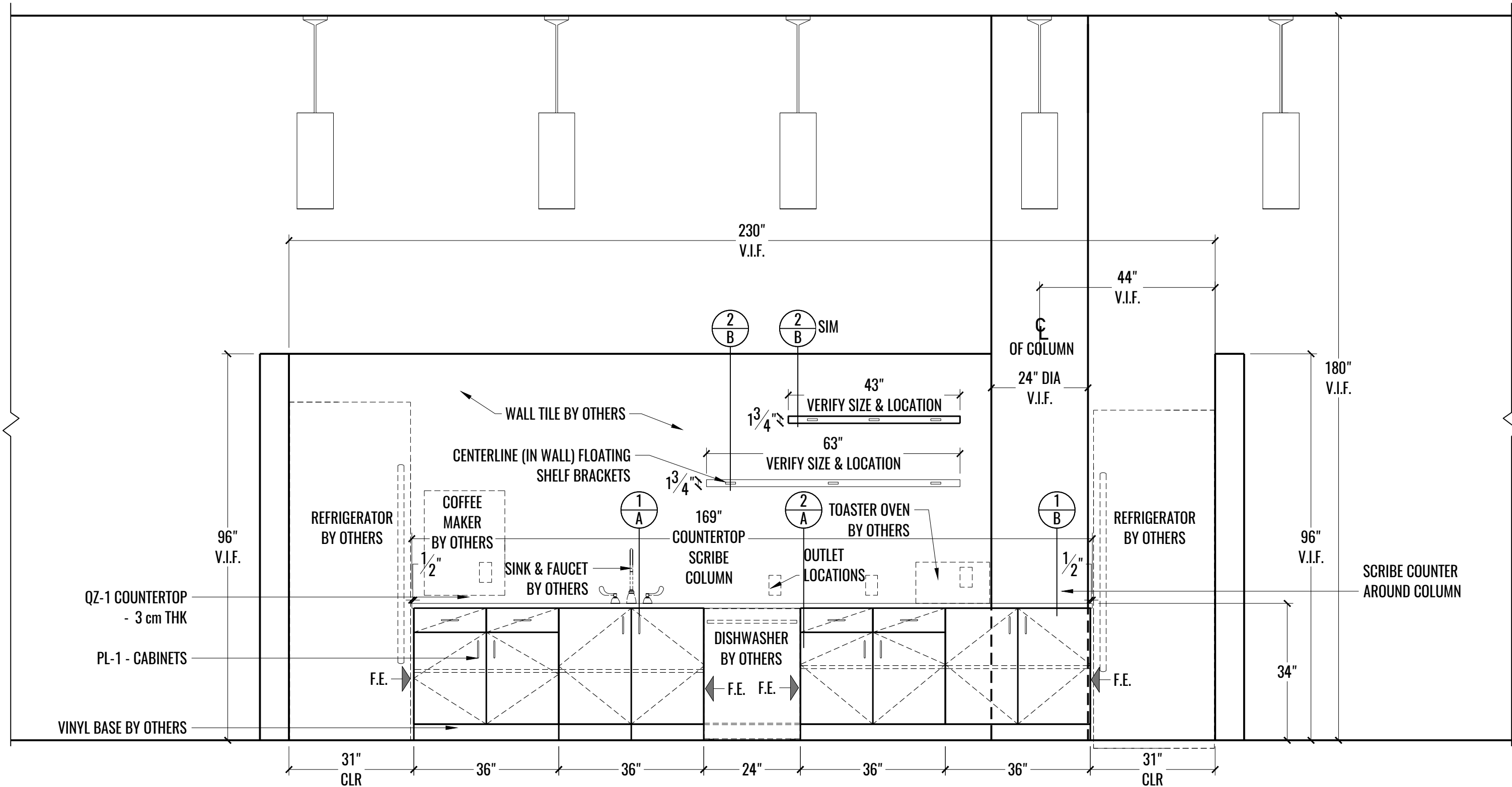
1 3 ELEVATION: KITCHEN RM# 303 @ WALL SCALE: 1/2" = 1'-0"
