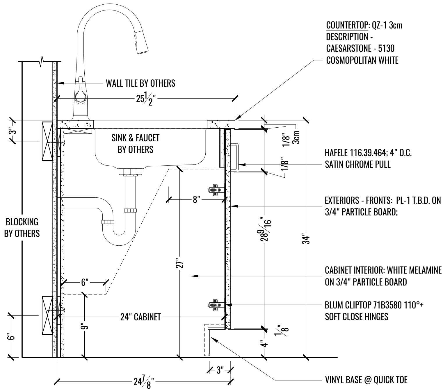
1 SECTION: KITCHEN RM# 303 @ SINK A SCALE: 1-1/2" = 1'-0"
