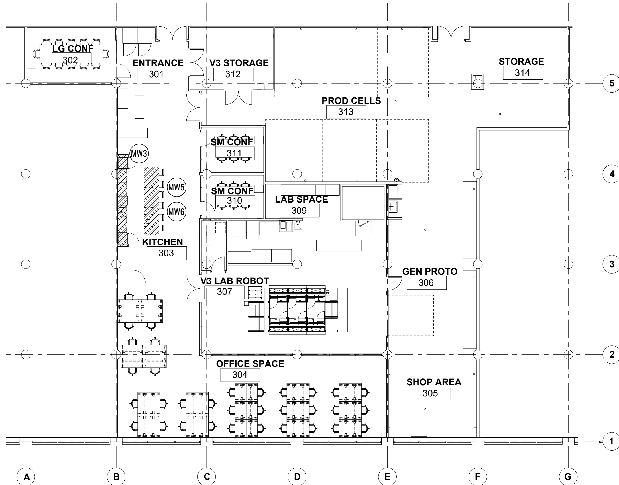
1 PLAN: PROJECT SCOPE - KITCHEN LEVEL THREE 1 SCALE: NOT TO SCALE
