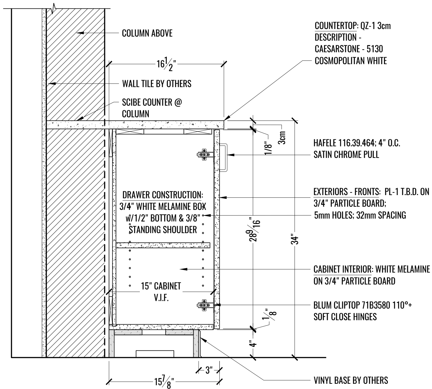
1 SECTION: KITCHEN RM# 303 - BASE CABINET @ COLUMN B SCALE: 1-1/2" = 1'-0"
