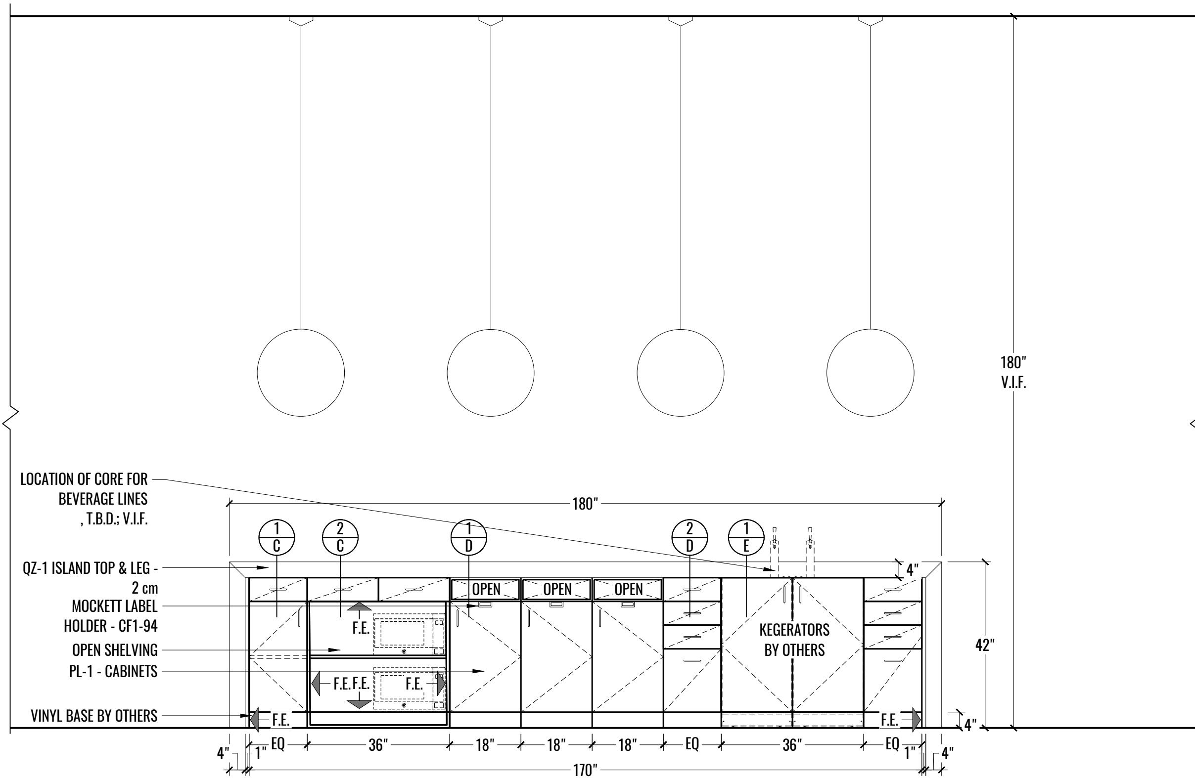
1 ELEVATION: KITCHEN ISLAND RM# 303 @ (BACK SIDE) 5 SCALE: 1/2" = 1'-0"
