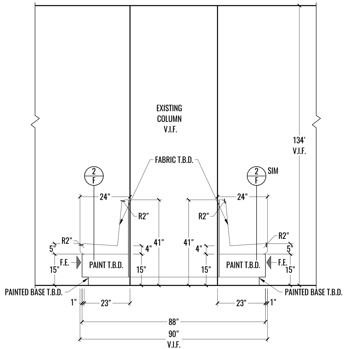
2 ELEVATION: WORK LOUNGE - BANQUETTE - 1502 8 SCALE: 1/2" = 1'-0"
