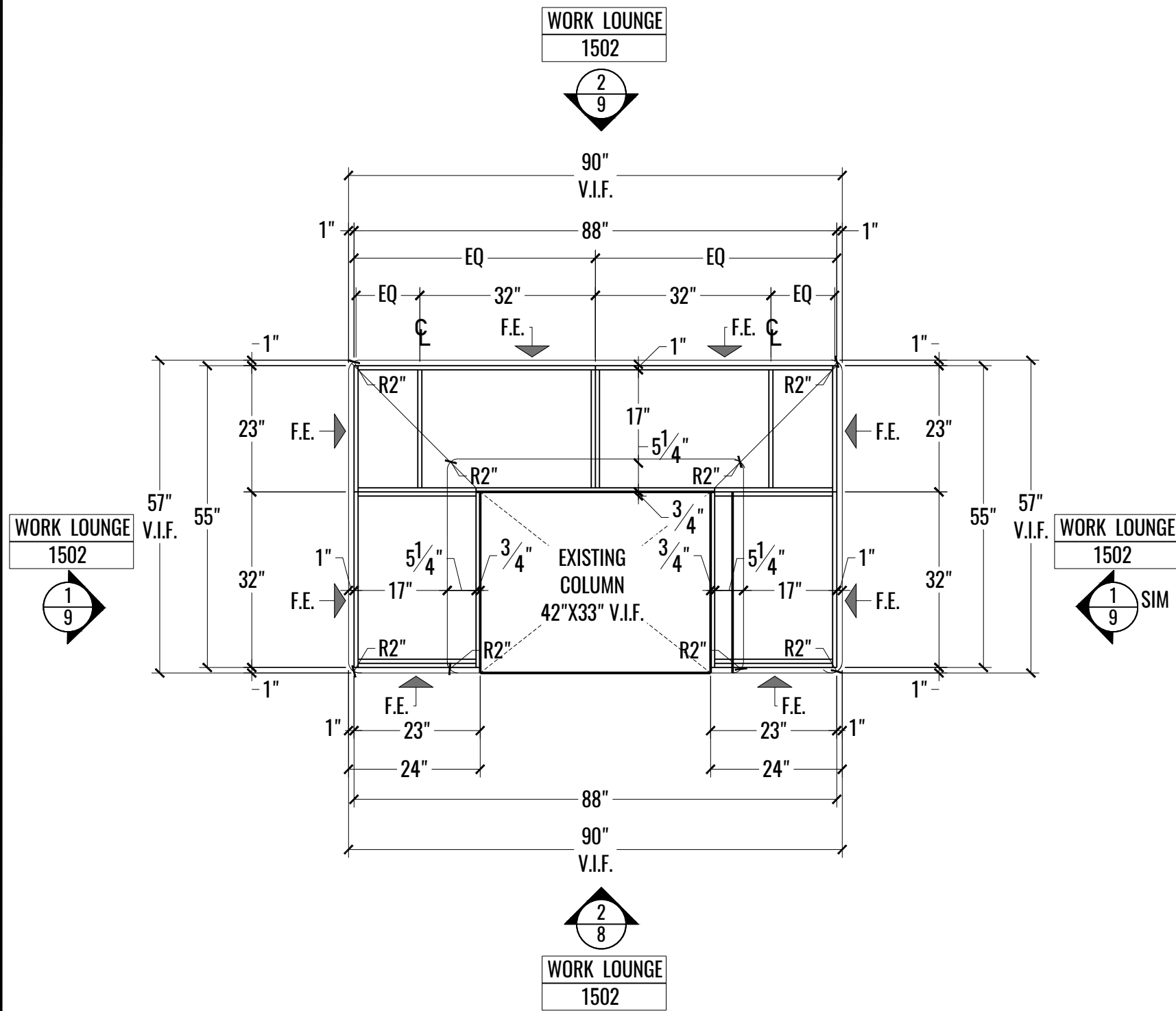
1 PLAN: WORK LOUNGE - BANQUETTE - 1502 8 SCALE: 1/2" = 1'-0"
