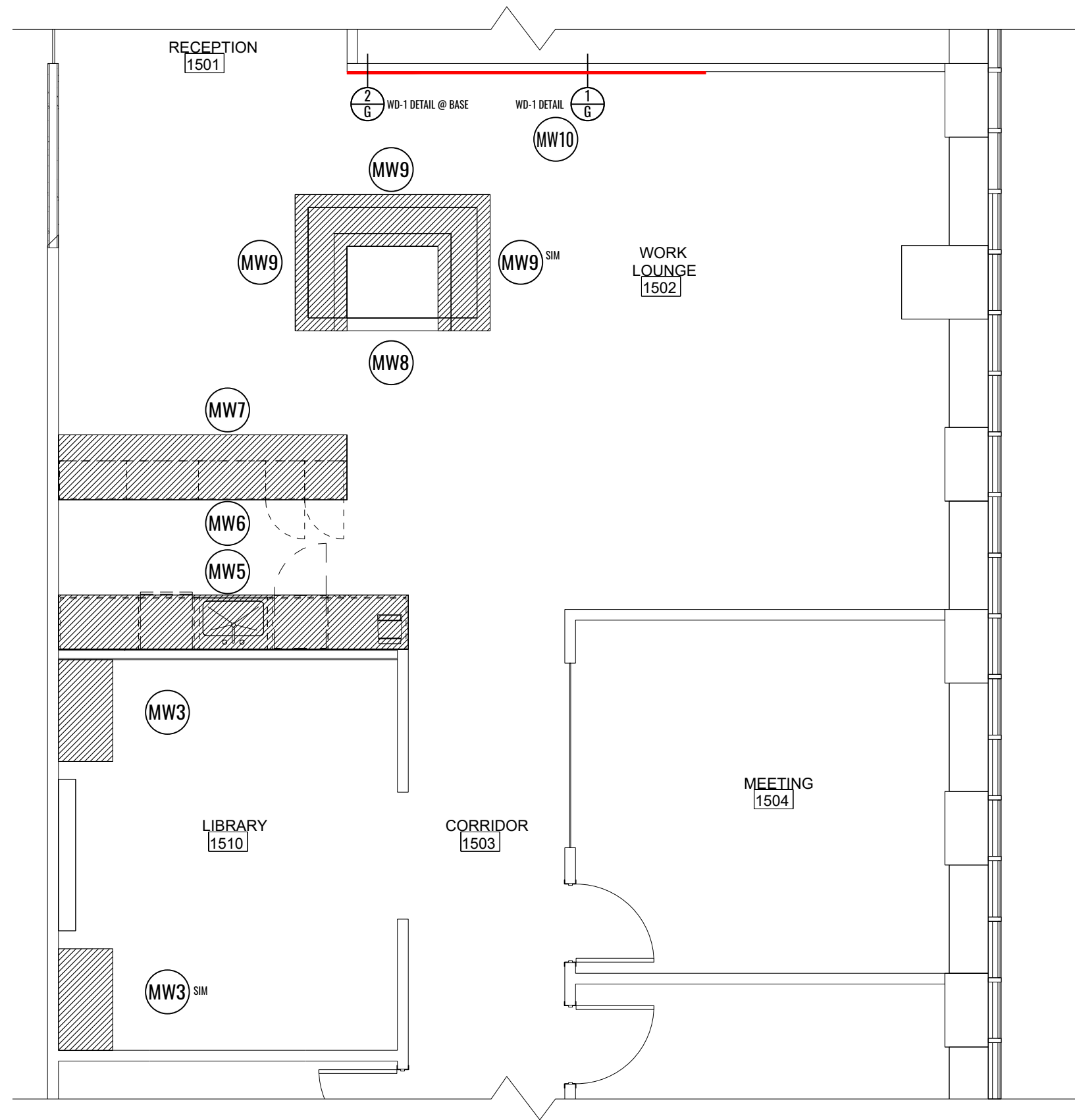
1 PLAN: PROJECT SCOPE - 15TH FLOOR 1 SCALE: NOT TO SCALE
