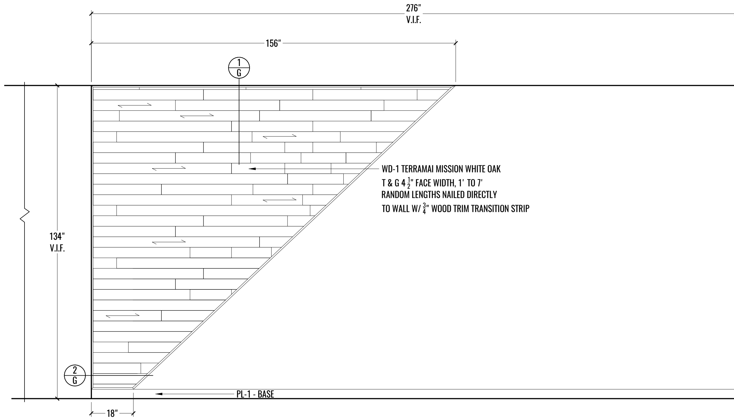
1 10 ELEVATION: WORK LOUNGE - WD-1 FEATURE WALL - 1502 SCALE: 1/2" = 1'-0"
