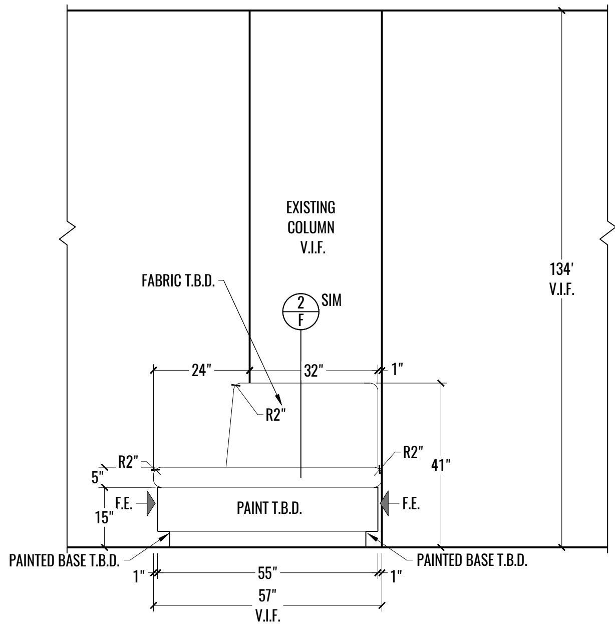
1 PLAN: WORK LOUNGE - BANQUETTE - 1502 9 SCALE: 1/2" = 1'-0"
