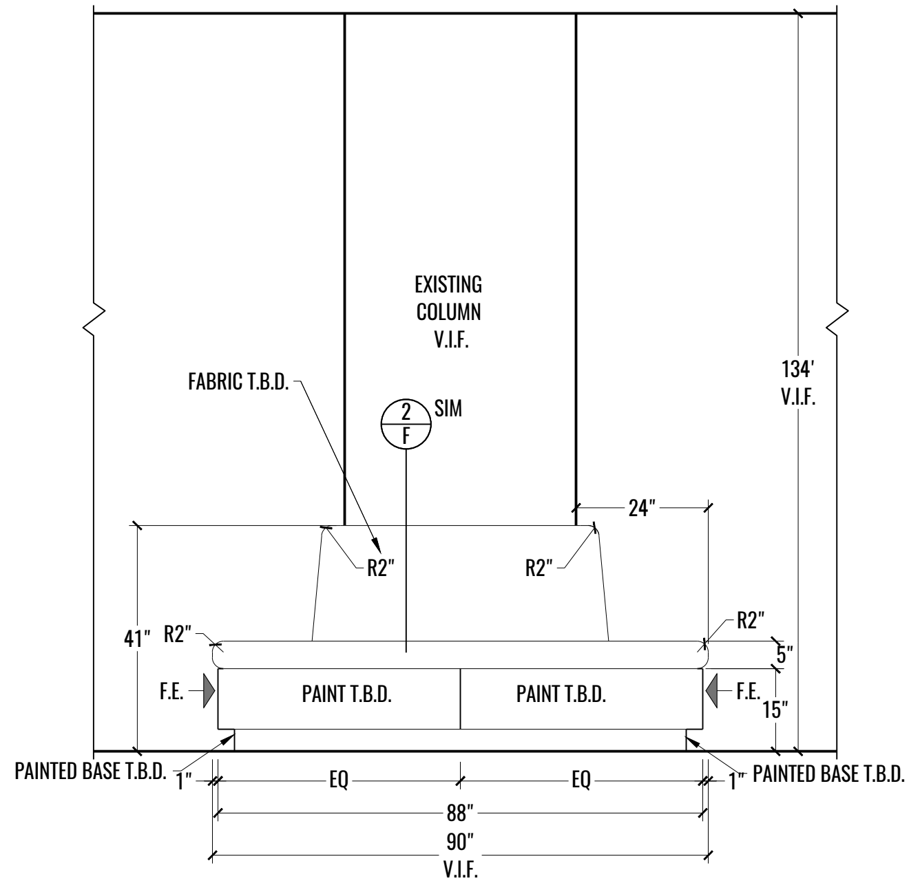
2 ELEVATION: WORK LOUNGE - BANQUETTE - 1502 9 SCALE: 1/2" = 1'-0"
