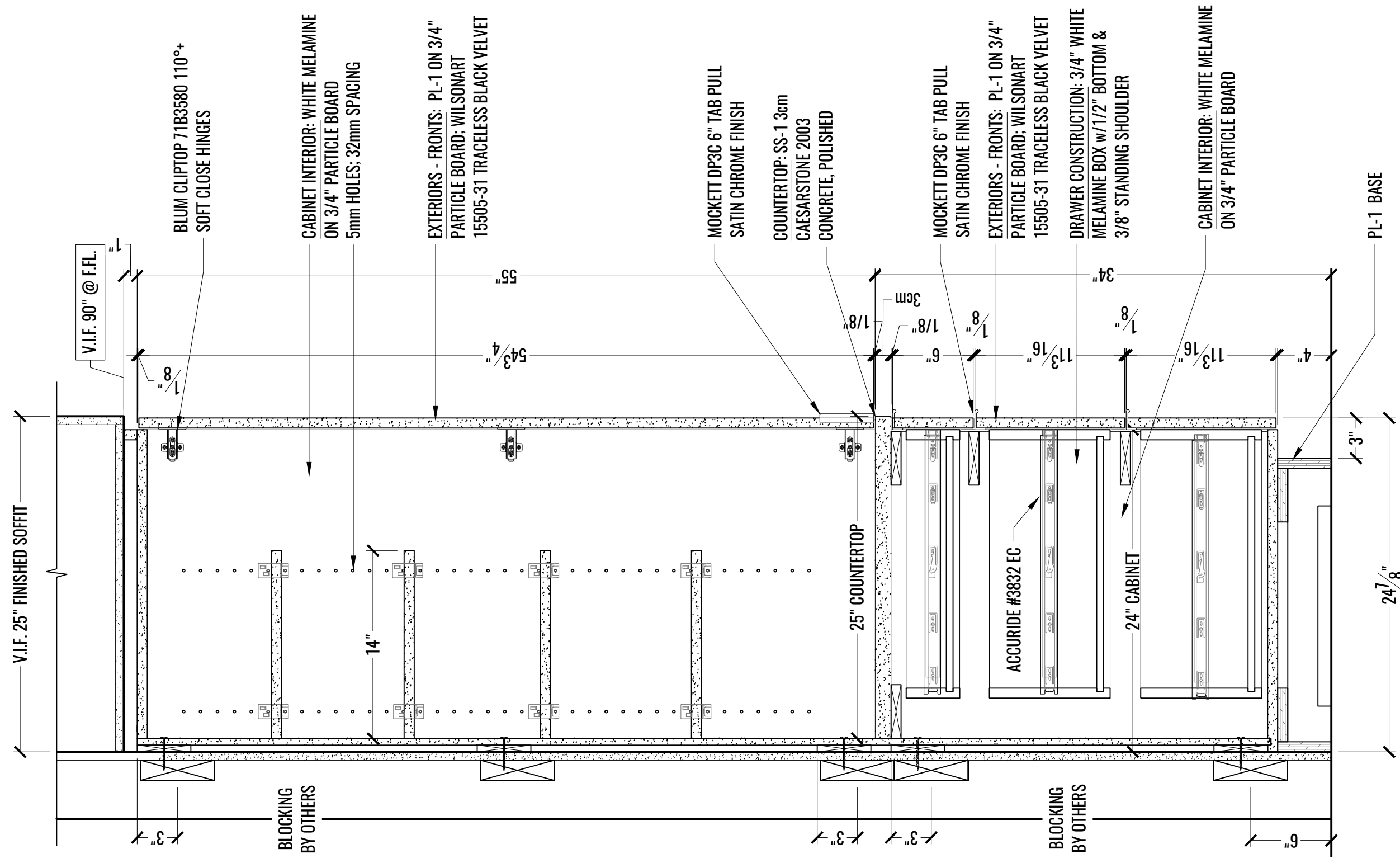
1 SECTION: TALL CABINET W/DRAWERS @ WORK LOUNGE - 1502 D SCALE: 1-1/2" = 1'-0"
