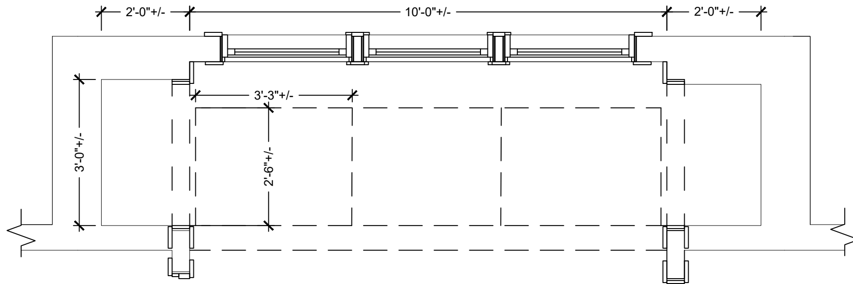
WINDOW SEAT PLAN (UPSTAIRS) - OPT 1
