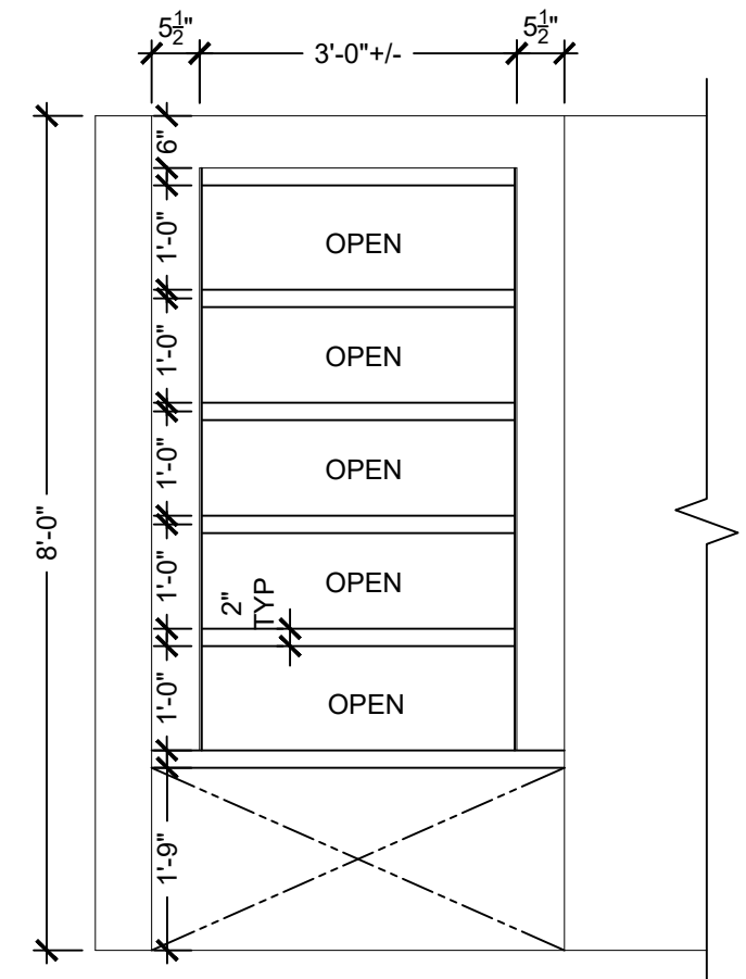
SIDE BOOKSHELVES ELEVATION
