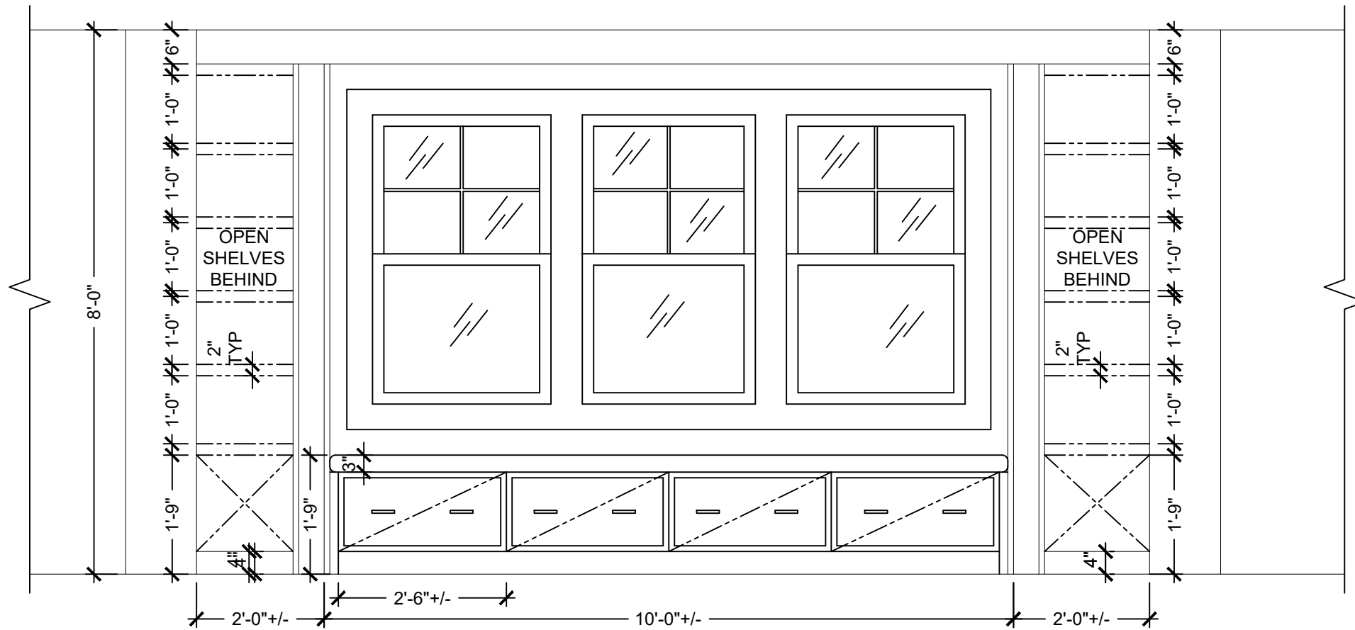
WINDOW SEAT ELEVATION (UPSTAIRS) - OPT 2
