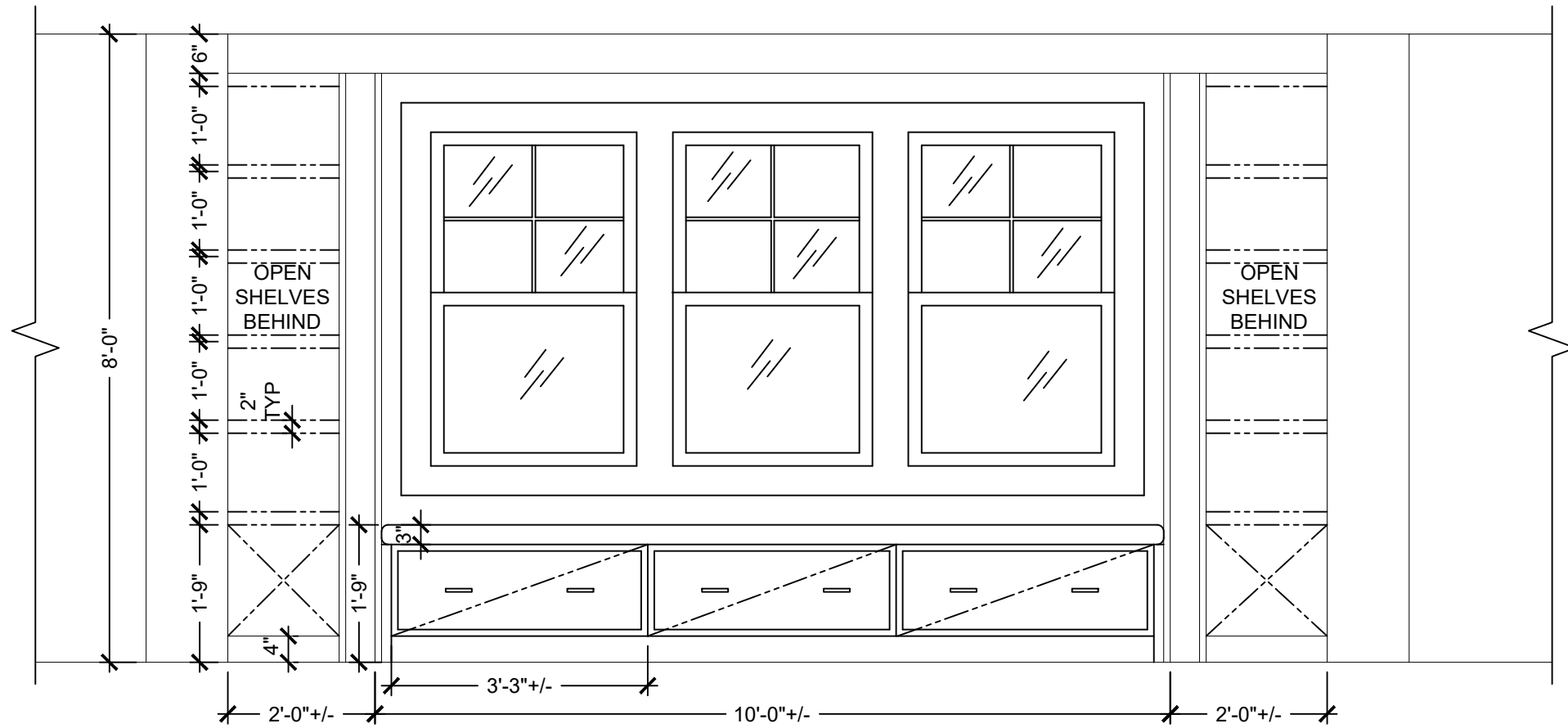
WINDOW SEAT ELEVATION (UPSTAIRS) - OPT 1
