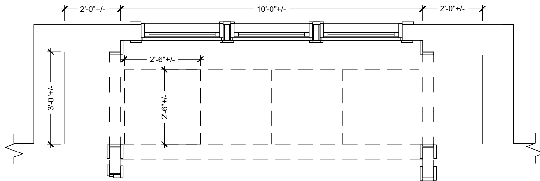
WINDOW SEAT PLAN (UPSTAIRS) - OPT 2
