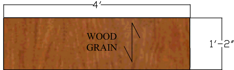
CONFERENCE ROOM BUILT-IN (TOP) PLAN VIEW
