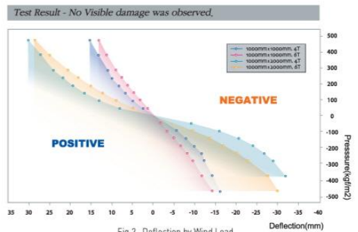
Fig.2, Deflection by Wind Load
