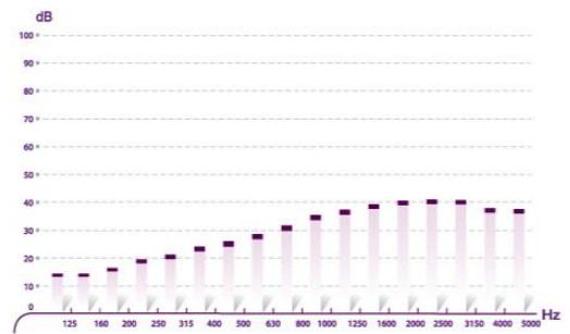
Fig.1. Sound Transmission Loss for 4mm ALCOPANEL
