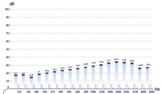
Fig.1, Sound Transmission Loss for 4mm ALCOPANEL FR
