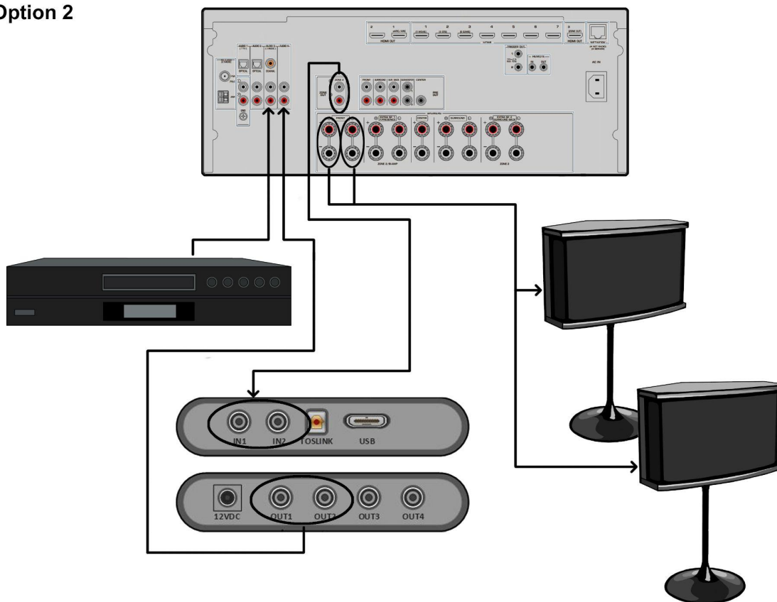
Diagram 2. Using zone 2 loop
