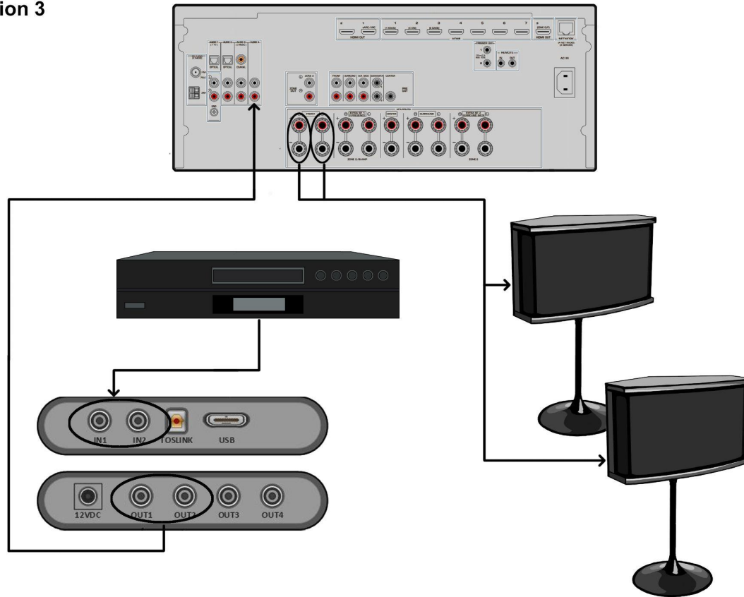
Diagram 3. Using only a single source
