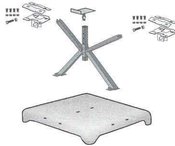
Foundation Base Pad 531-59326
