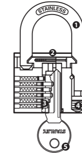
Standard Shackle Padlock
