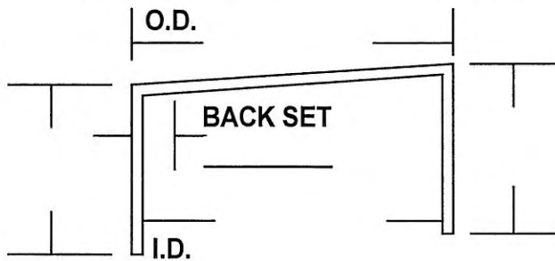
LH/RHR TOP VIEW
