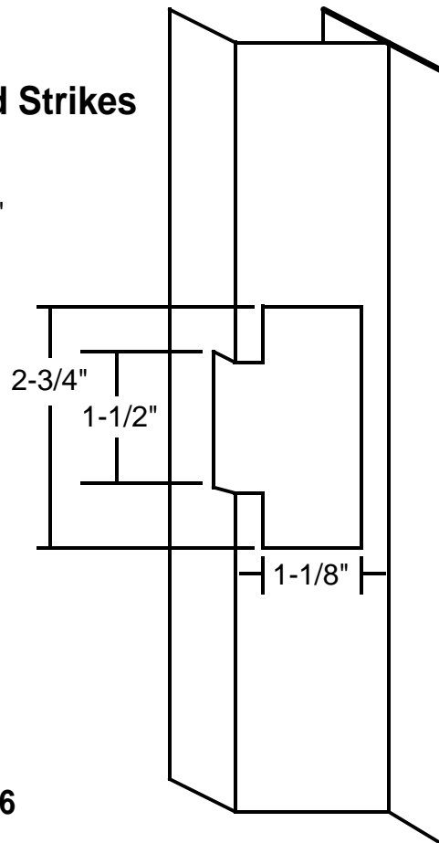
ASA Strike 4-7/8" X 1-1/4" w/ 3-3/8" Lip
