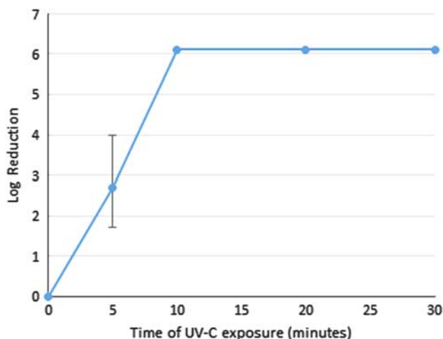
FIGURE 1. Log reduction of MHV-A59 following Surfaced UV-C exposure at a 4-foot distance (1.22 m). Virus was reduced by 2.71 log 10 in 5 minutes and by 6.11 log 10 in 10 minutes to undetectable levels. Results are the means of triplicate samples.
