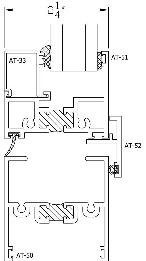
16 SILL @ PIVOT POINT
