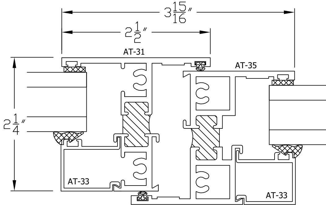
9 VENT @ RIGHT OF FIXED
