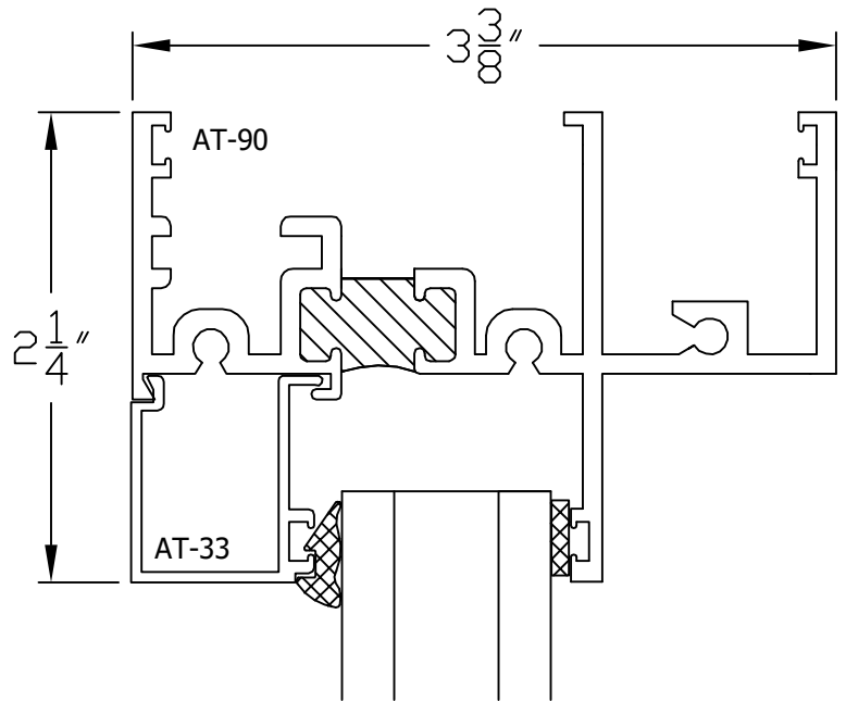
⑤ HEAD @ FIXED
