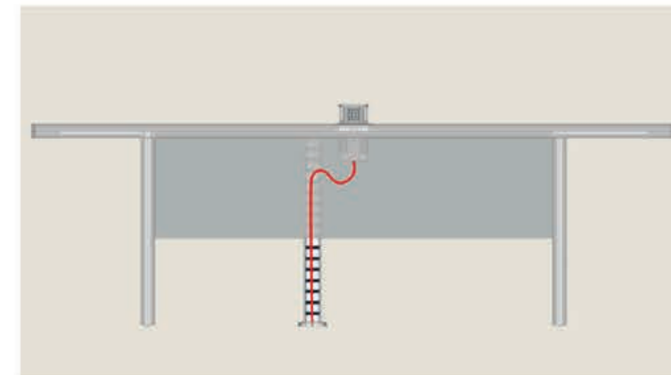
Conference table wiring diagram
