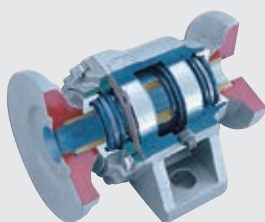
TAPERED BEARINGS AND DUO-CONE TYPE SEALS.
