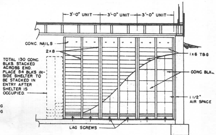
Front Elevation
