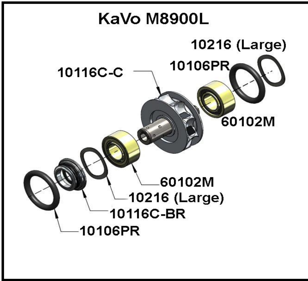
KaVo M8900L Repair Diagram
