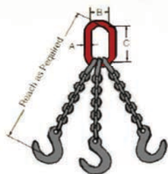
Triple Leg
