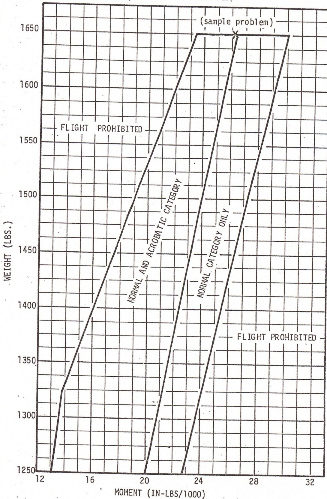
FIGURE 5-4 FLIGHT ENVELOPE - 7GCAA, 7KCAB ONLY
