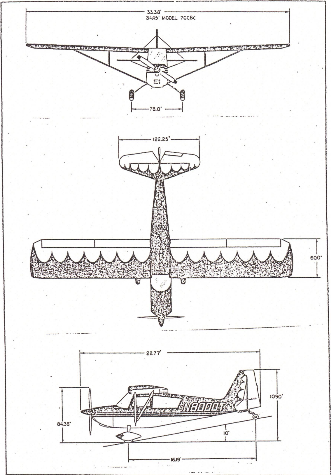
FIGURE 6-2 CITABRIA THREE-VIEW
