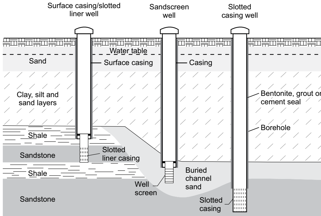
Figure 3-4, Well Completions
