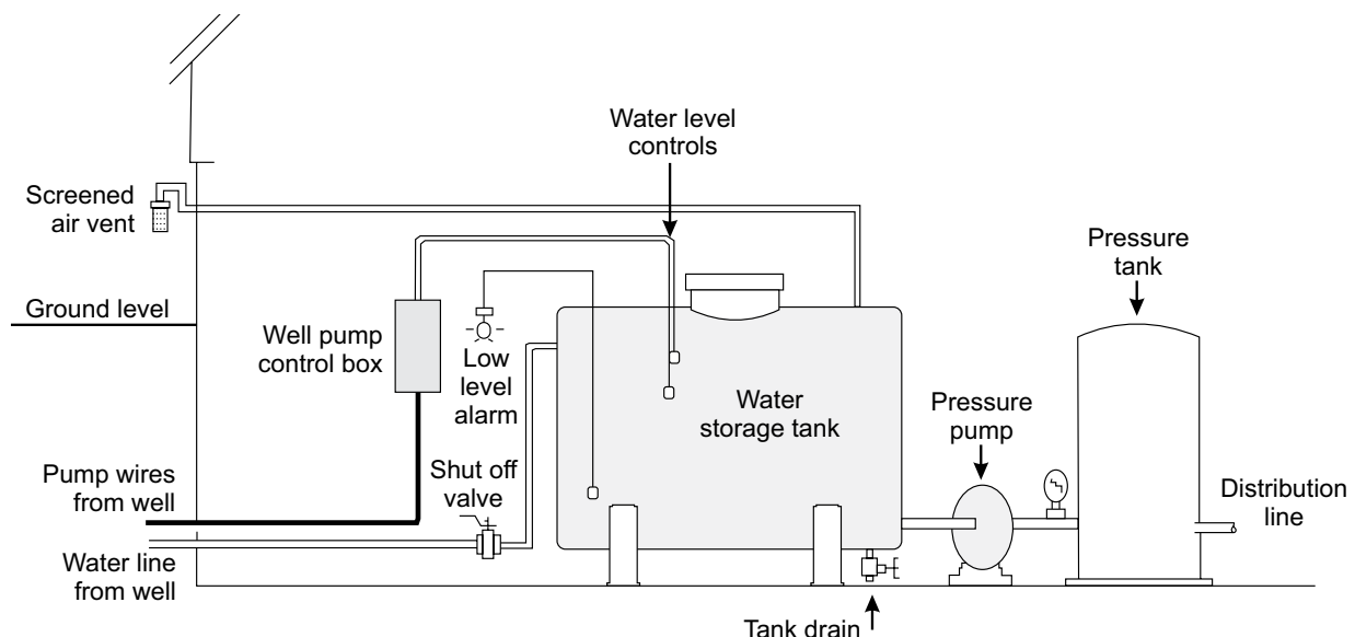
Figure 3-7, Components of an Additional Water Storage System
