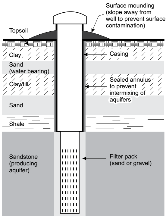
Figure 3-5, Annular Seal
