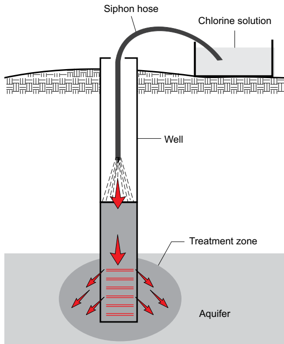
Figure D-1 Siphoning Chlorine Solution
