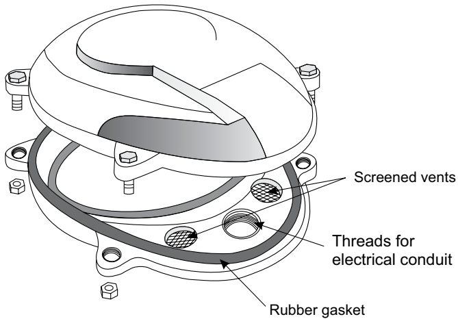
Figure 4-5, Examples of Standard Well Caps
