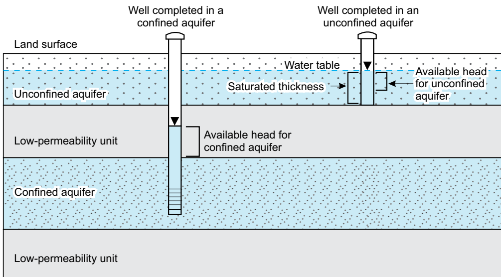
Figure 3-6, Available Head
