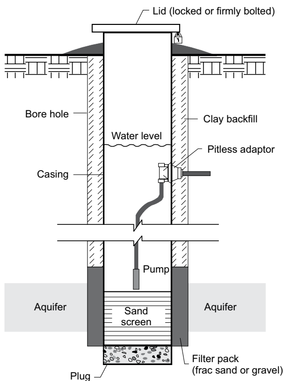
Figure 3-2, Bored Well
