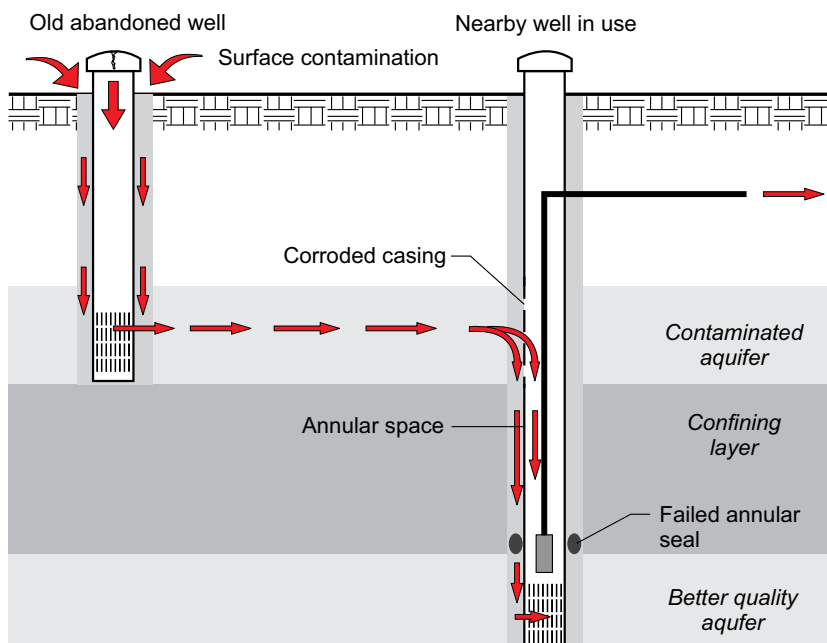
Figure 8-1, Well Contamination
