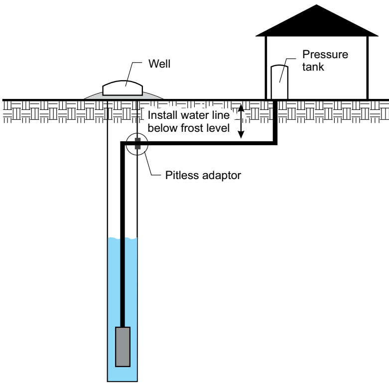
Figure 4-2, Pitless Adaptor
