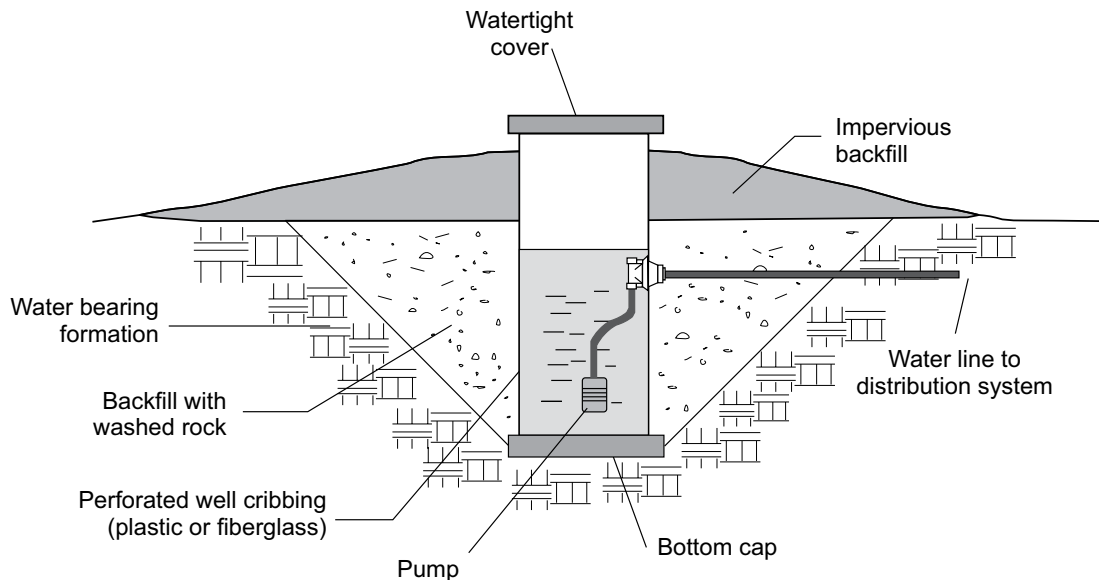
Figure 3-3, Dug Well
