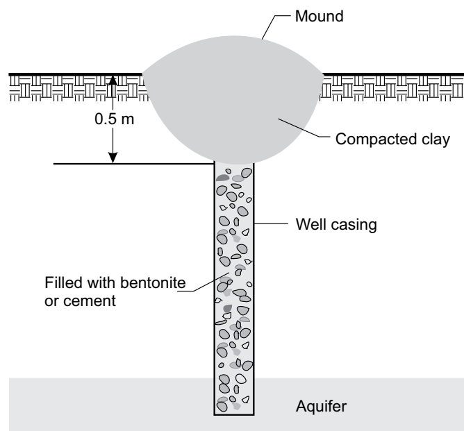
Figure 8-4, Cutting Off Casing and Mounding Clay
