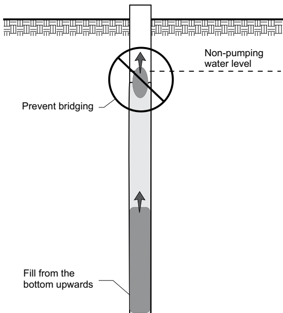
Figure 8-2, Bridging of Fill Material
