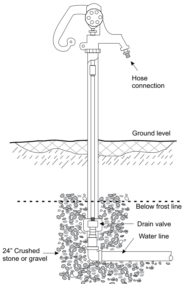
Figure 4-6, Frost-Free Hydrant
