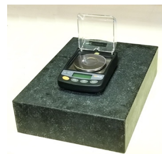
Powder Scale on 9"x12"x3" Granite
