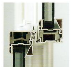
Non-metal Reinforcement at Interlock
