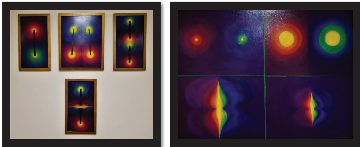
Left: Red-Orange Male and Blue-Green Female Poles of Multiple Gravity Bars (Magnets); Right: Scientific Painting Showing Red-Orange Male and Green-Blue Female Poles.
