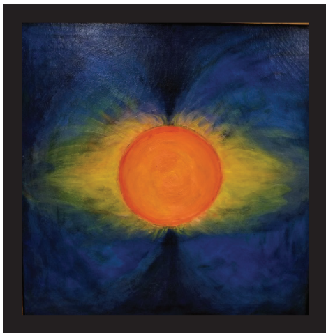
The Sun with Dark Blue Polar Caps Centripetally Converging Inward and Golden Centrifugal Discharge Fanning Out from the Equatorial Rim (Left); The Earth and Moon Showing Spectrum Colors of Waves in Octave Tonal Positions (Right).
