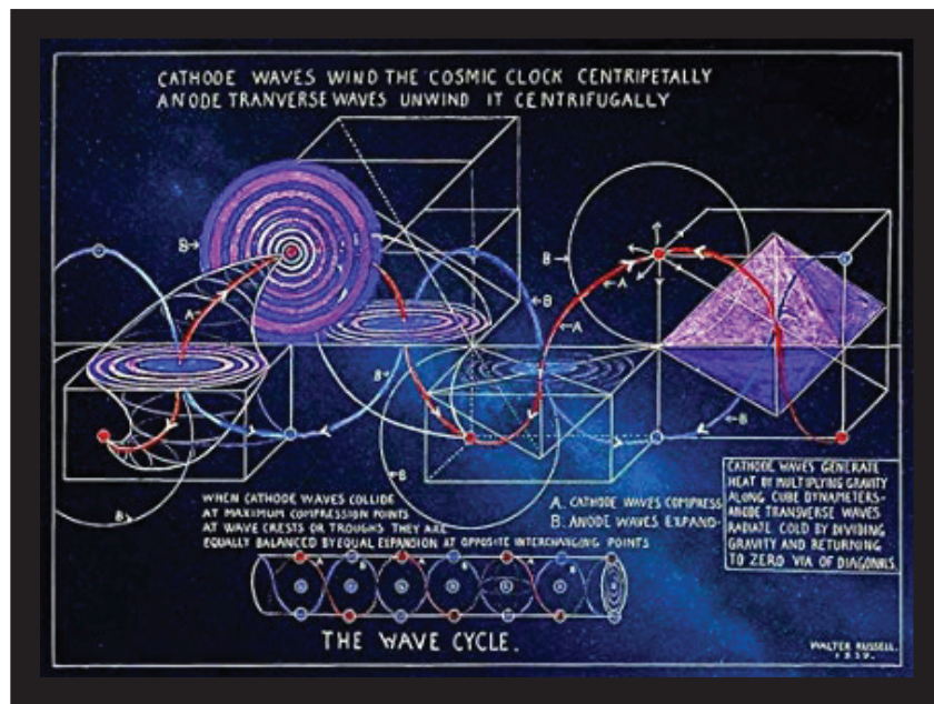
The Wave Cycle.
