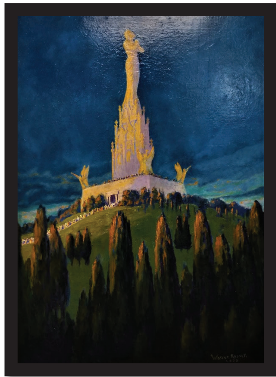
Left: The Octave Wave Showing a Complete Wave Cycle (All That Exists in the Universe); Right: Christ of the Blue Ridge Painting.
