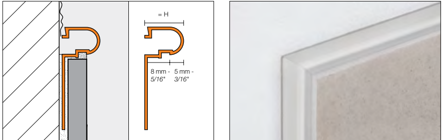
Outside corner (90°)
