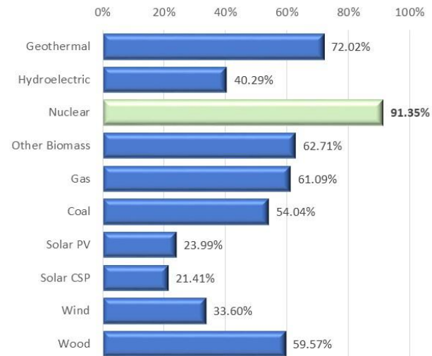
Average USA Capacity Factors (2011-20)
