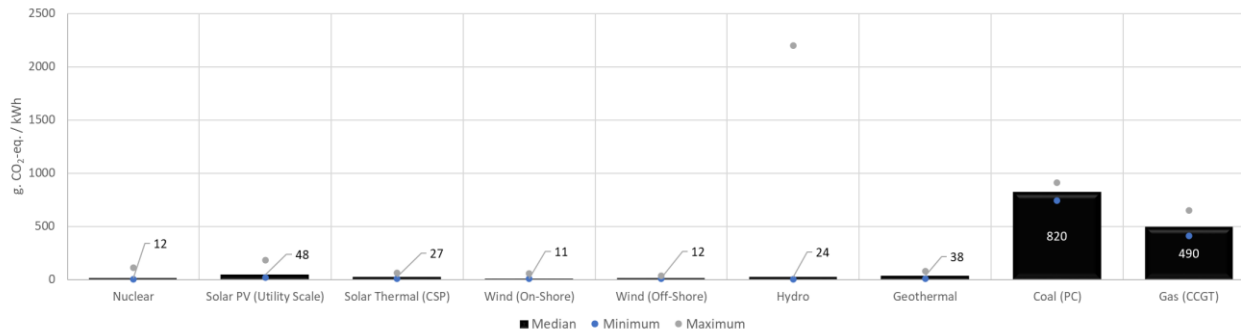
World Life-Cycle Carbon Emissions for Different Generation Technologies
