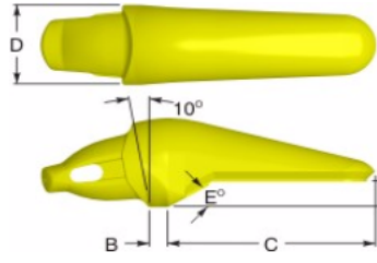
Type 2 Flush Mount
