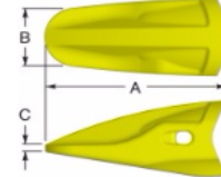
RP2 & 3 Rock Penetrator
