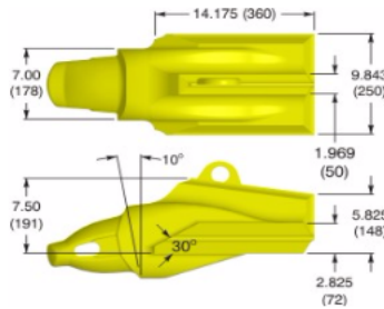
Type 4 "T" Style Corner
