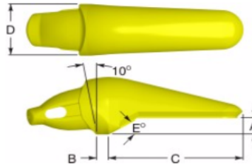
Type 2 Flush Mount
