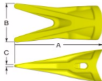
WT Twin Tiger
