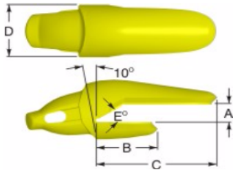
Type 1 1-1/2 Leg
