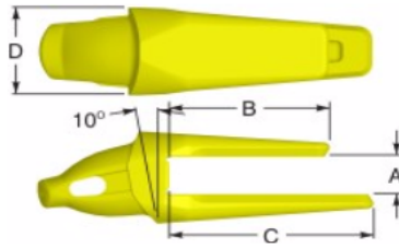
Type 5 1-1/2 Leg Blunt
