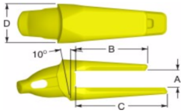
Type 5 1-1/2 Leg Blunt
