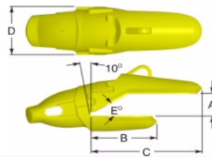
Type 4 "T" Style Corner
