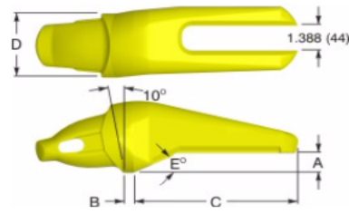
Type 9 Straddle Leg Flush Mount
