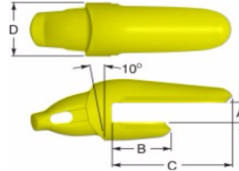
Type 5A 1-1/2 Leg Blunt
