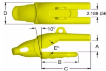
Type 8 Straddle Leg
