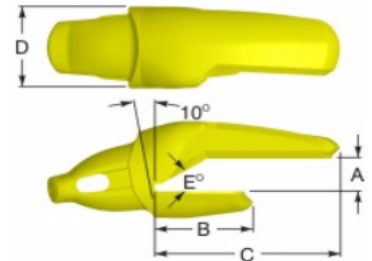
Type 3 Notched Corner
