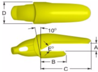
Type 1 1-1/2 Leg
