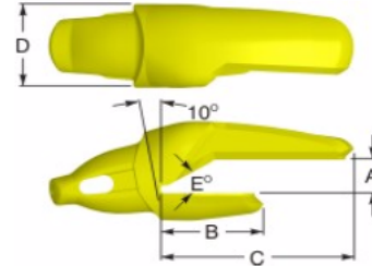
Type 3 Notched Corner
