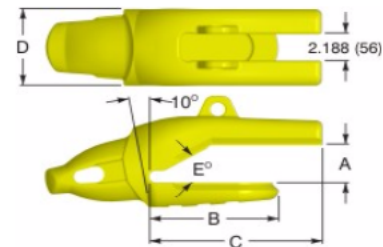
Type 8 Straddle Leg
