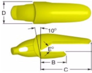
Type 1 1-1/2 Leg
