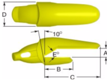
Type 1 1-1/2 Leg
