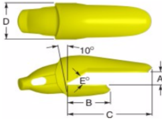
Type 1 1-1/2 Leg
