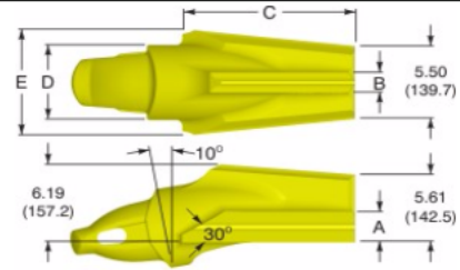
Type 4 "T" Style Corner
