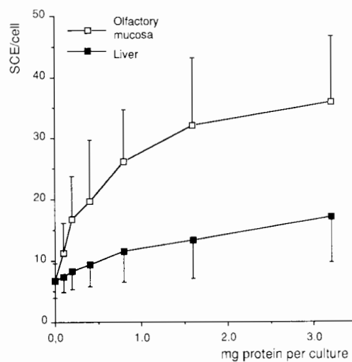
Fig. 6. The influence of various amounts of S-9 preparation from bovine olfactory mucosa or liver, present during a 1 h treatment with 0.2 \mu M AFB 1 , on the induction of SCE in CHO cells. Bars represent standard deviation of the mean.
