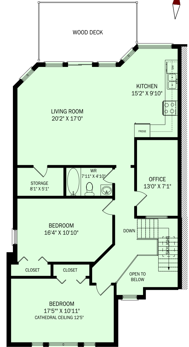
CEILING HEIGHT 8'0" SECOND FLOOR - 1280 SQUARE FEET
