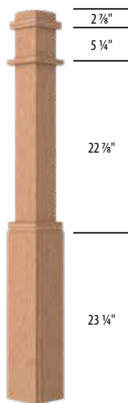
55 1/4" 5 1/2" LJ-4391CR Box Newel
