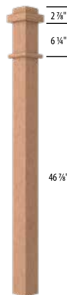
56" 3 1/2" LJ-4075CR Box Newel
