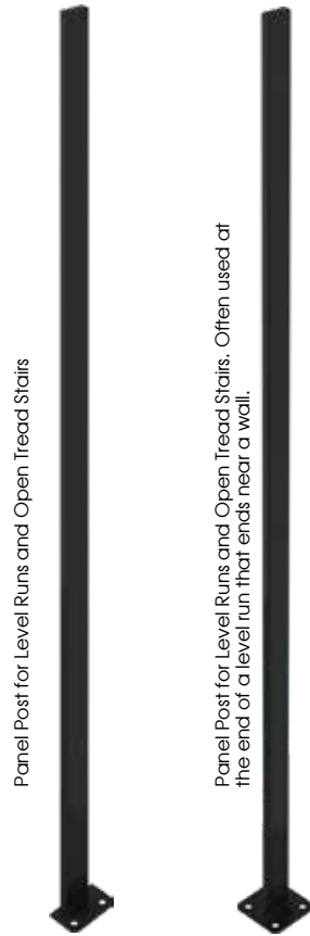
P-POST2H 2-Hole Foot Plate P-POST4H 4-Hole Foot Plate
