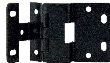
H760-45. Institutional Hinge 3/4" Overlay x 13/16" Door with 45mm CC on the Door Leaf CASE QTY 100 WEIGHT/CASE 46 lbs BOX QTY 10 Available Colors Item Number Black H760-45.BK Dull Chrome H760-45.DC
