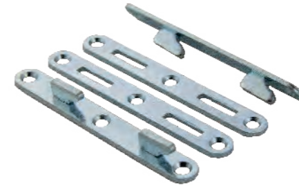
B850.NP Bed Rail Fastener 5" w/ Round Corners Zinc Plated CASE QTY 25 SETS WEIGHT/CASE 20 lbs
