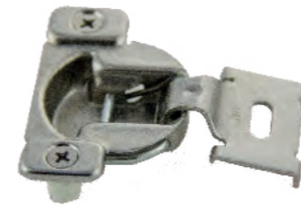
1 Pc Face Frame Hinge w/ Dowels H250-D 1/2" OL H254-D 3/4" OL
