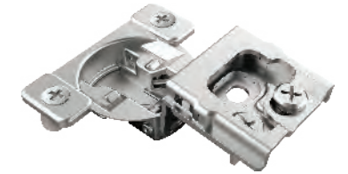
6 Way 3 Cam Adjustable 1 pc Face Frame Hinge 1-1/4" H292-D With Dowels
