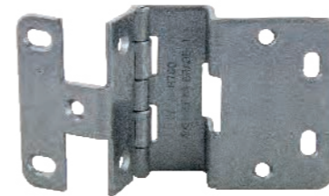
H780.DC Institutional Hinge 13/16" Overlay x 13/16" Door CASE QTY 100 WEIGHT/CASE 46 lbs BOX QTY 10 Available Colors Item Number Dull Chrome H780.DC
