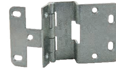
H760. Institutional Hinge 3/4" Overlay x 13/16" Door CASE QTY 100 WEIGHT/CASE 46 lbs BOX QTY 10 Available Colors Item Number Dull Chrome H760.DC Powder Dull Chrome H760.PDC
