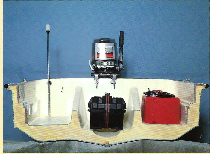
FULLY FOAMED CONSTRUCTION
