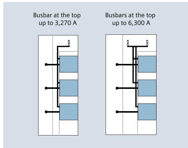
Fig. 3/6: Cubicle types with three circuit-breakers (side view)
