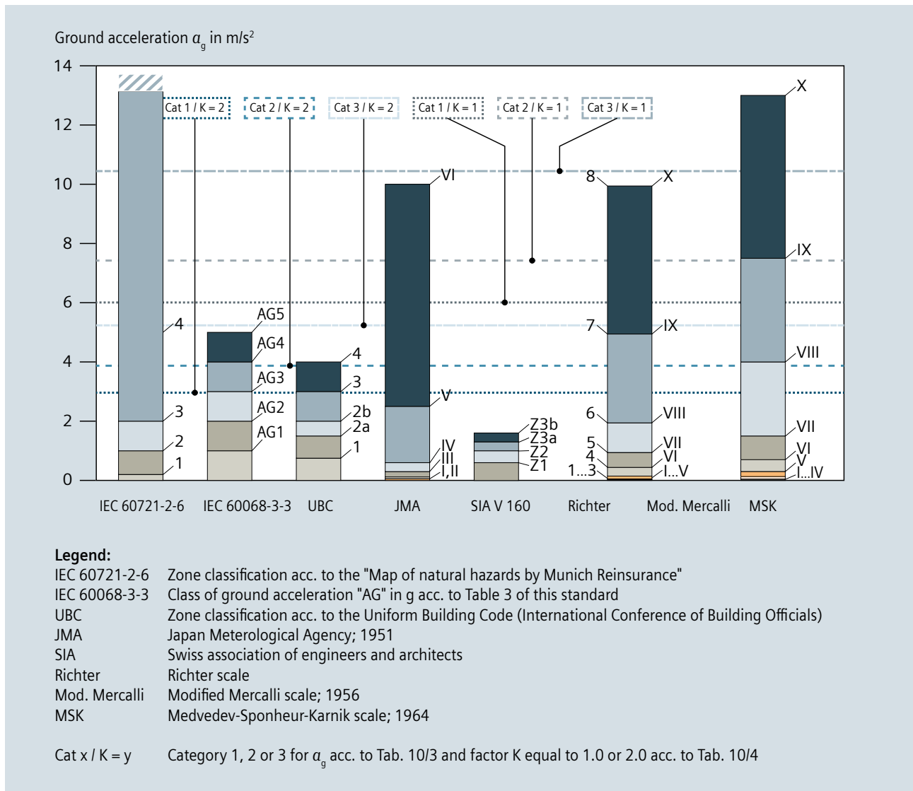
Fig. 10/7: Comparison of seismic scales for the classification of seismic response categories of SIVACON S8
