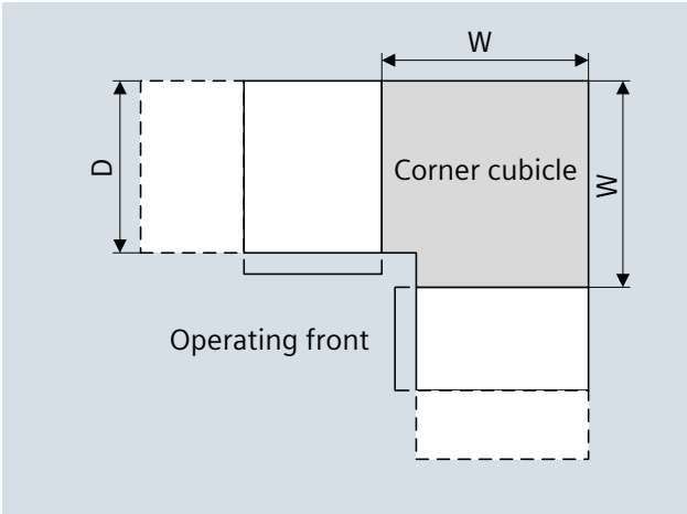
Fig. 2/3: Integration of a corner cubicle
