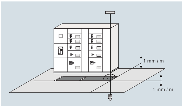
Fig. 9/5: Permissible deviations in the installation area
