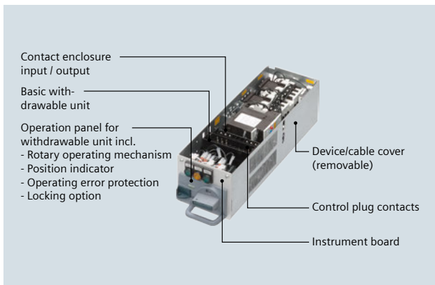
Fig. 4/6: Structure of a small withdrawable unit in HFD
