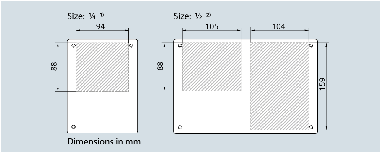
Fig. 4/9: Front areas usable for an instrument board for small withdrawable units with a mounting height of 200 mm for 1) 2) and 300 mm for 1)
