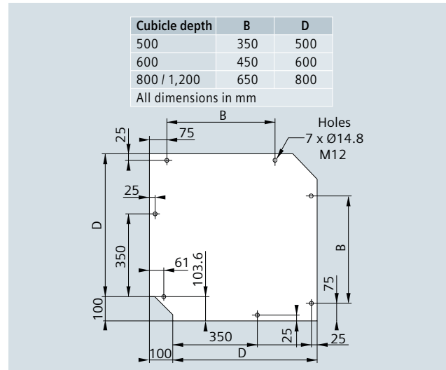
Fig. 9/9: Fixing points for the corner cubicle
