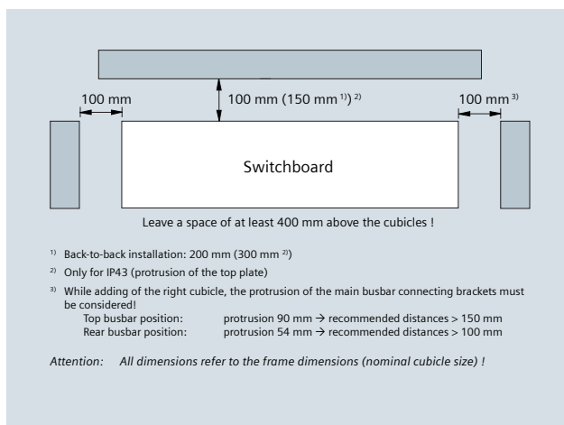
Fig. 9/1: Distances to obstacles
