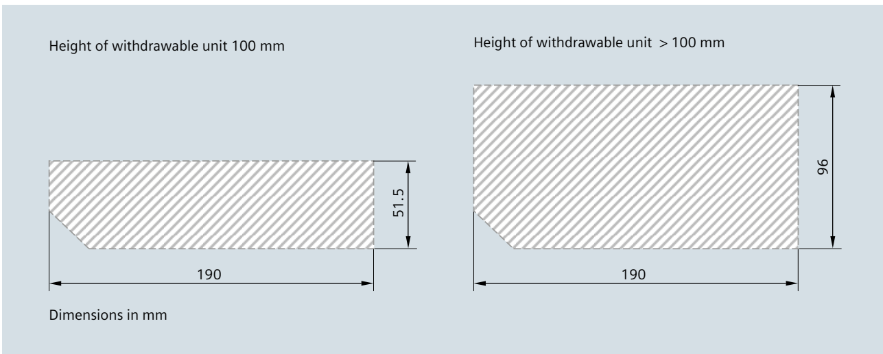
Fig. 4/10: Front areas usable for an instrument board for normal withdrawable units
