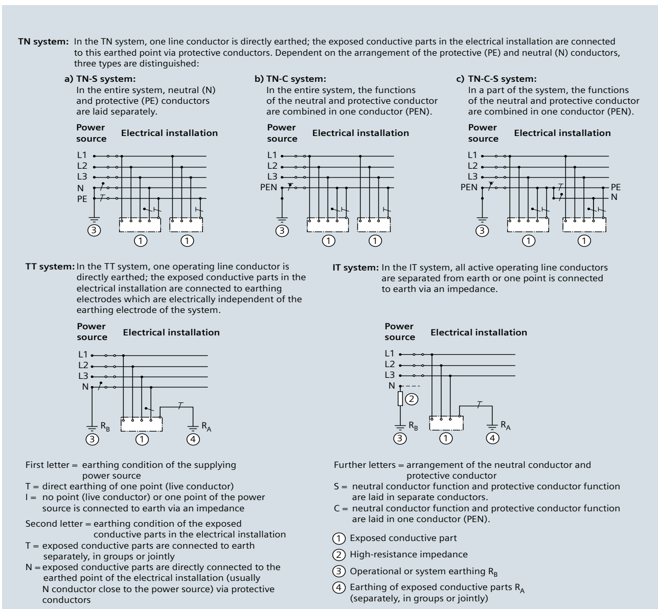
Fig. 11/1: Systems by type of connection to earth in accordance with IEC 60364-1
