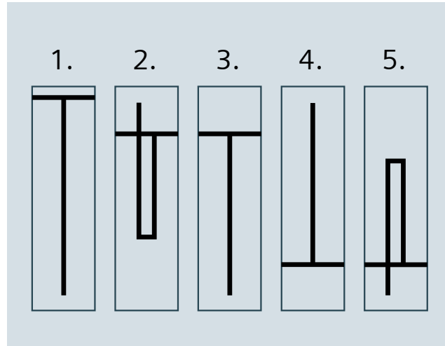
Fig. 3/7: Cubicle types for direct incoming feeder / direct outgoing feeder (refer to the text for explanations)
