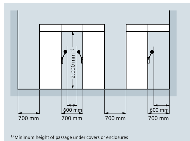
Fig. 9/2: Gangway widths and passage heights
