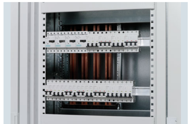
Fig. 6/5: Assembly kit for modular installation devices (without cover)
