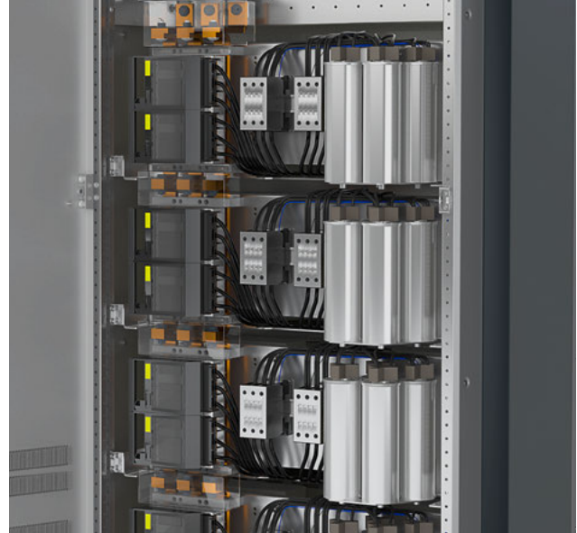
Fig. 7/2: Capacitor assemblies of the reactive power compensation
