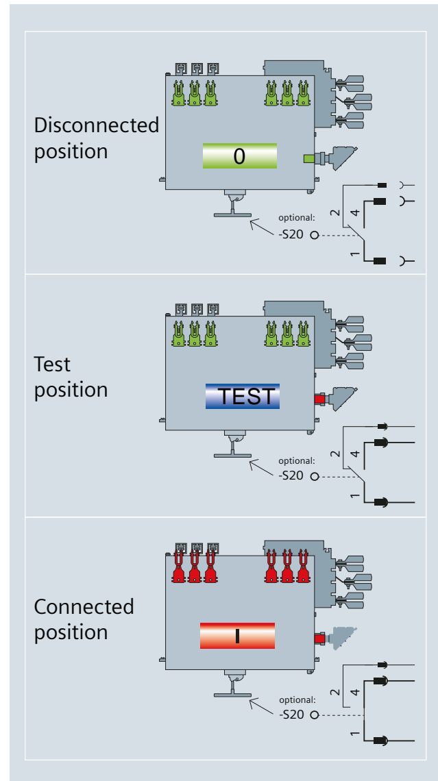
Fig. 4/7: Positions with disconnecting contact system in HFD
