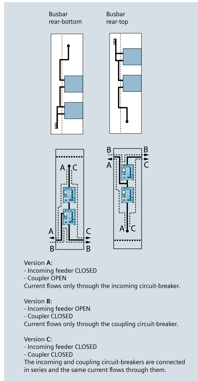
Fig. 3/3: Cubicle types and load cases with two 3WA12 as longitudinal coupler and incoming feeder / outgoing feeder (top: side view; bottom: front view)
