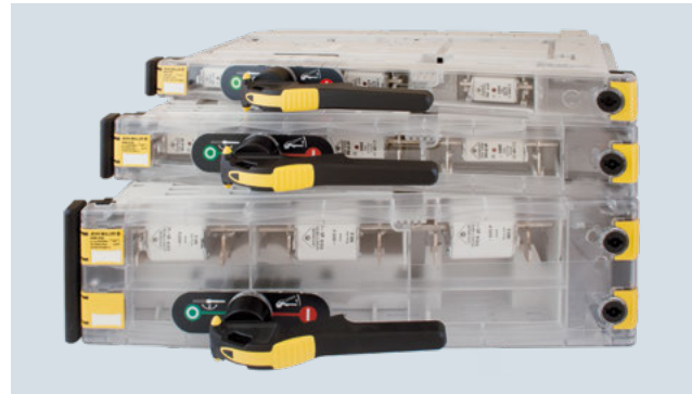
Fig. 5/3: Plug-in in-line switch-disconnectors SASILplus
