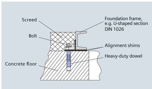
Fig. 9/7: Foundation frame fixing on concrete
