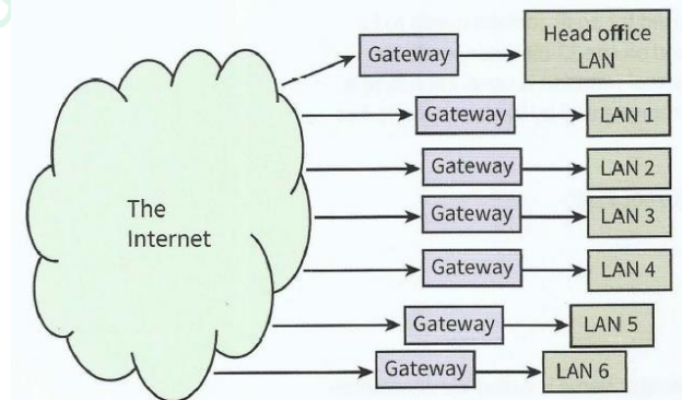
Figure 2.07 Connecting LANs using the original classful IPv4 scheme
