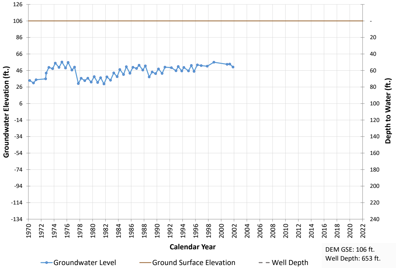
Well 752 Hydrograph
