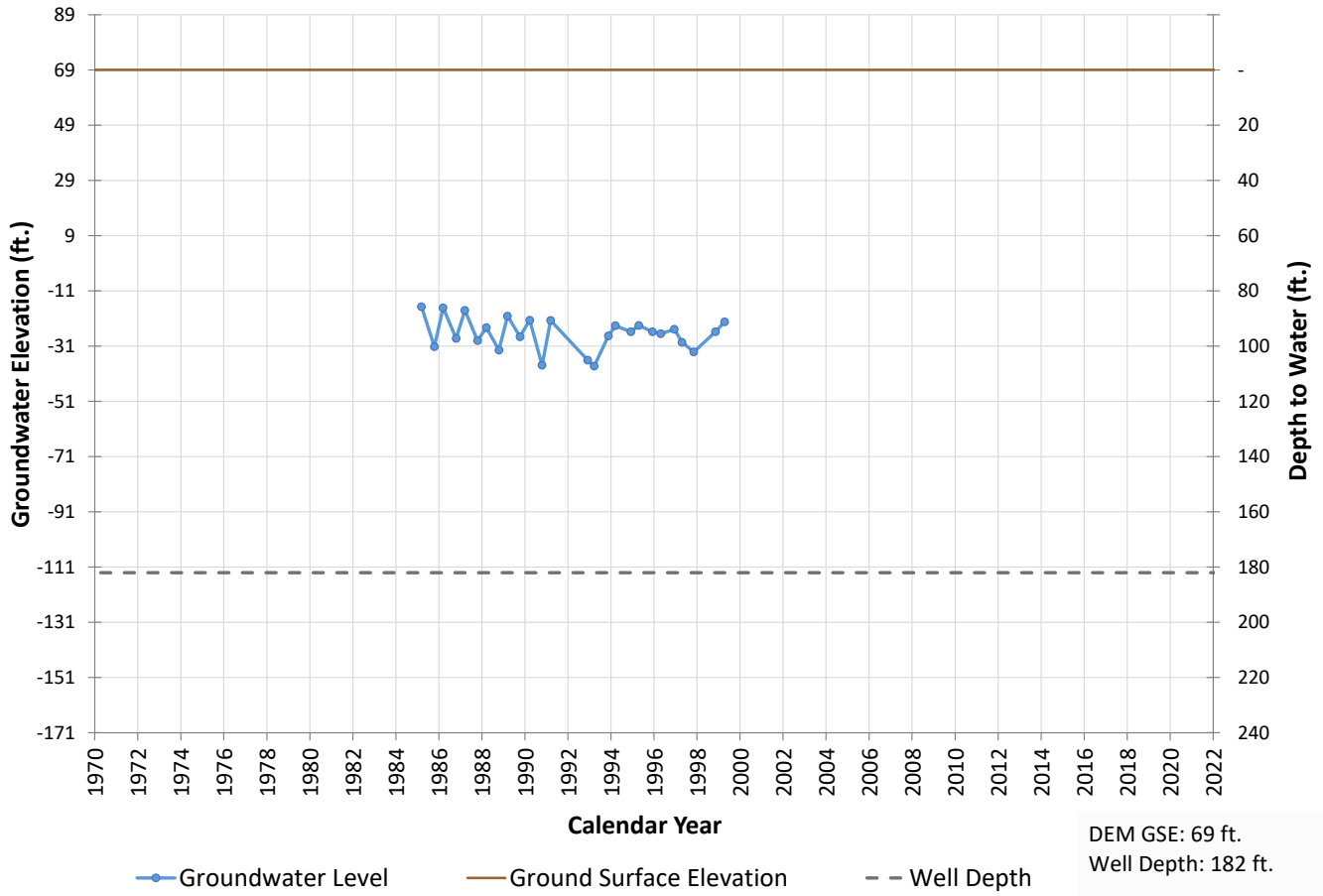
Well 267 Hydrograph
