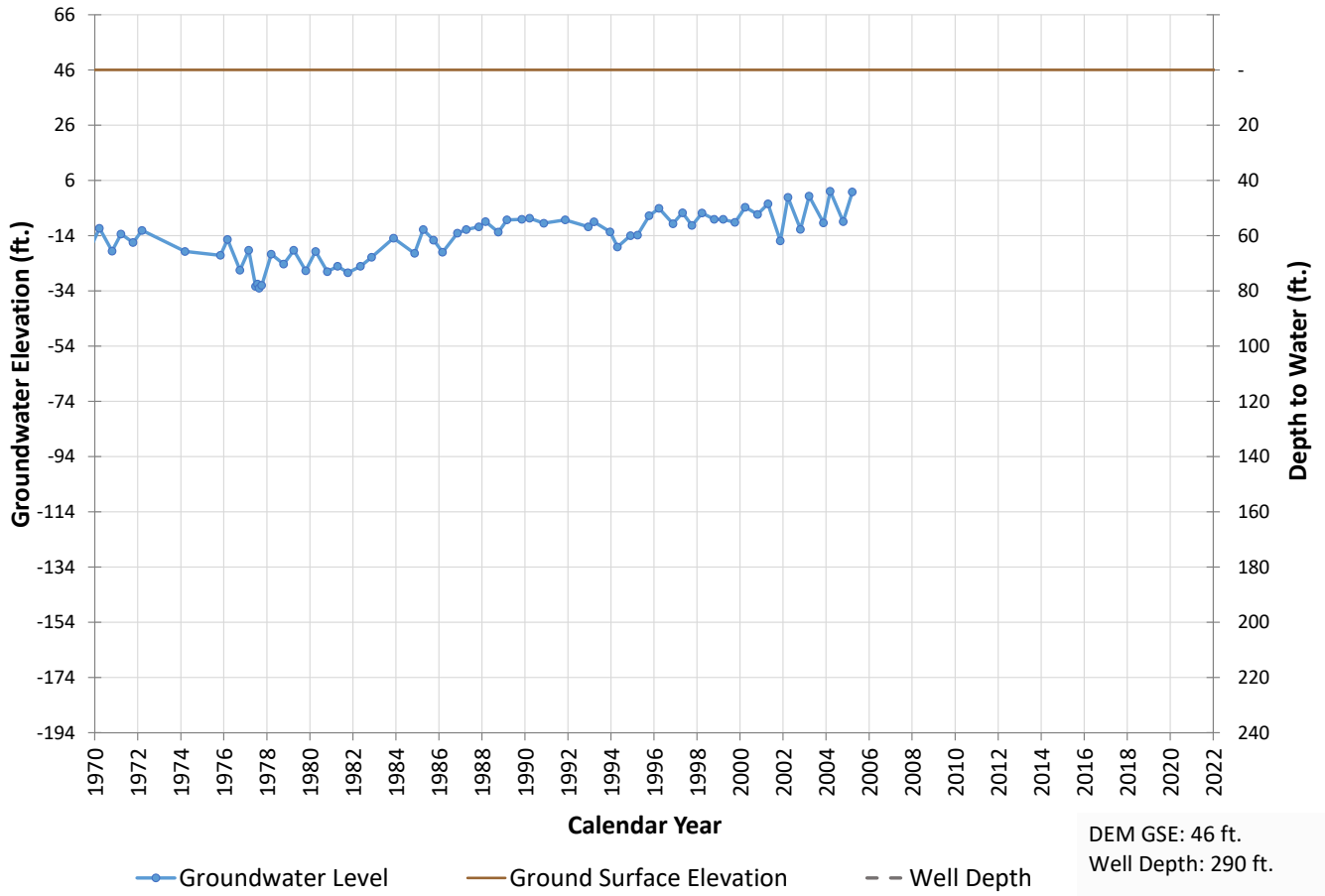
Well 538 Hydrograph
