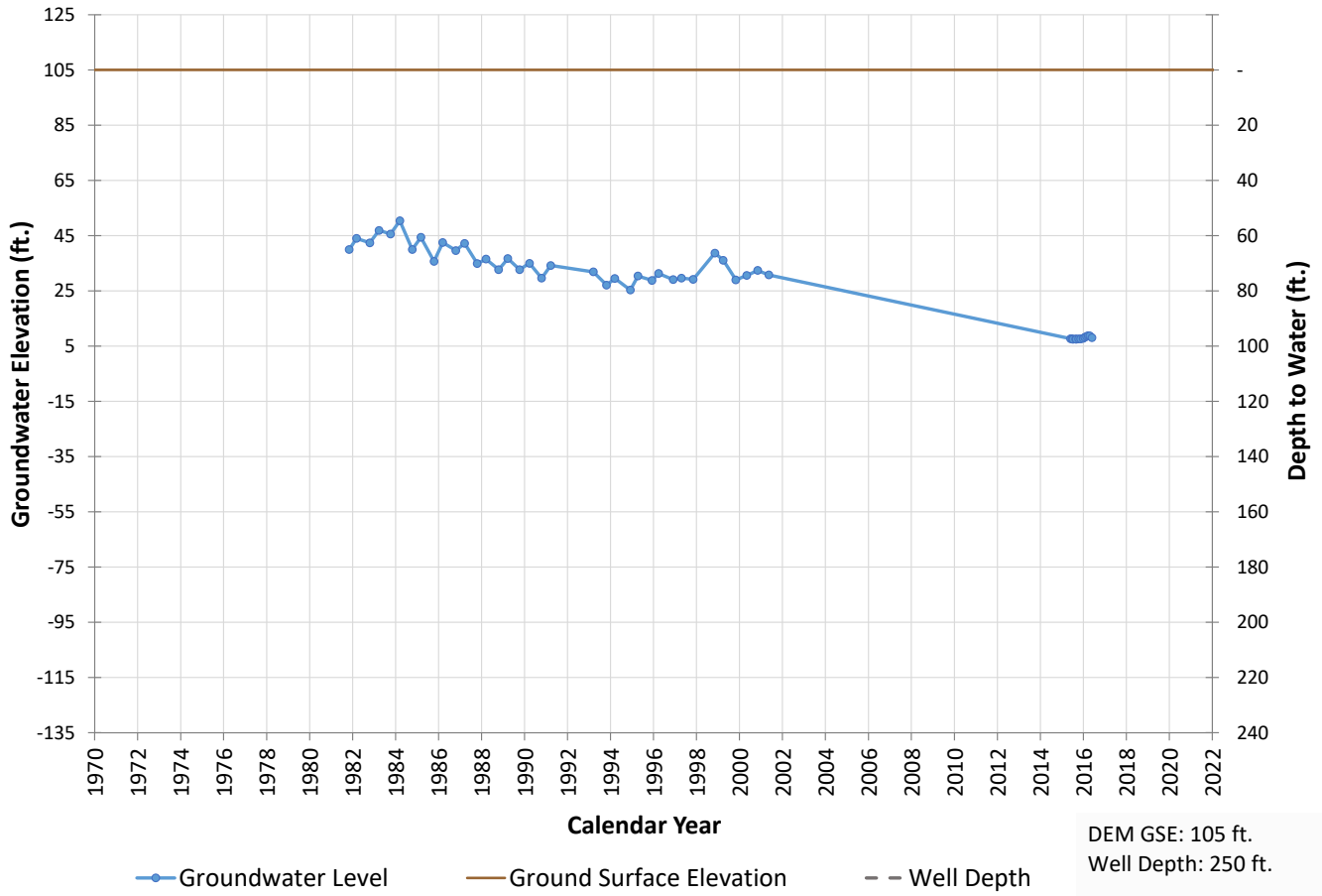
Well 357 Hydrograph
