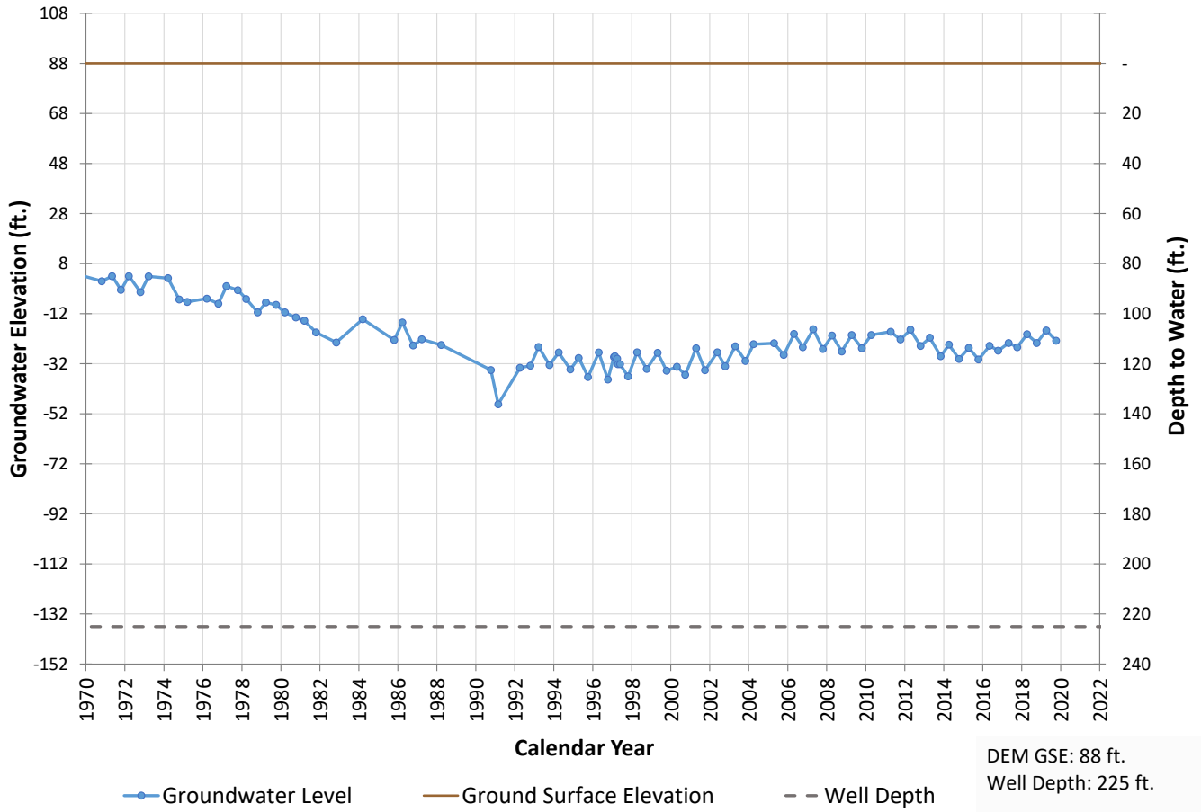
Well 489 Hydrograph
