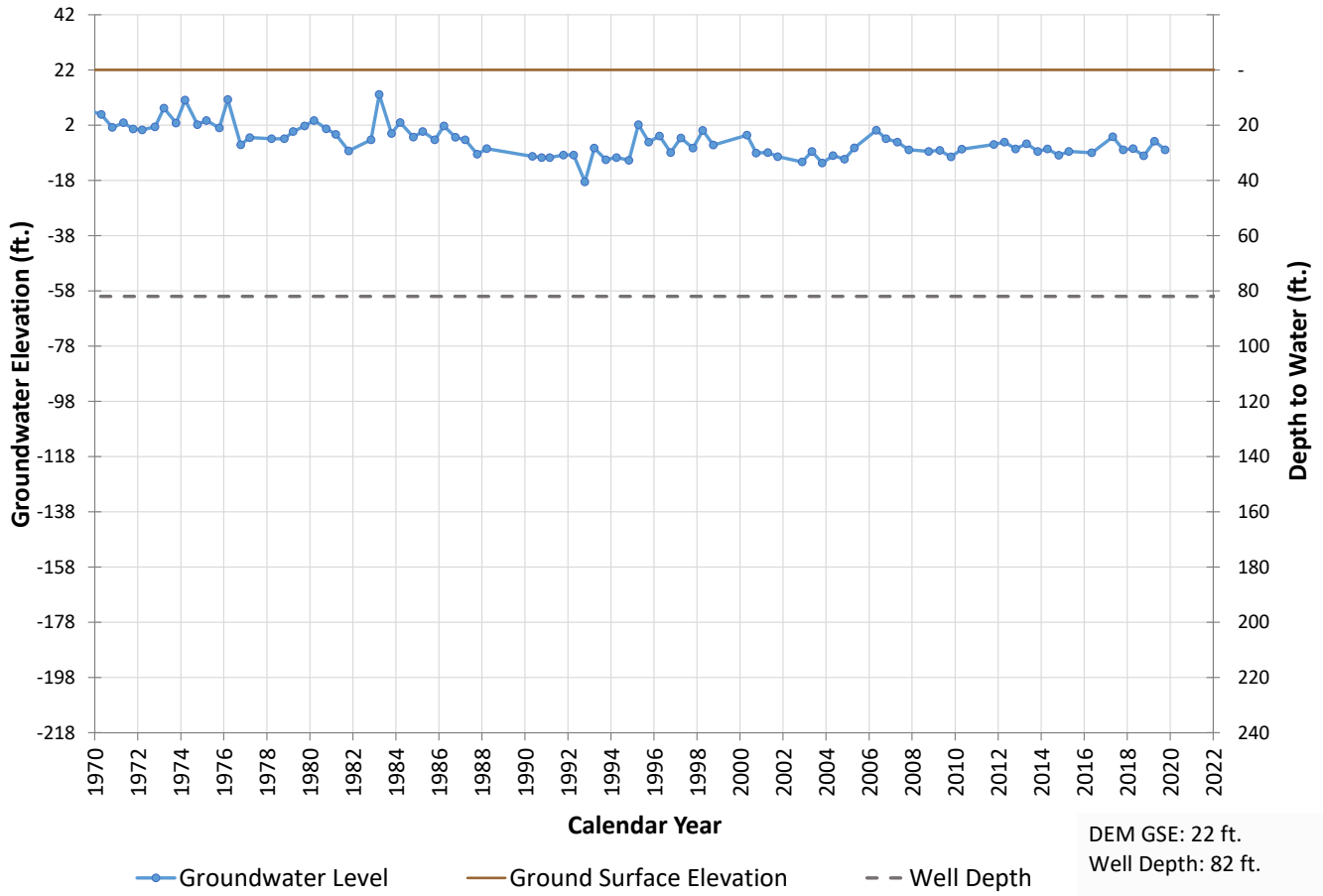
Well 447 Hydrograph
