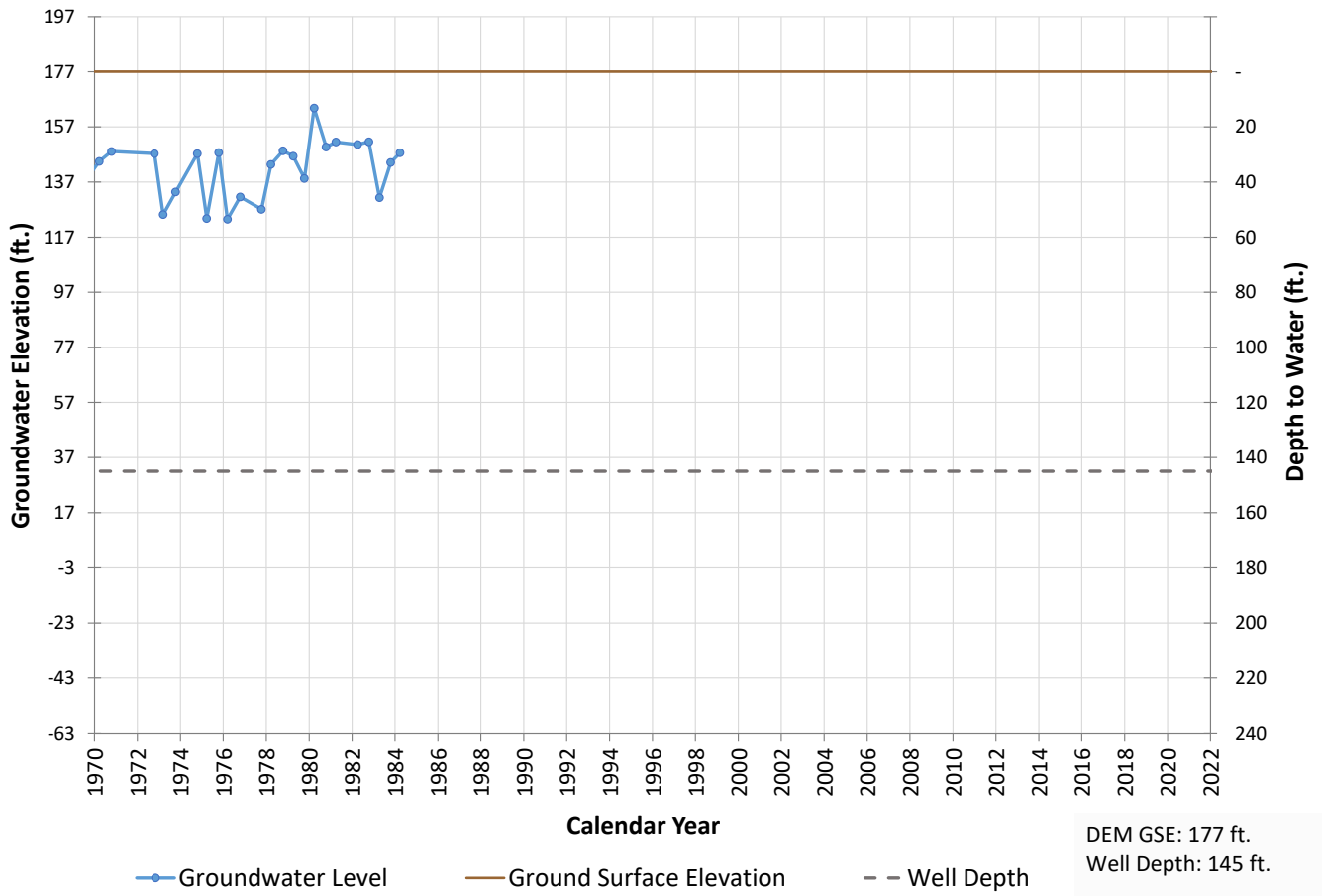
Well 774 Hydrograph
