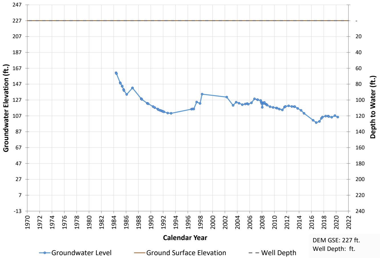
Well 867 Hydrograph
