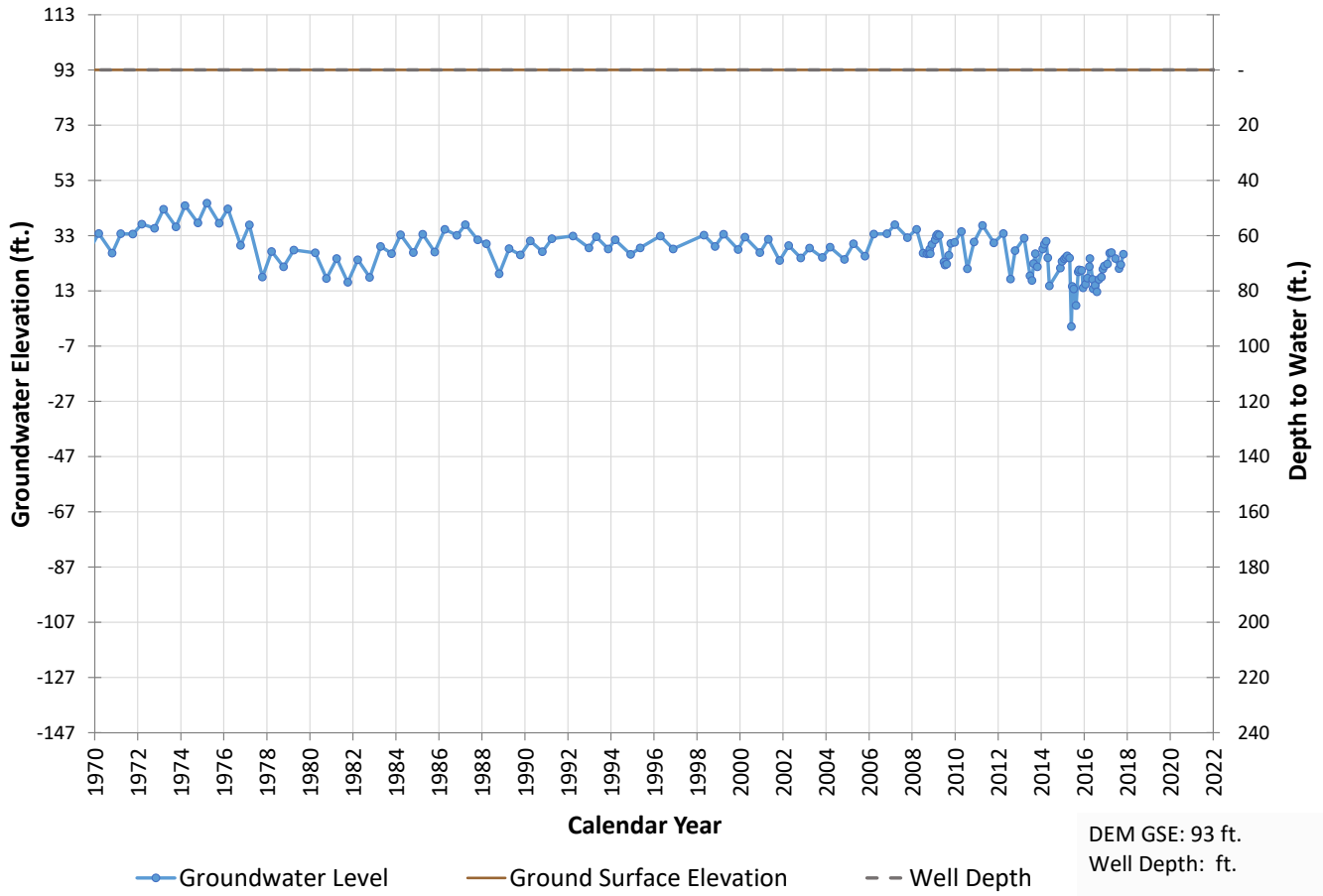
Well 731 Hydrograph
