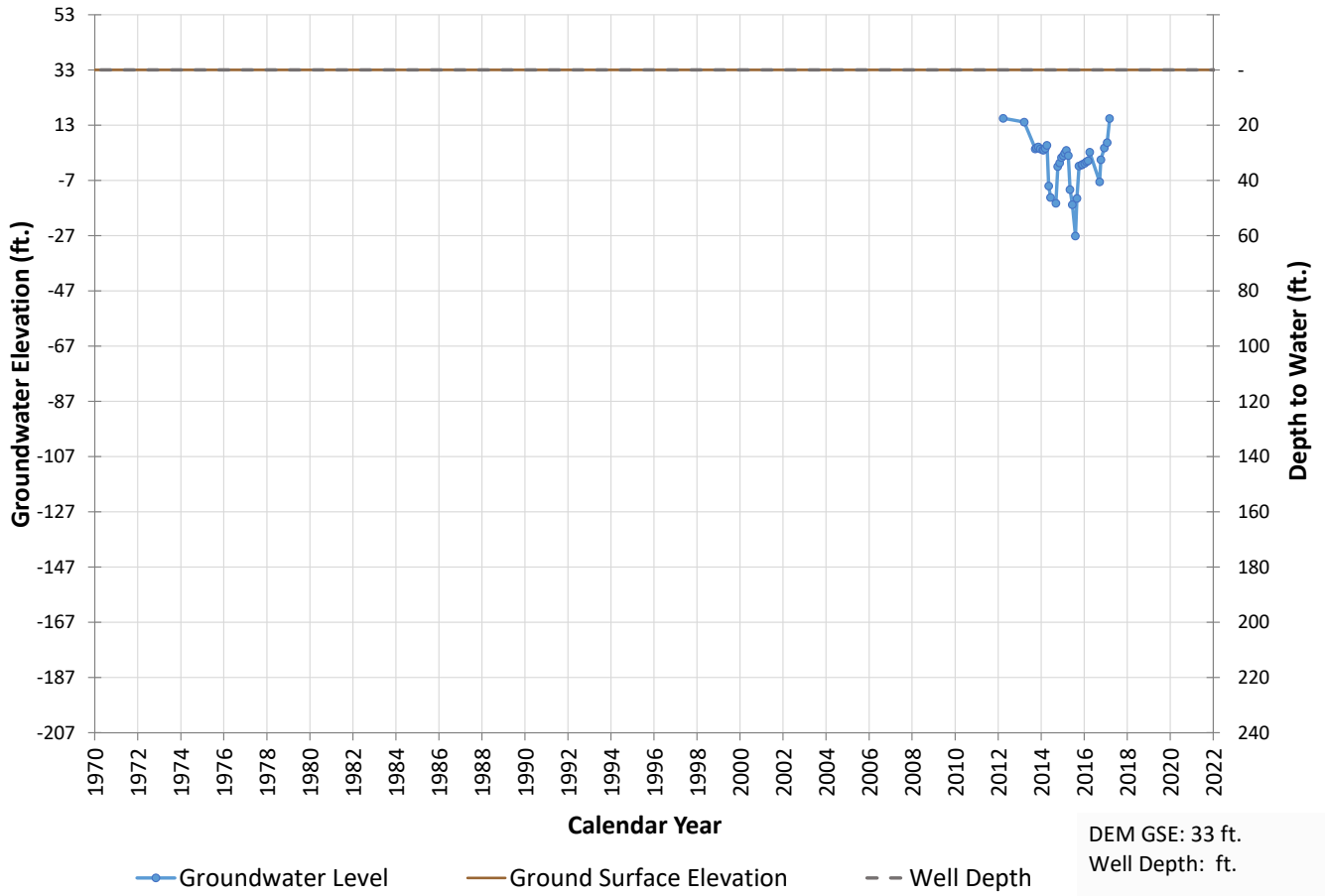
Well 655 Hydrograph
