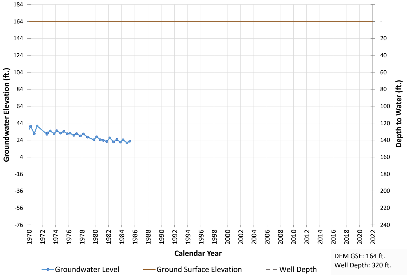
Well 582 Hydrograph
