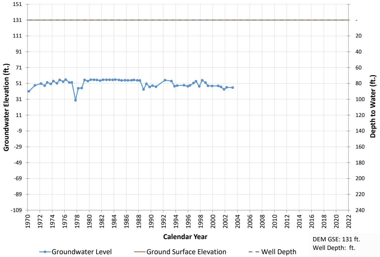
Well 743 Hydrograph
