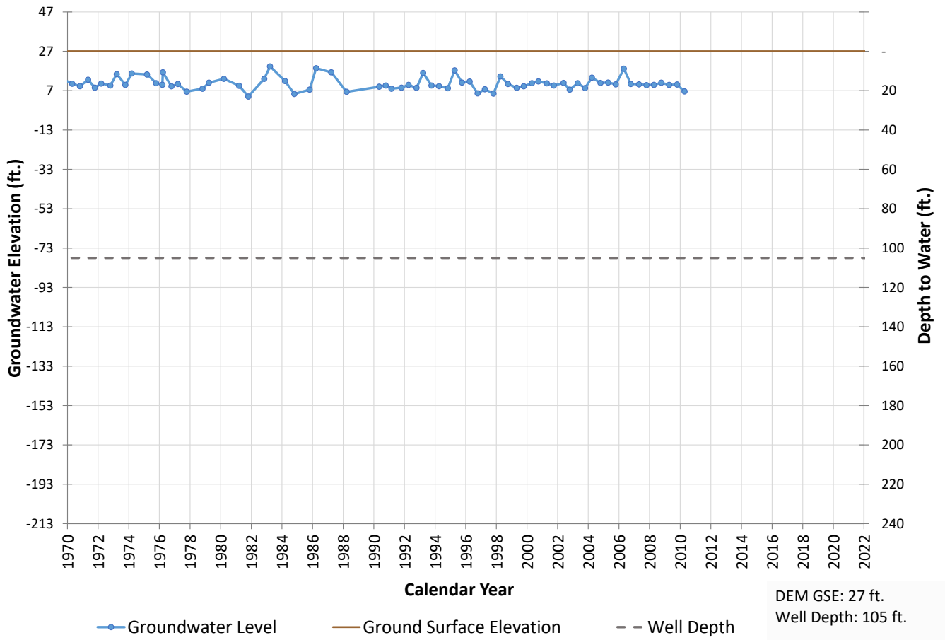
Well 438 Hydrograph
