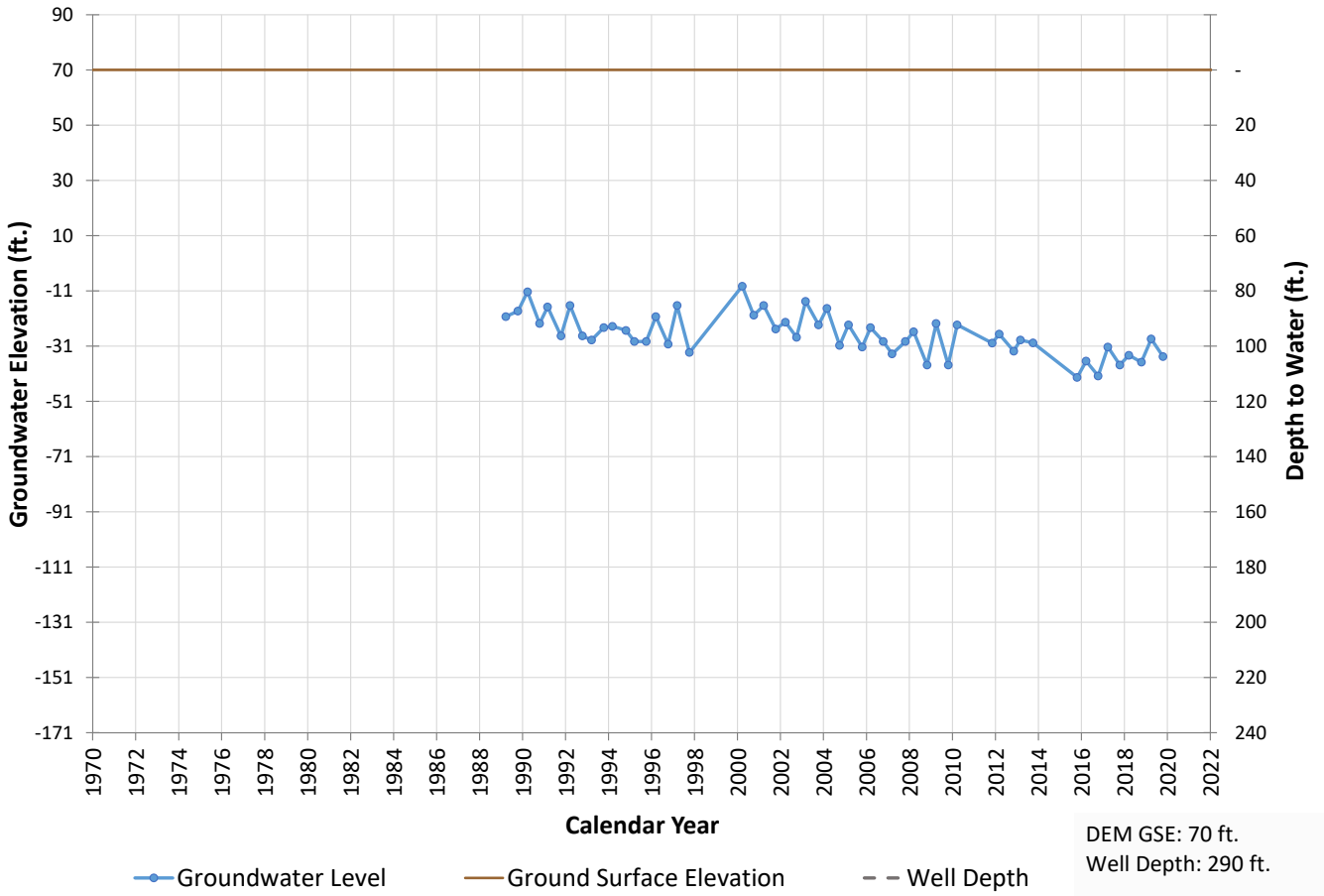
Well 13 Hydrograph
