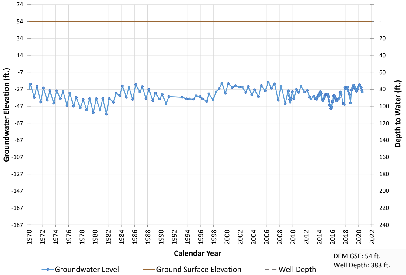
Well 69 Hydrograph
