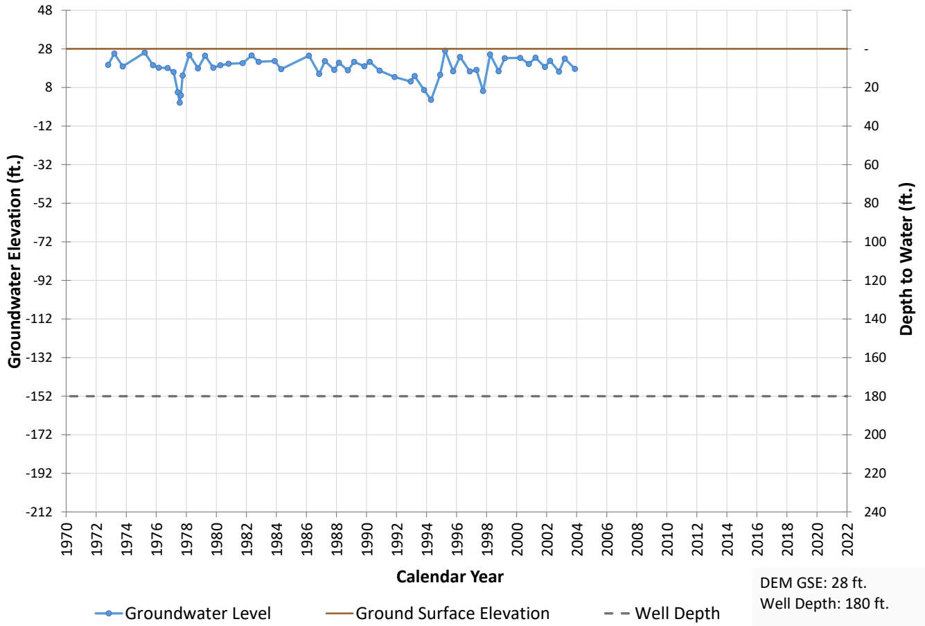
Well 718 Hydrograph
