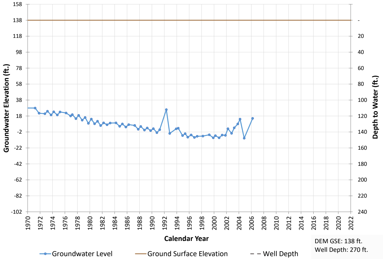
Well 554 Hydrograph
