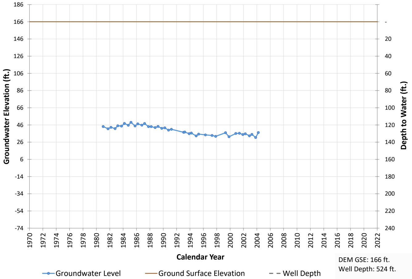
Well 277 Hydrograph
