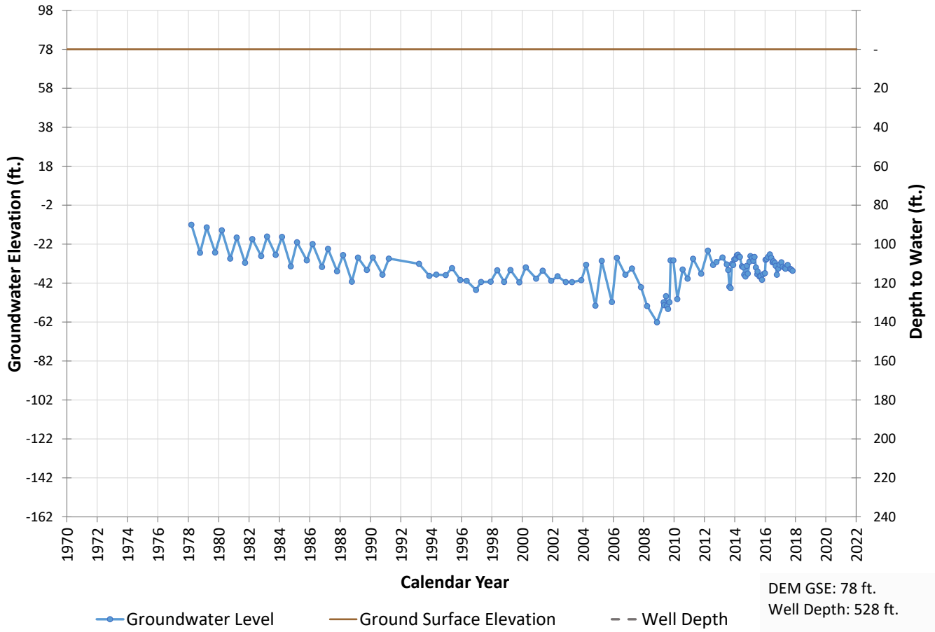
Well 431 Hydrograph
