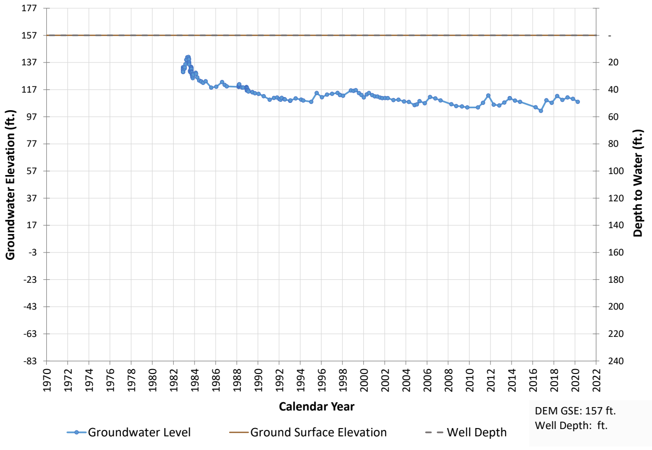
Well 859 Hydrograph
