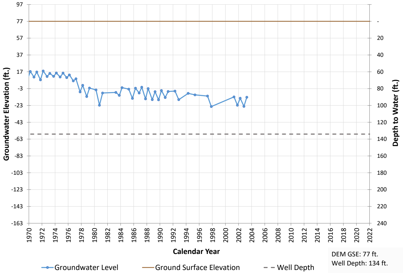
Well 640 Hydrograph
