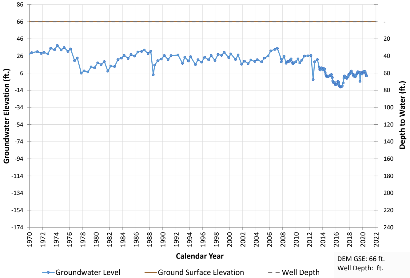
Well 735 Hydrograph
