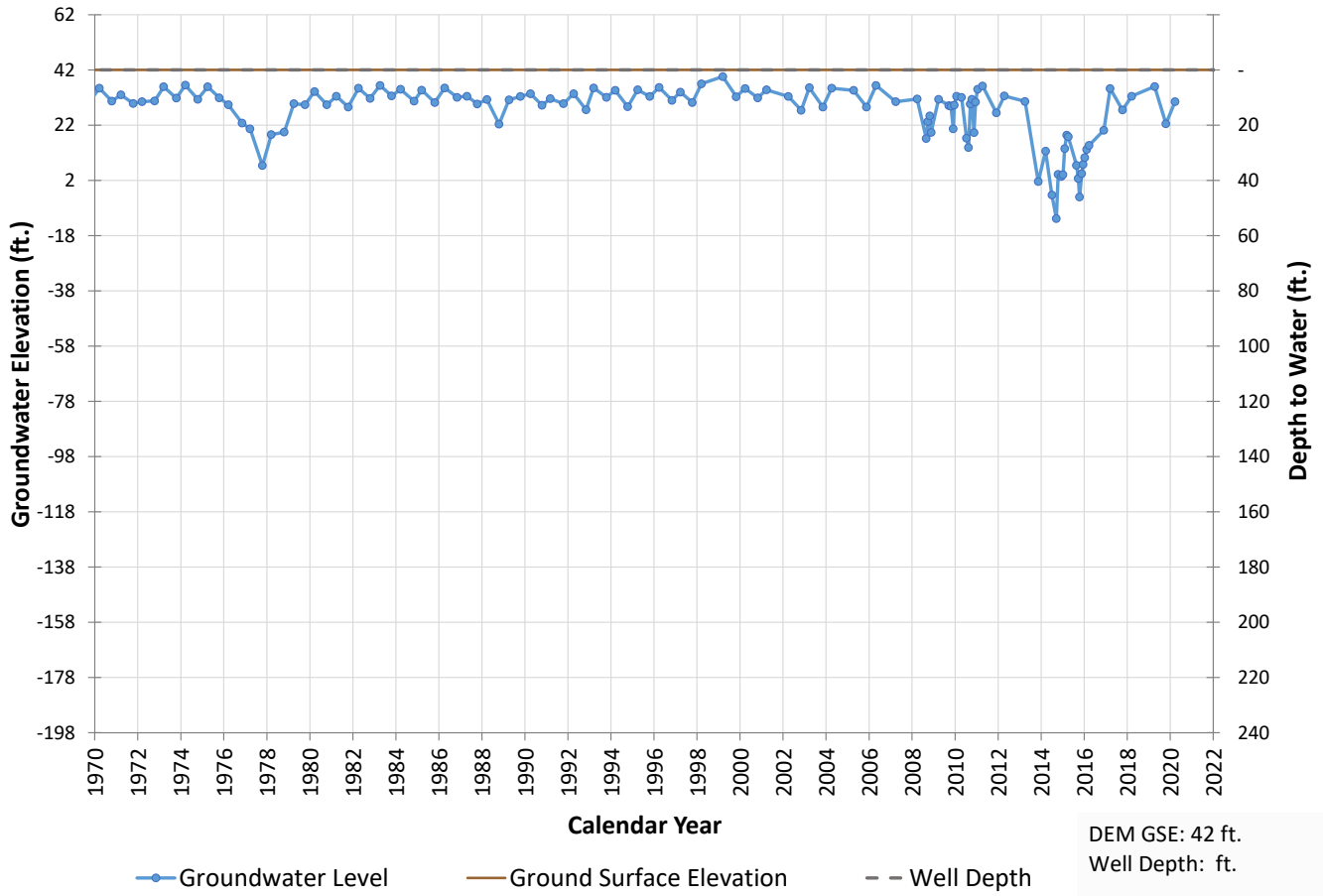
Well 763 Hydrograph
