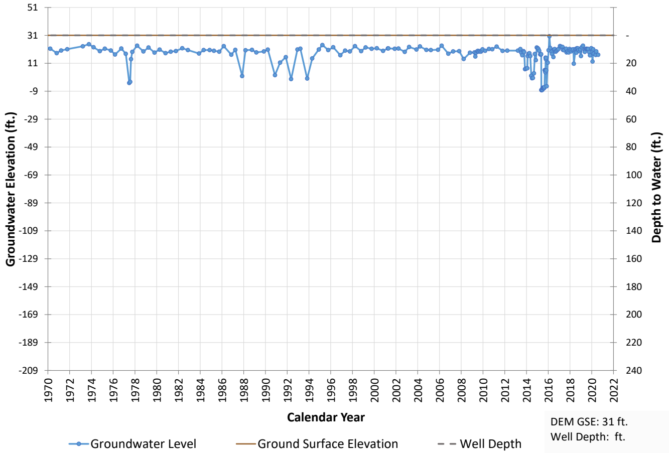
Well 602 Hydrograph
