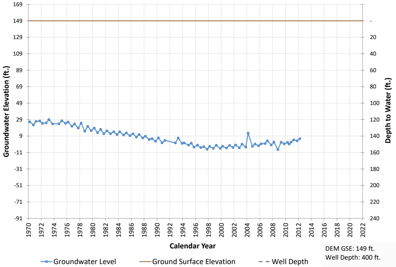
Well 544 Hydrograph
