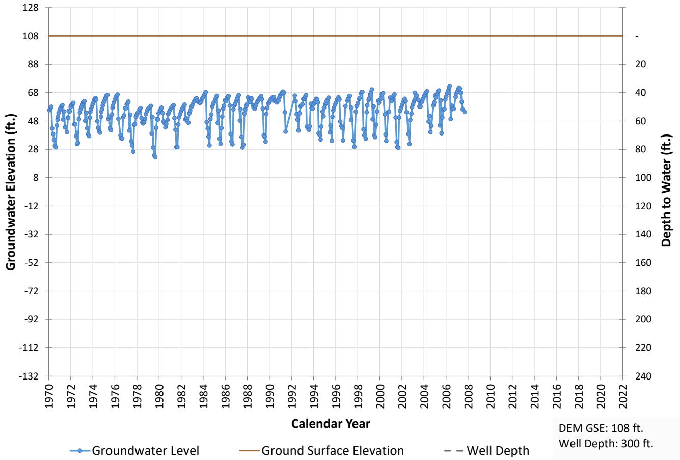
Well 771 Hydrograph
