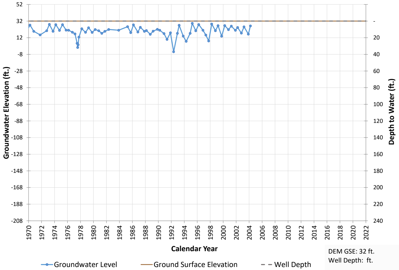
Well 734 Hydrograph
