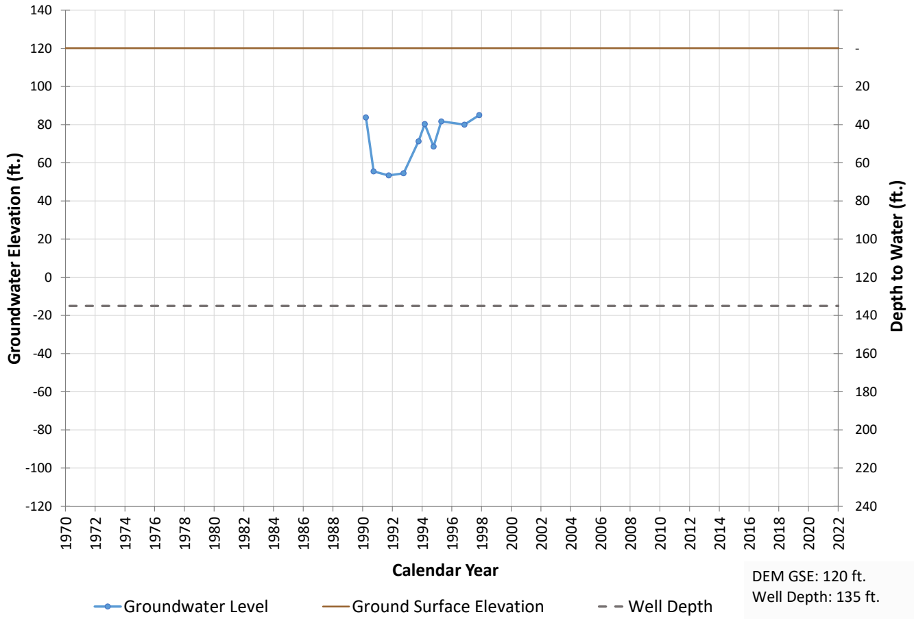
Well 247 Hydrograph
