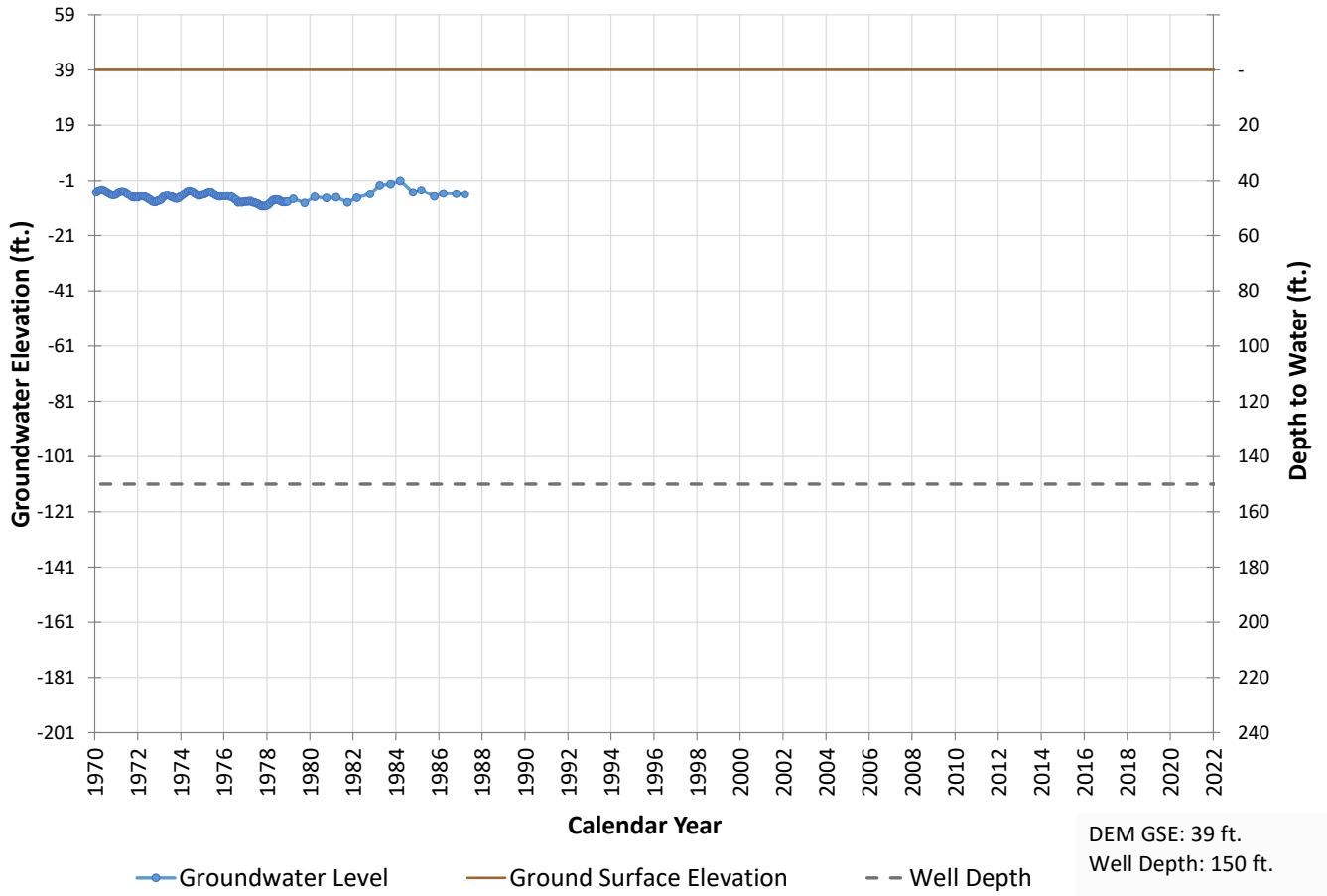
Well 285 Hydrograph
