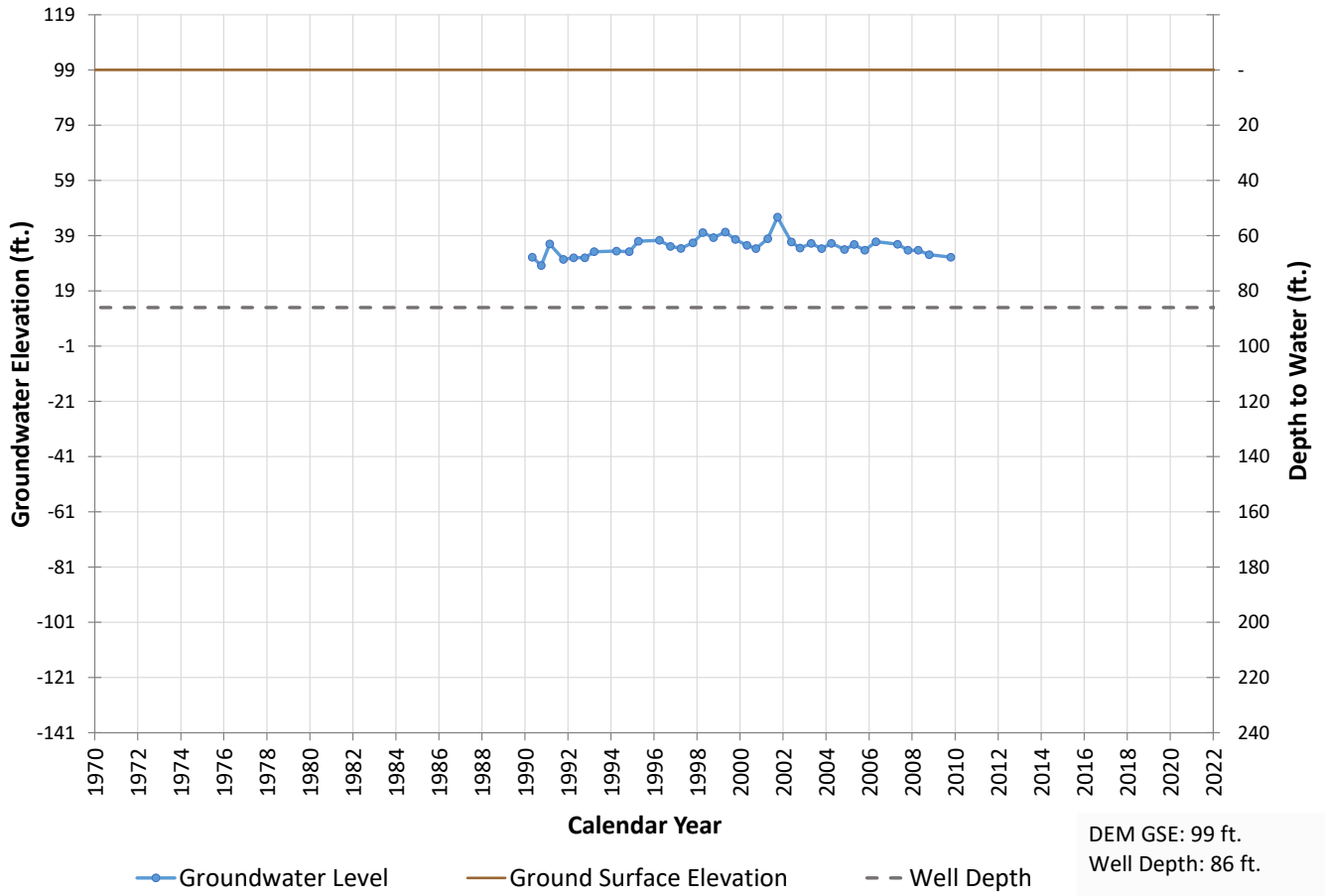
Well 361 Hydrograph
