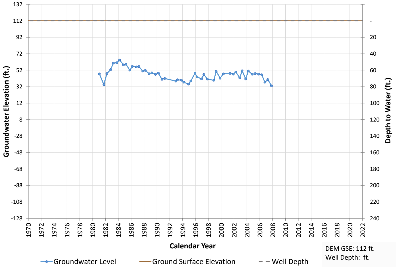
Well 331 Hydrograph
