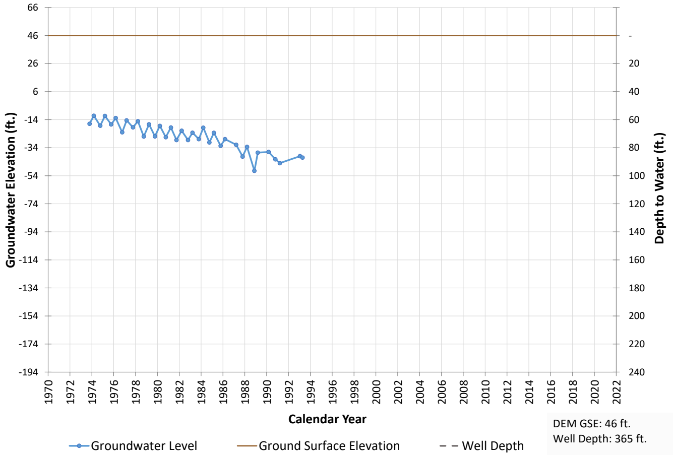
Well 412 Hydrograph
