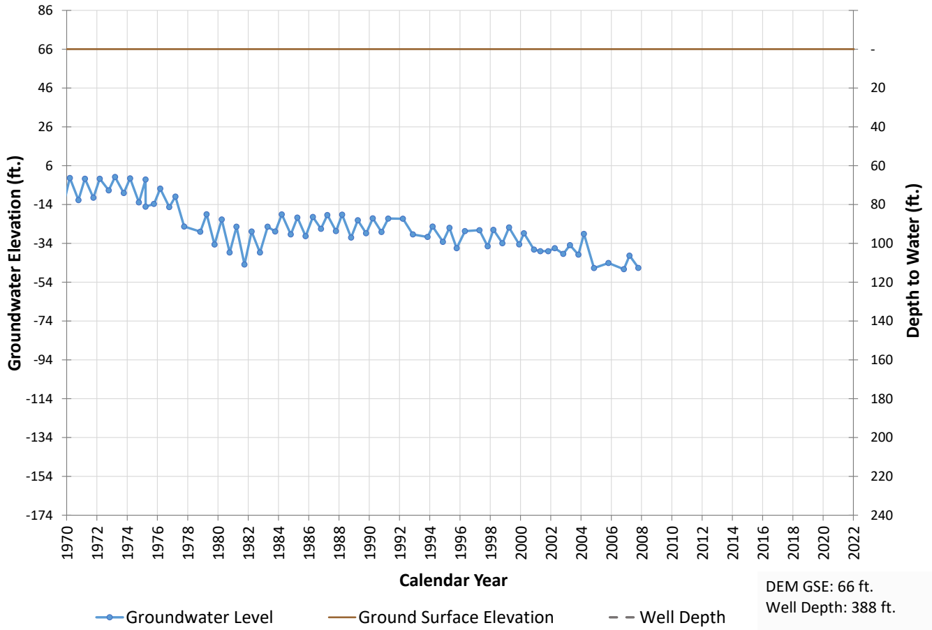
Well 586 Hydrograph
