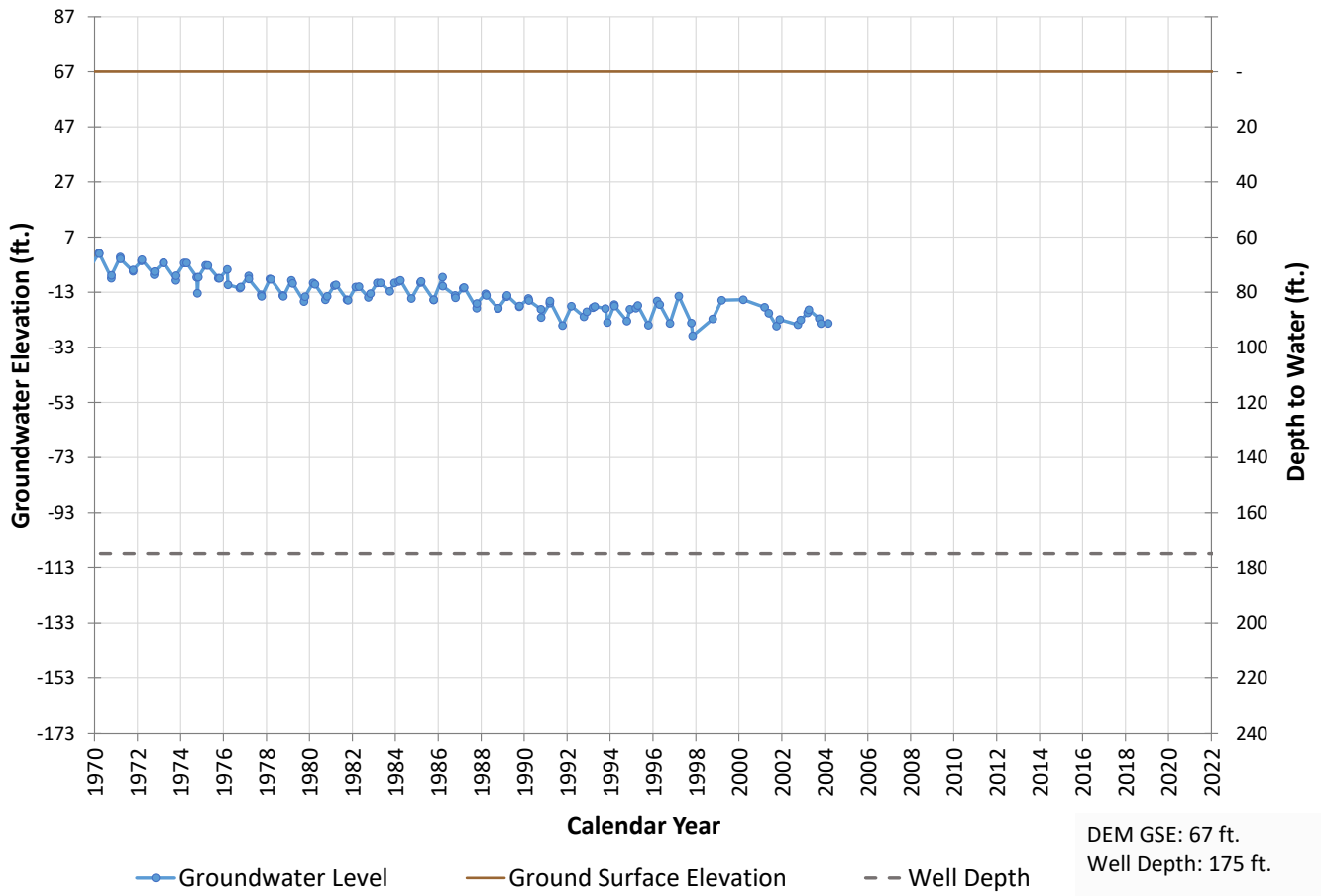
Well 275 Hydrograph
