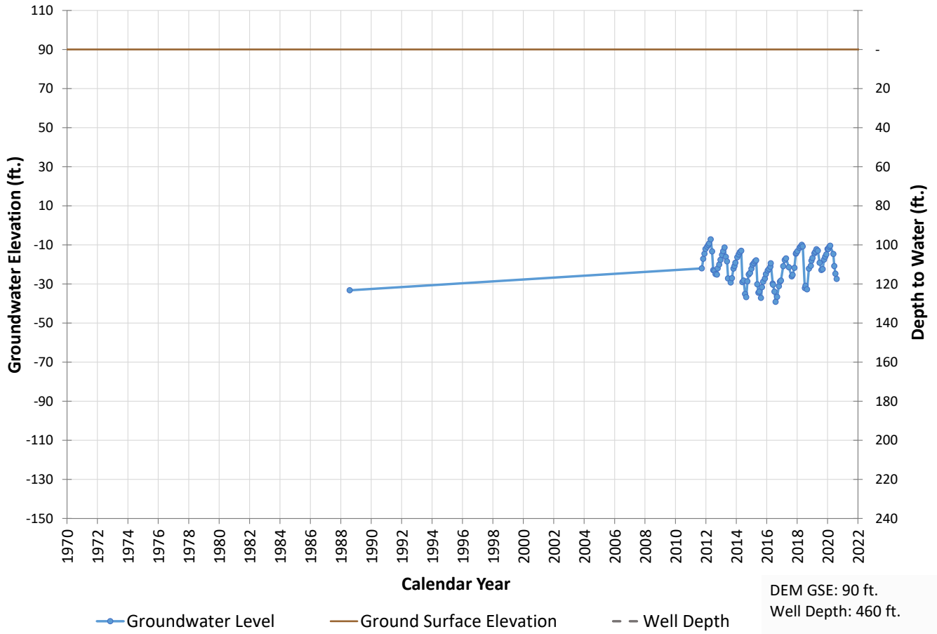
Well 639 Hydrograph
