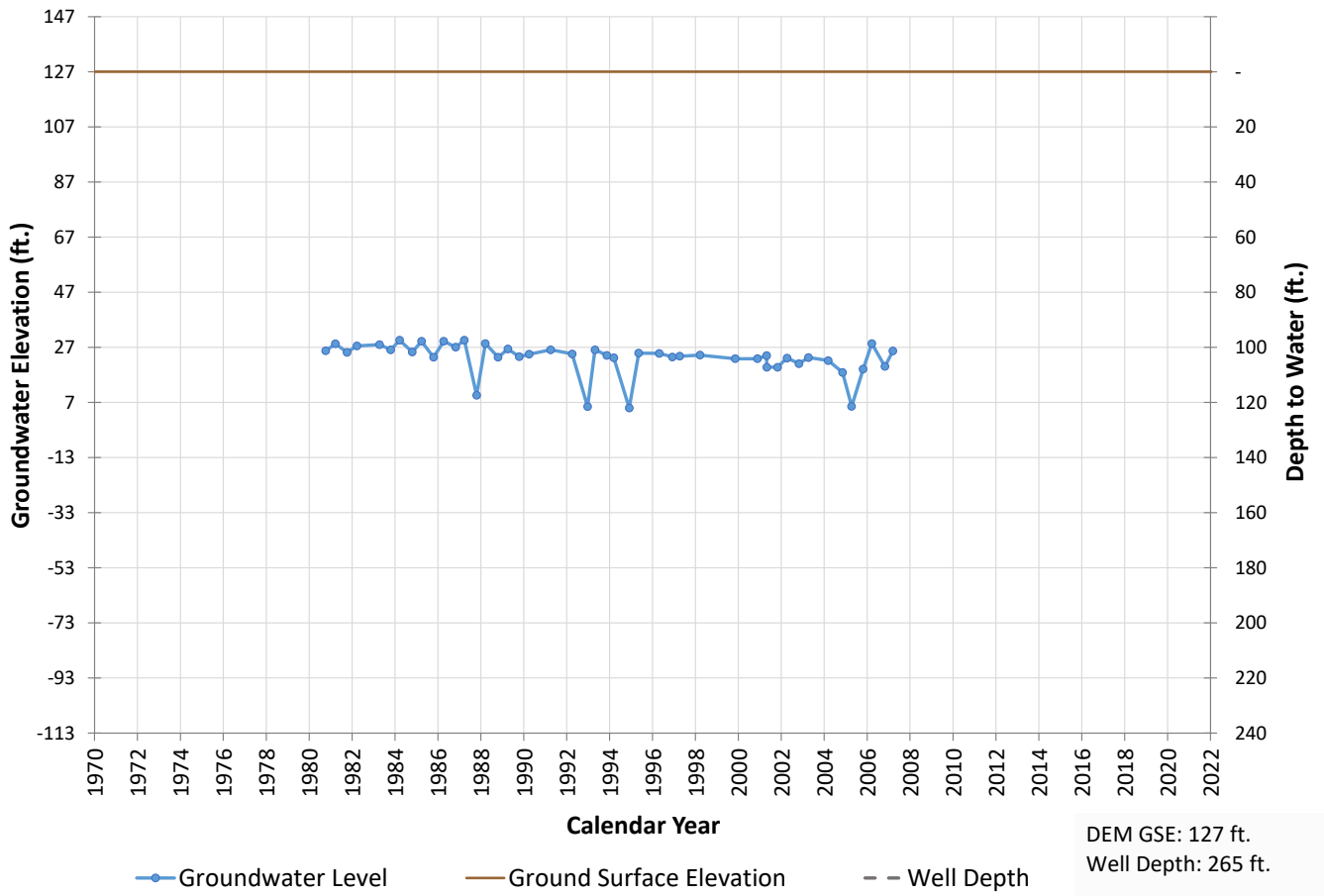
Well 701 Hydrograph
