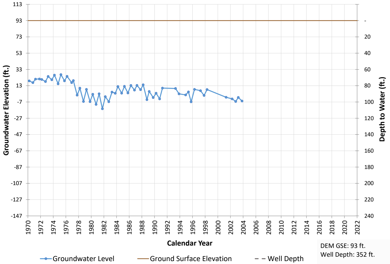
Well 713 Hydrograph
