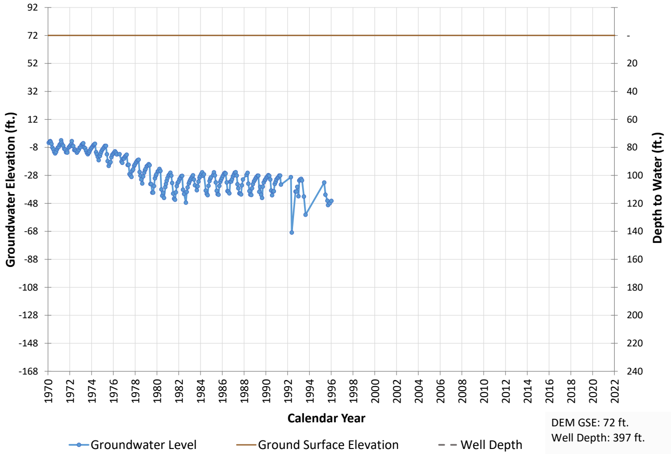
Well 568 Hydrograph
