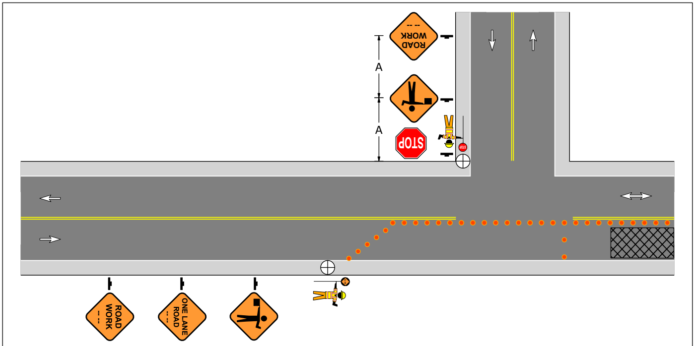
Figure 6-18 Intersection within the Activity Area
