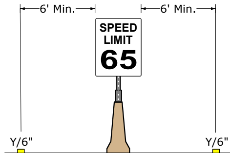
Figure 10-64 Adjacent to Barrier
