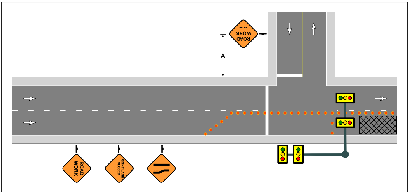
Figure 6-57 Intersection within the Activity Area
