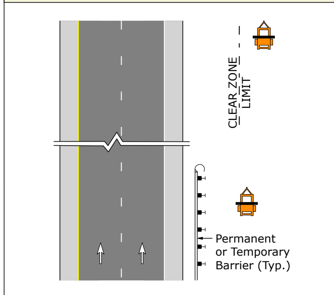
Figure 9-3 Trailer Outside Clear Zone or Behind Barrier Delineation is Not Required
