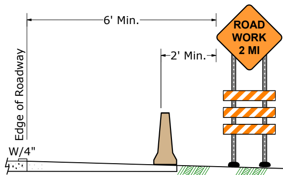
Figure 10-58 Adjacent to Barrier
