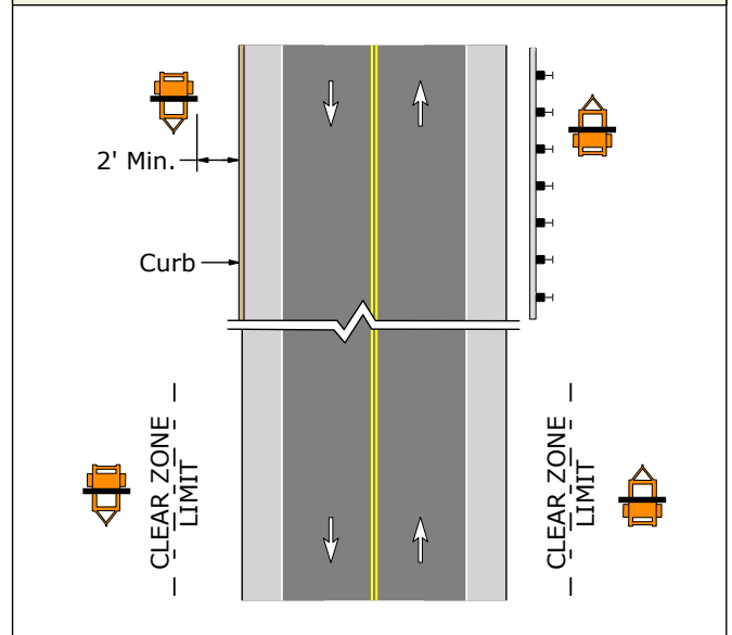
Figure 9-5 Trailer Outside Clear Zone or Behind Barrier Delineation is Not Required
