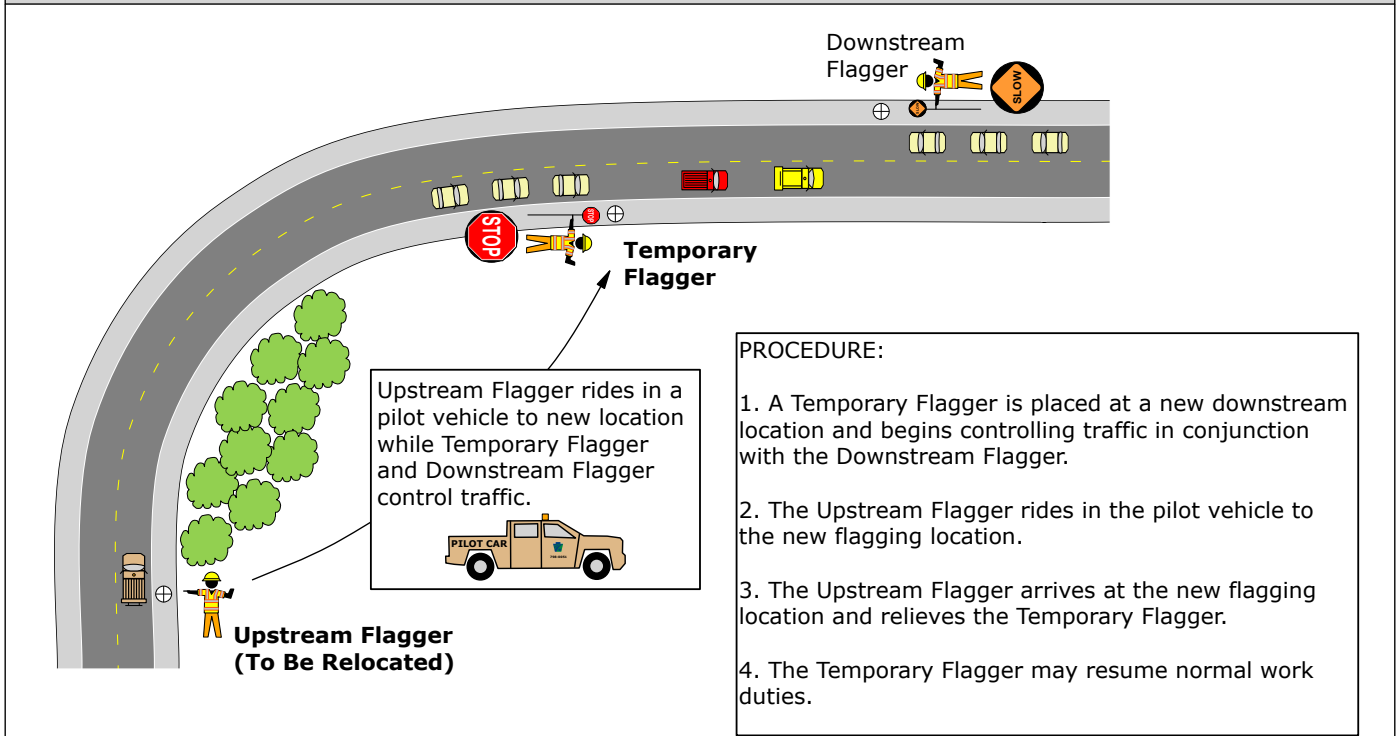
Figure 302-12 Temporary Flagger Utilized
