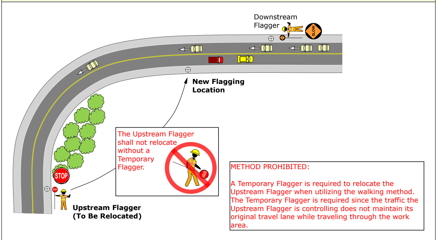
Figure 302-5 No Temporary Flagger Utilized
