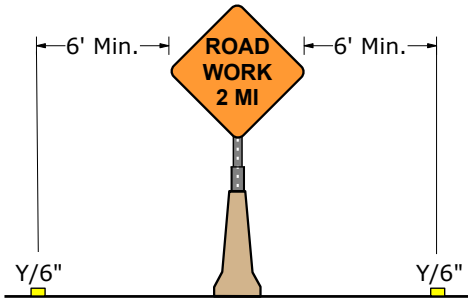
Figure 10-63 Not Adjacent to Barrier
