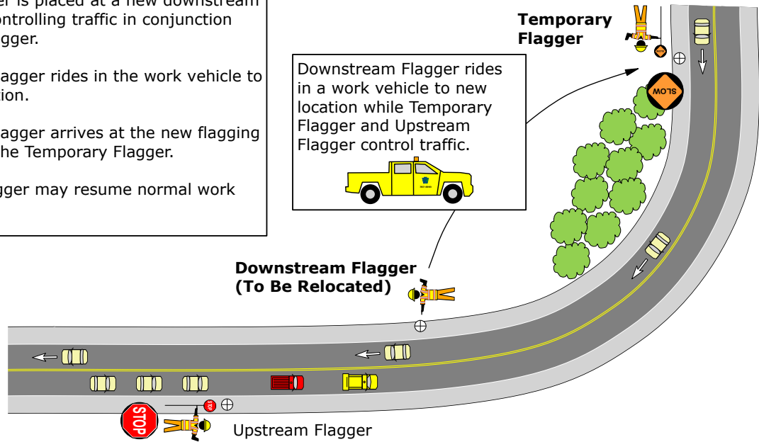
Figure 302-6 Temporary Flagger Utilized
