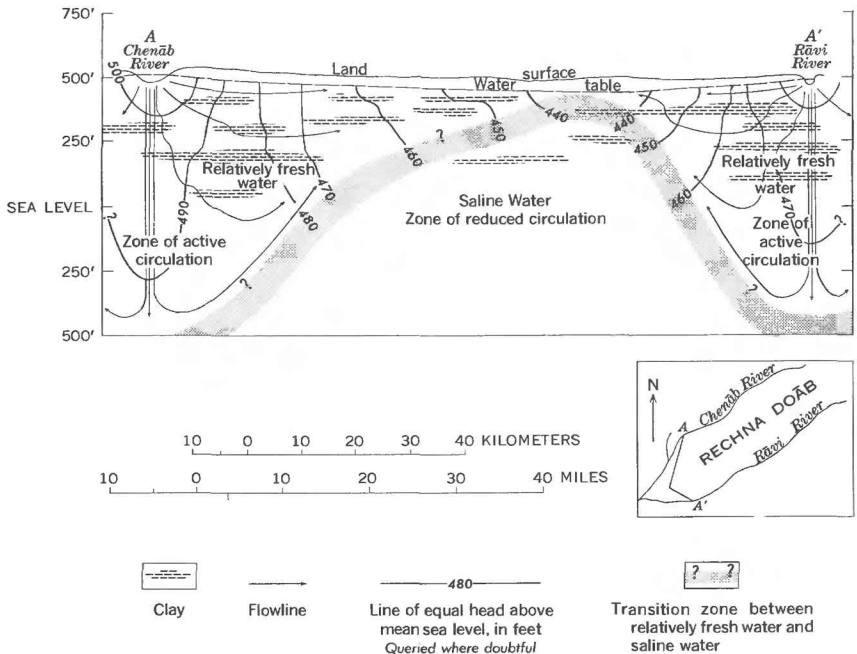
FIGURE 3.—Hydraulic profile for Rechna Doab for preirrigation period.
