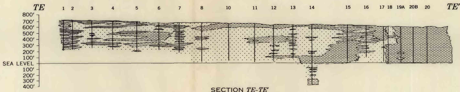
SECTION TE-TE'
