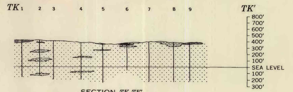
SECTION TK-TK'
