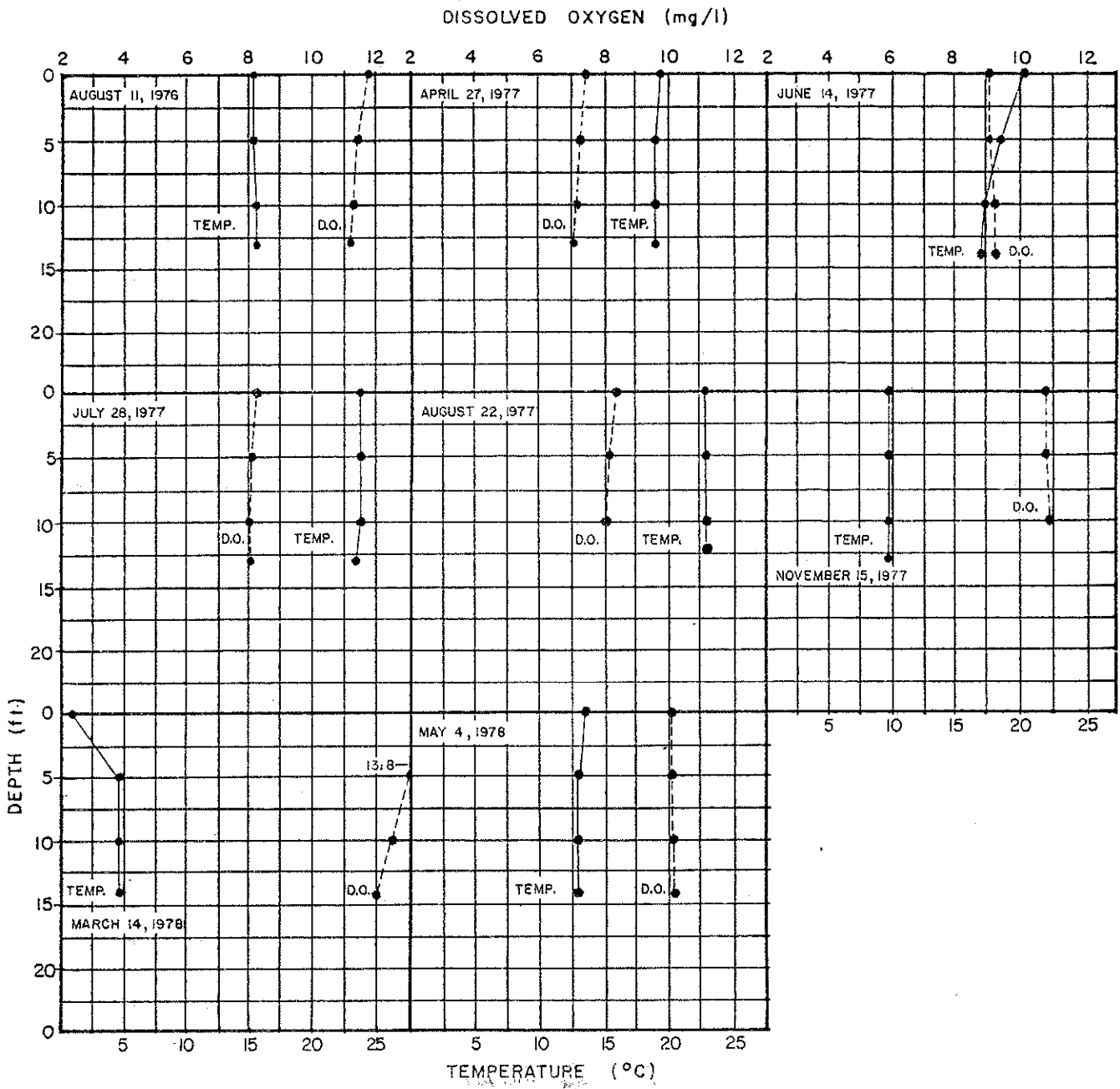
WHITE ISLAND POND TEMPERATURE (°C) and DISSOLVED OXYGEN DATA STATION 3
