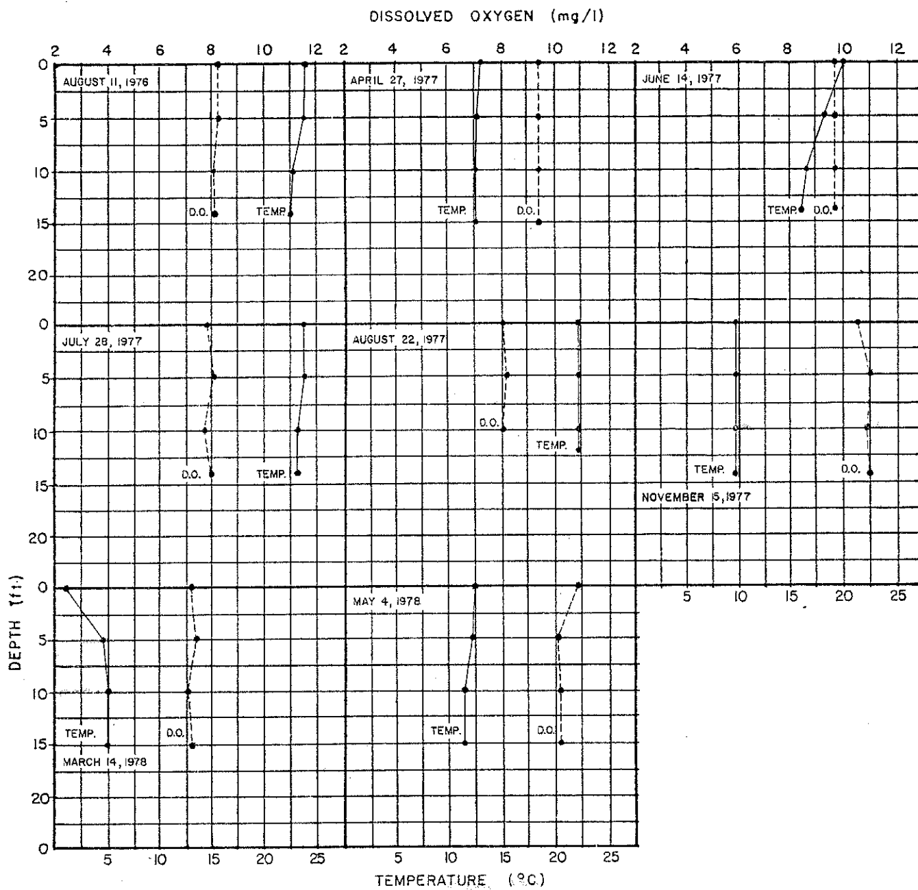
WHITE ISLAND POND TEMPERATURE (°C) and DISSOLVED OXYGEN DATA STATION I
