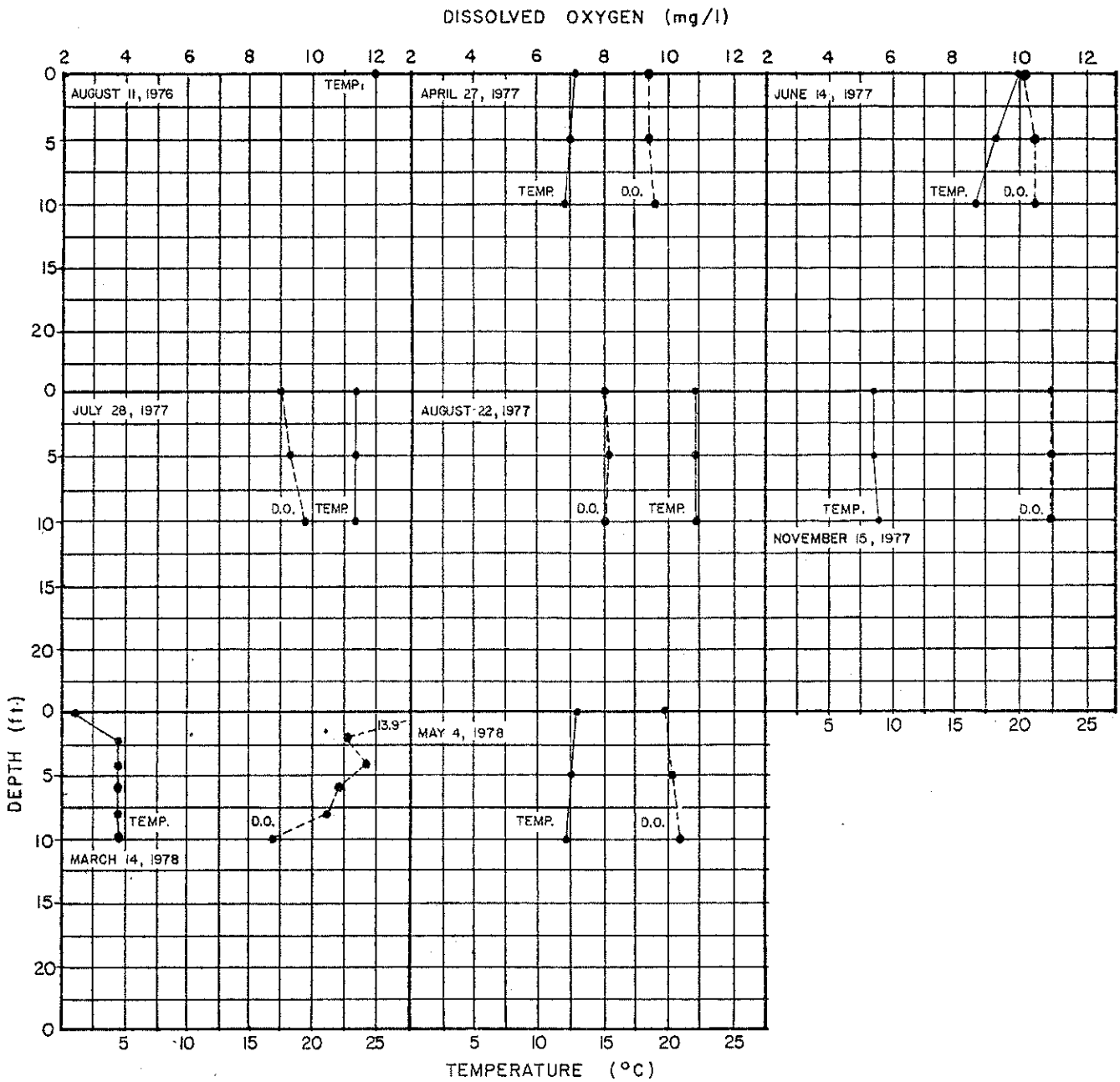
WHITE ISLAND POND TEMPERATURE (°C) and DISSOLVED OXYGEN DATA STATION 2
