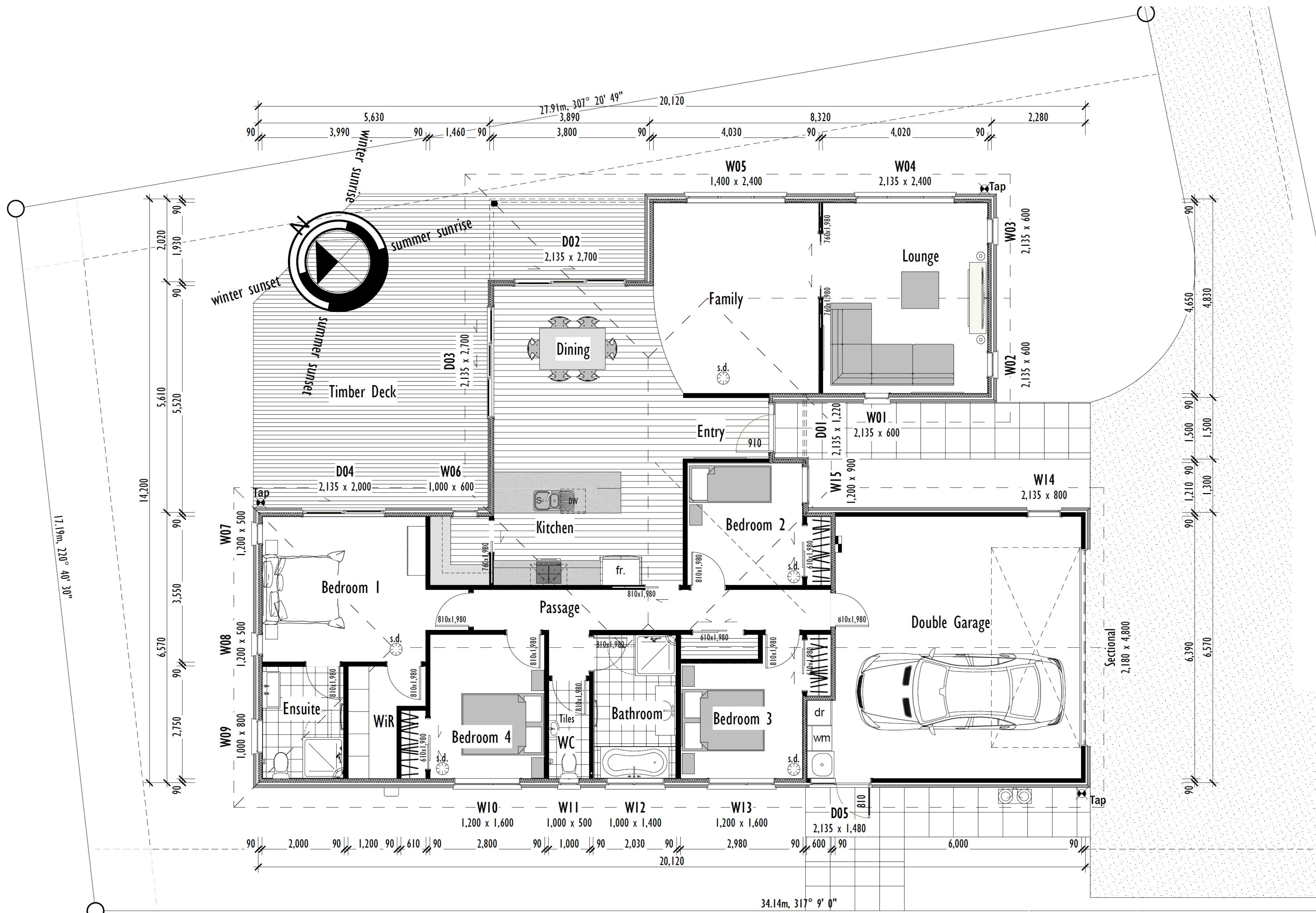
5 CLEAN FLOOR PLAN 1:100
