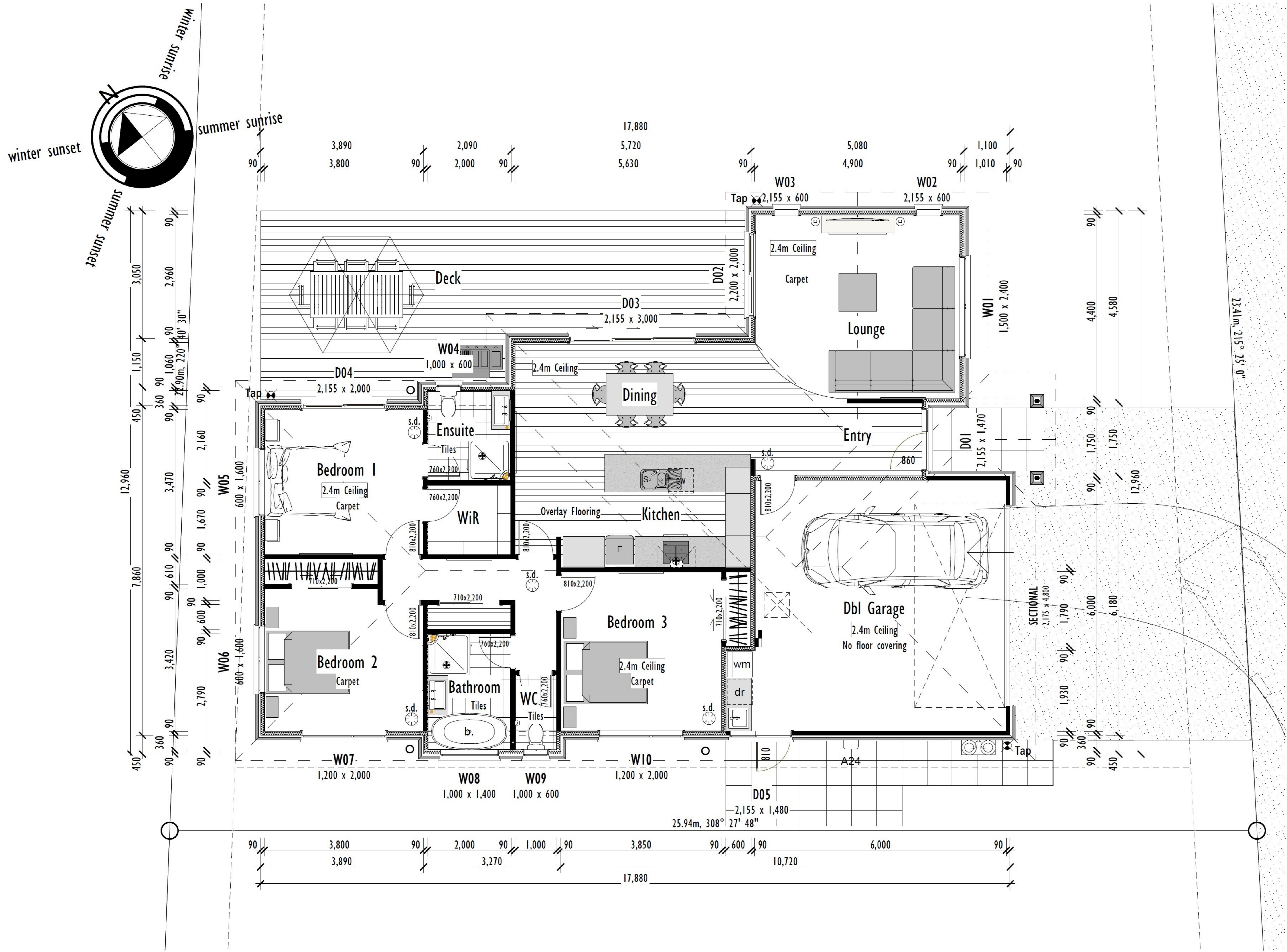
4 FLOOR PLAN CLEAN 1:100
