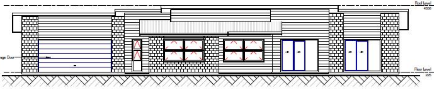
1 North Elevation 1 : 100
