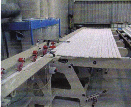
FE 6430 Lateral Infeed
