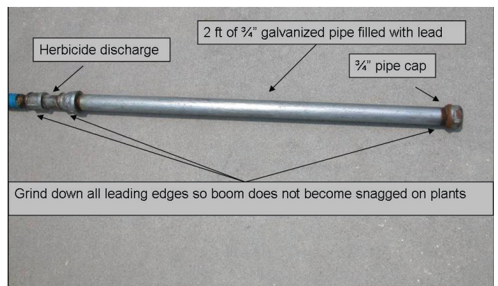
Figure 6. L lead-filled pipe at the end of the trailing hose. The depth of the lead-filled pipe will depend on the water depth and hose length and is greatly influenced by speed and weed density. Credits: Greg Reynolds.
