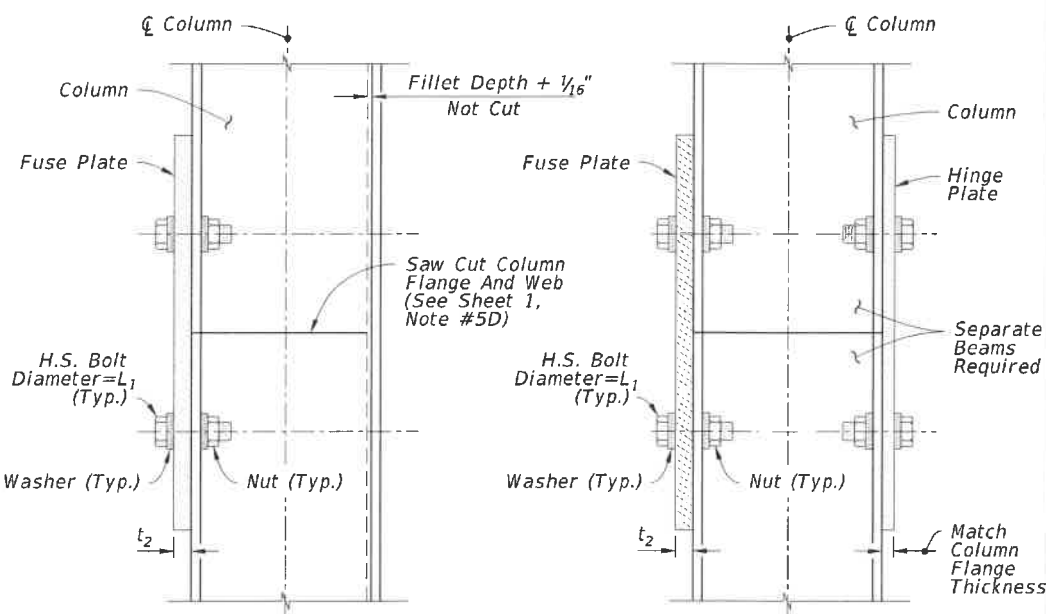
Side Elevation TYPICAL HINGE
