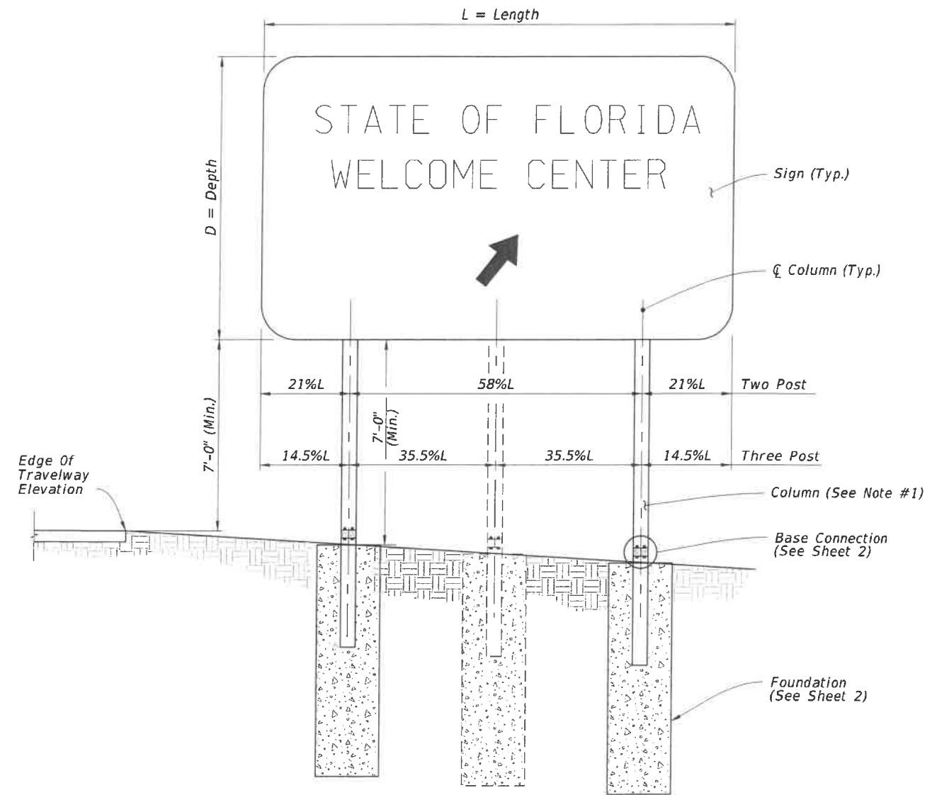
FRONT ELEVATION
