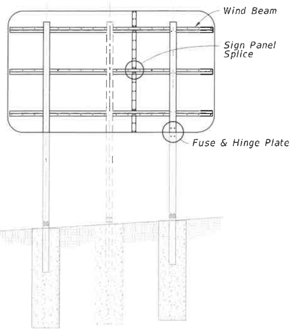
BACK ELEVATION
