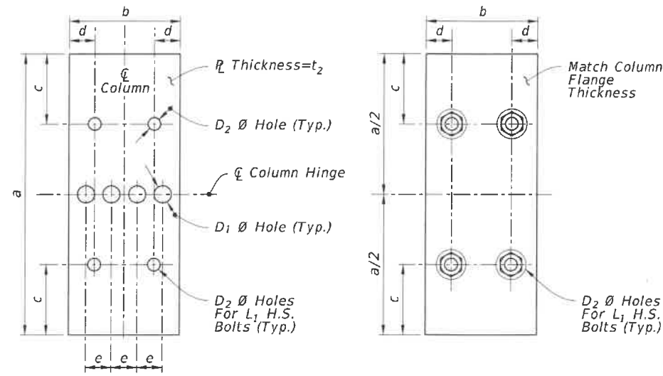
HINGE PLATE
