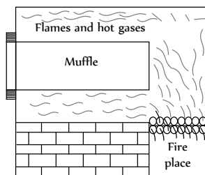
Fig. 16.7. Muffle furnace
