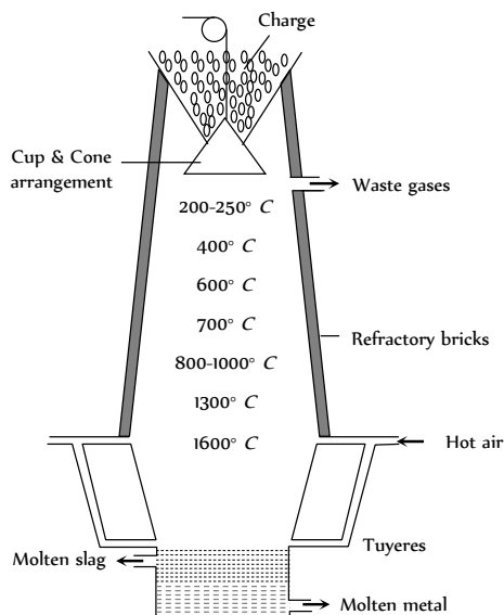
Fig. 16.5 Blast Furnace
