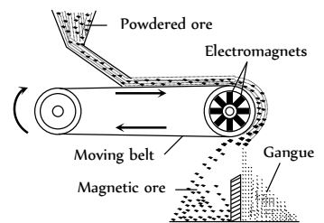
Fig. 16.3 Electromagnetic separation
