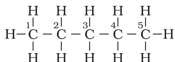
Pentane (n-pentane) (b.p. 309 K)
