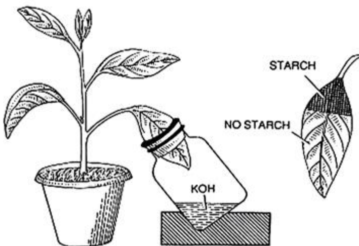
Fig 5.27. Mohl's experiment.
